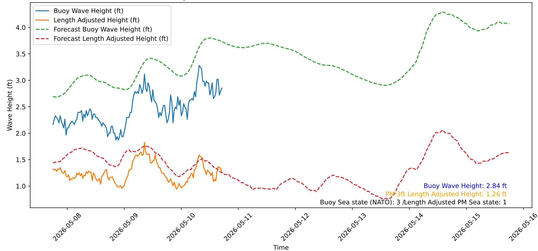
Wave Heights over Time for Oceanside Harbor at 2026-05-10 18:00:31
