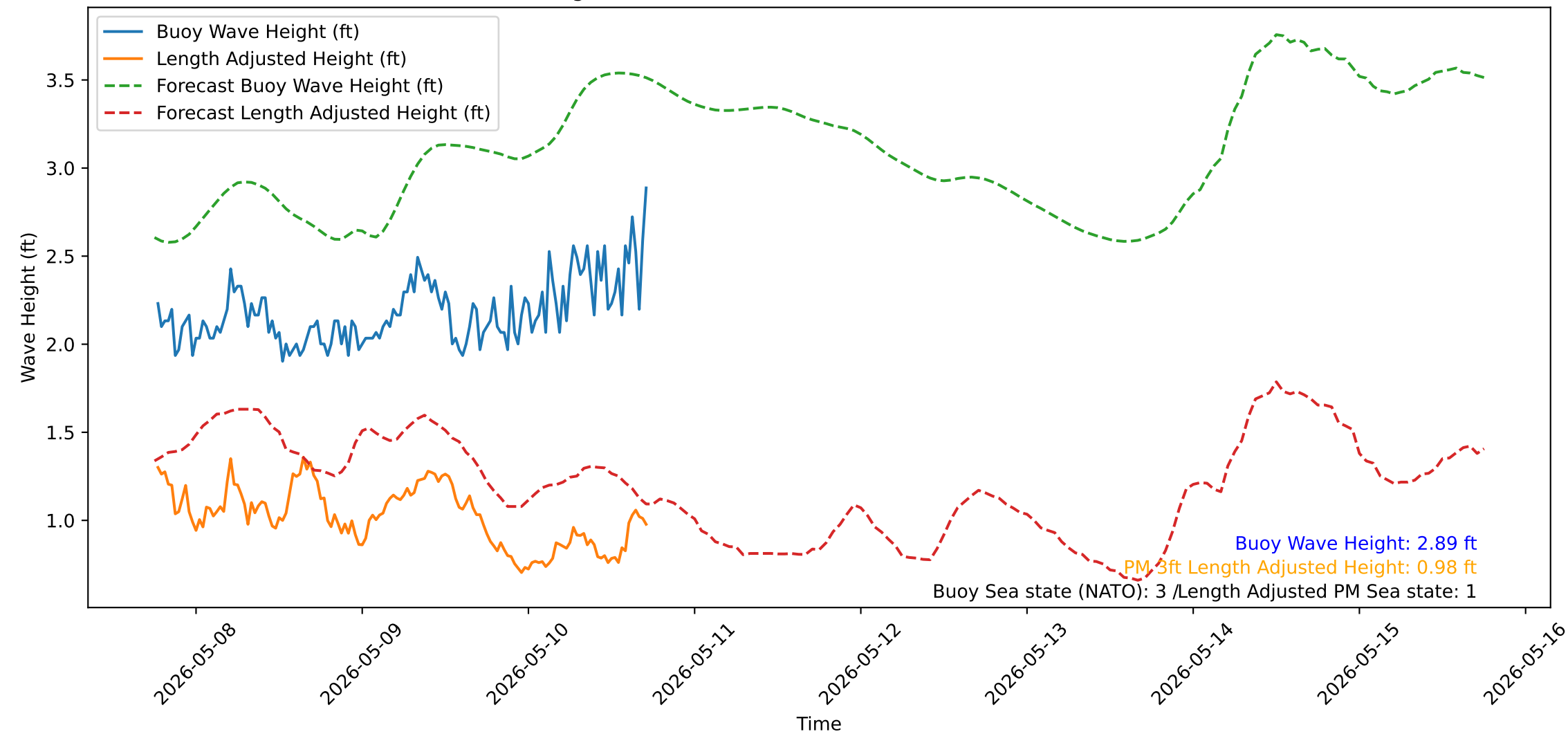
Wave Heights over Time for Red Beach at 2026-05-10 18:00:51
