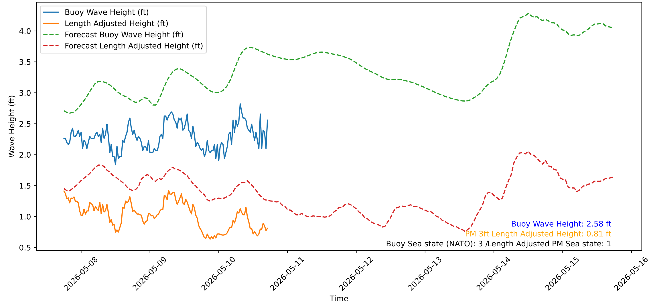
Wave Heights over Time for Green Beach at 2026-05-10 18:01:14
