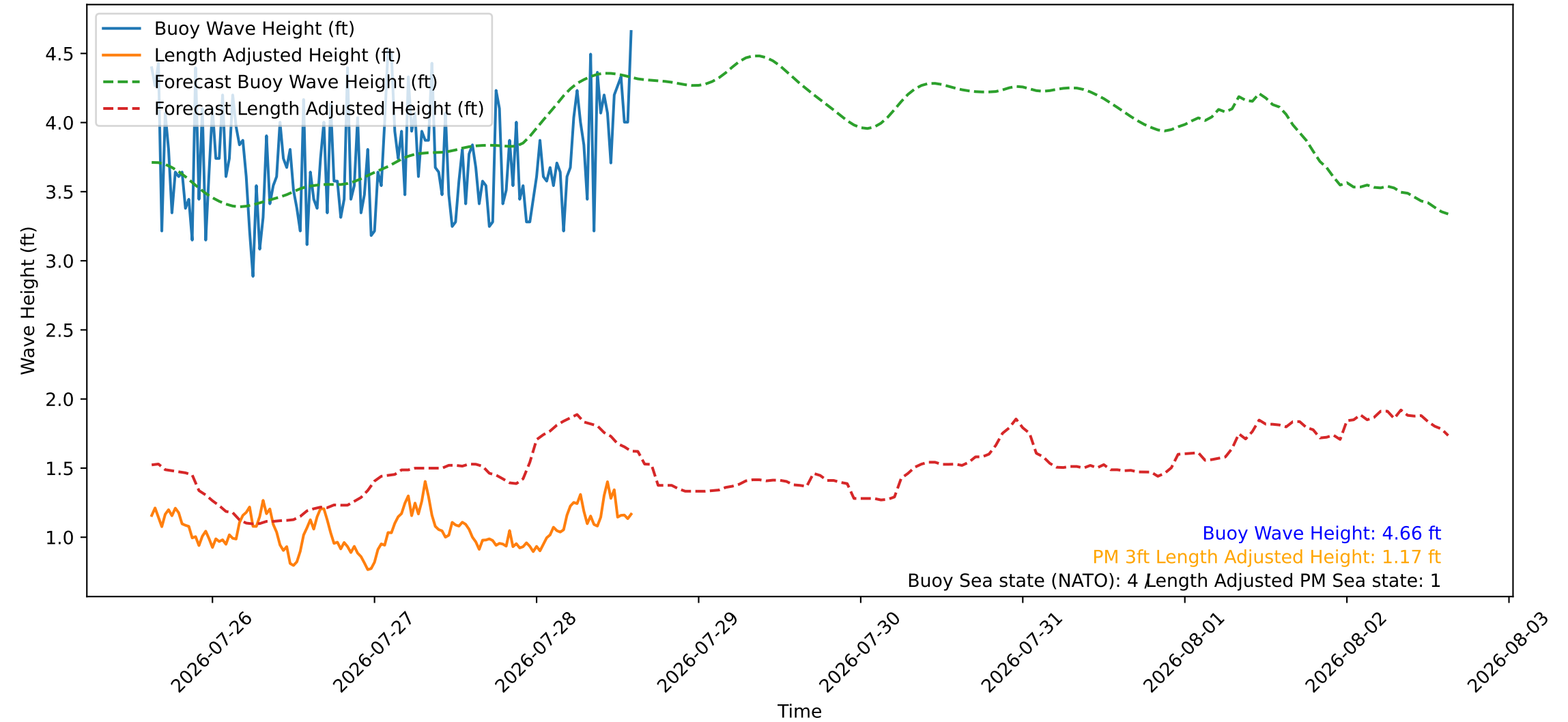
Wave Heights over Time for Red Beach at 2026-07-28 14:40:46
