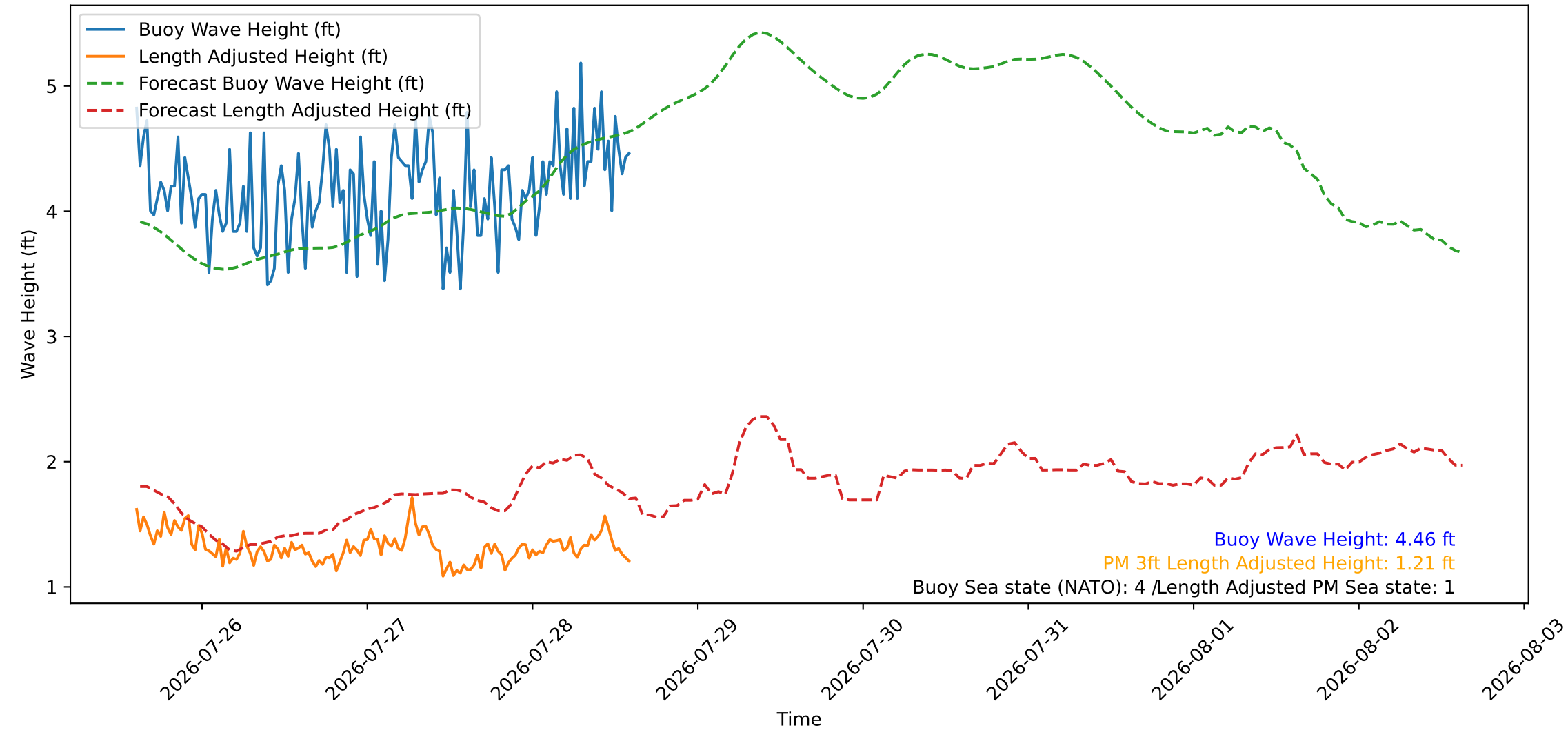
Wave Heights over Time for Green Beach at 2026-07-28 14:41:09
