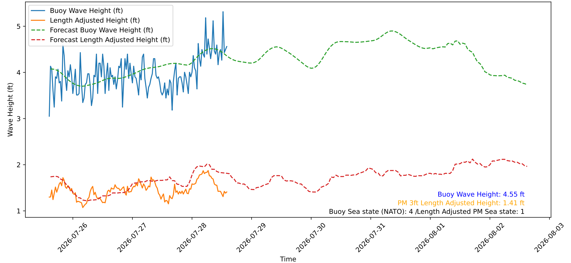
Wave Heights over Time for Oceanside Harbor at 2026-07-28 14:40:26
