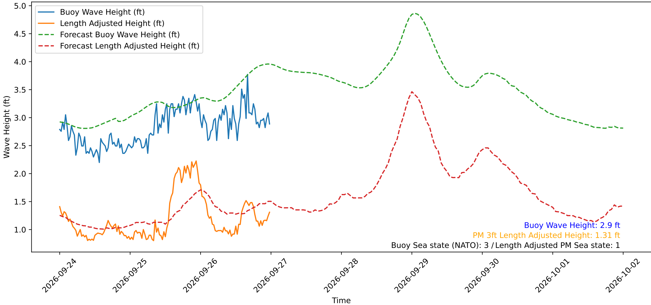
Wave Heights over Time for Oceanside Harbor at 2026-09-27 00:10:30
