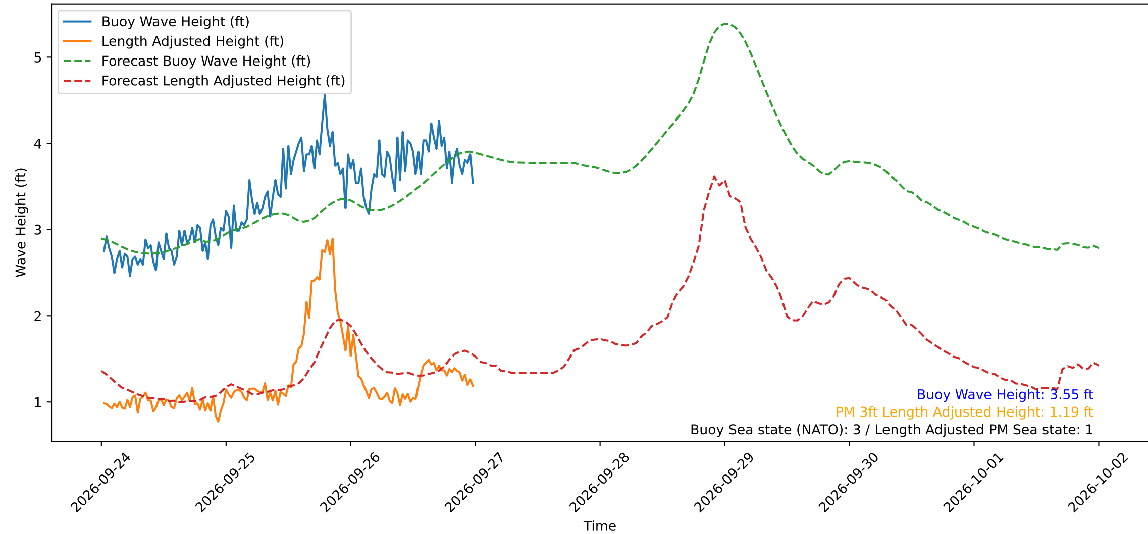
Wave Heights over Time for Green Beach at 2026-09-27 00:11:12
