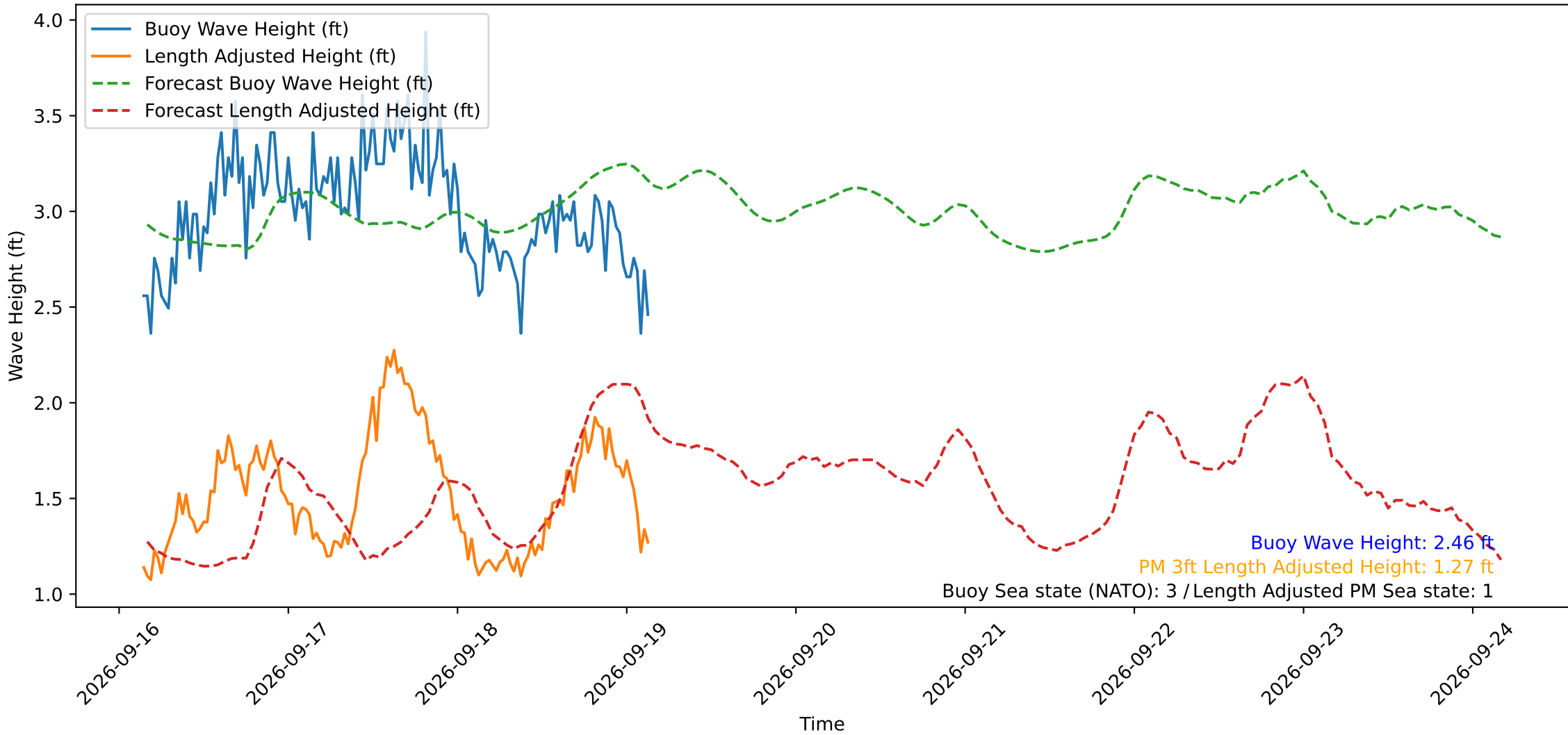
Wave Heights over Time for Oceanside Harbor at 2026-09-19 03:40:29
