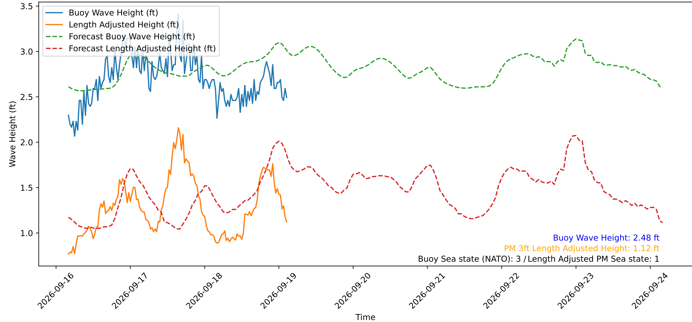
Wave Heights over Time for Red Beach at 2026-09-19 03:40:50
