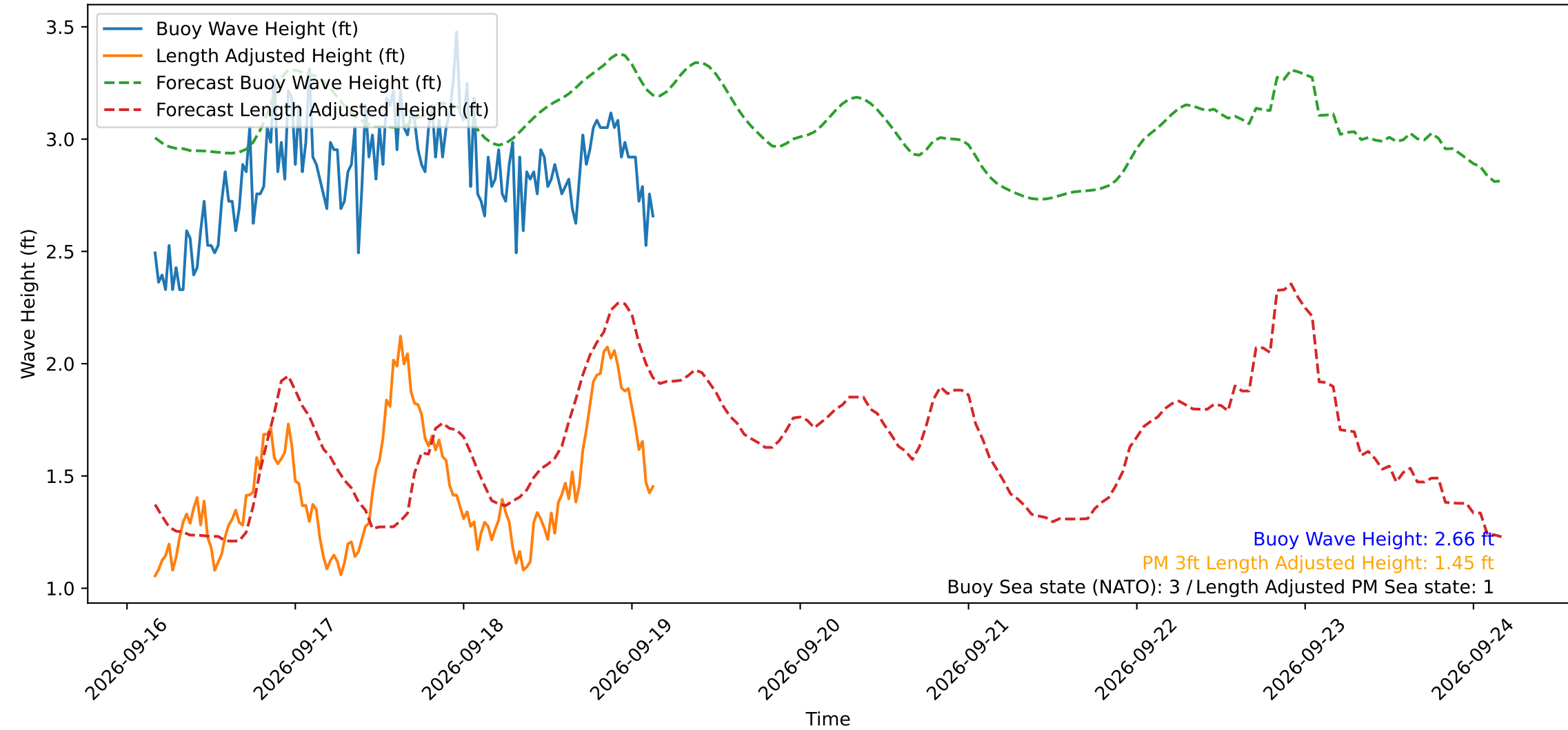
Wave Heights over Time for Green Beach at 2026-09-19 03:41:14
