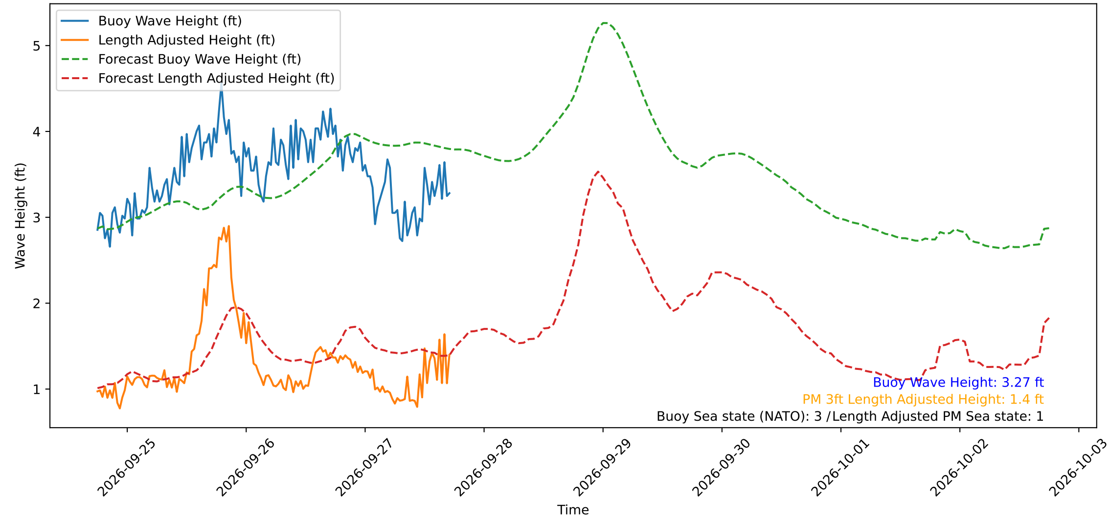
Wave Heights over Time for Green Beach at 2026-09-27 17:41:13
