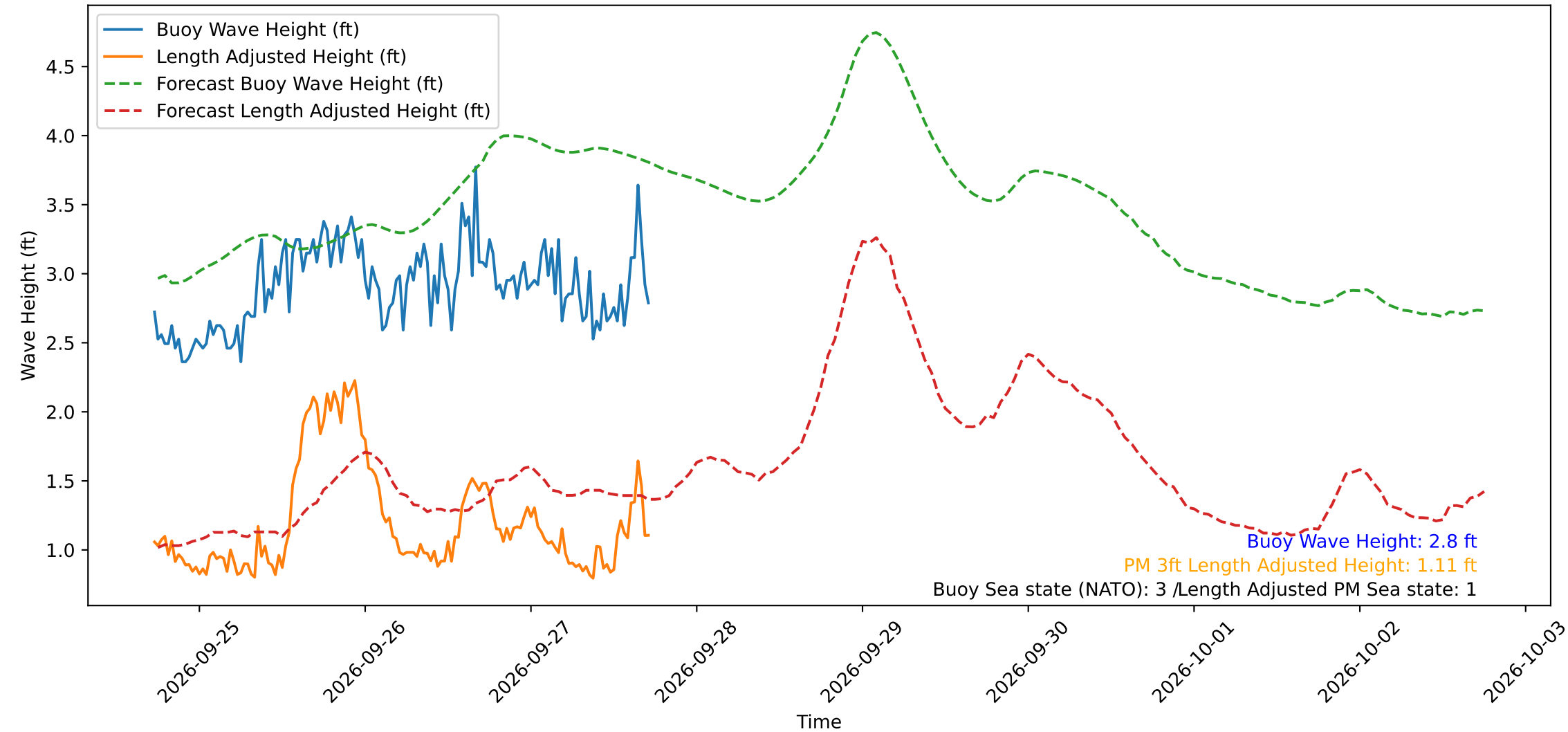
Wave Heights over Time for Oceanside Harbor at 2026-09-27 17:40:30
