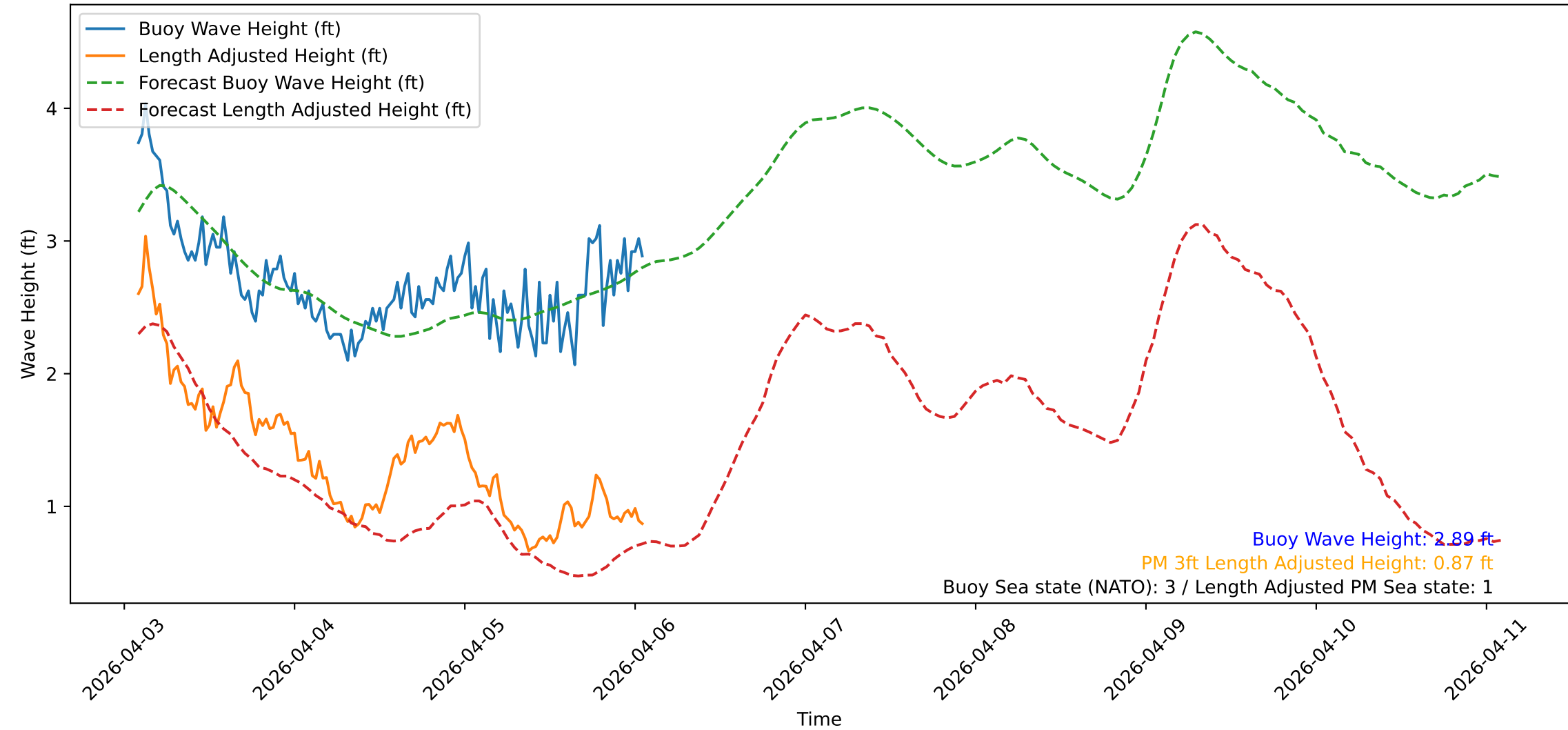
Wave Heights over Time for Oceanside Harbor at 2026-04-06 01:50:32
