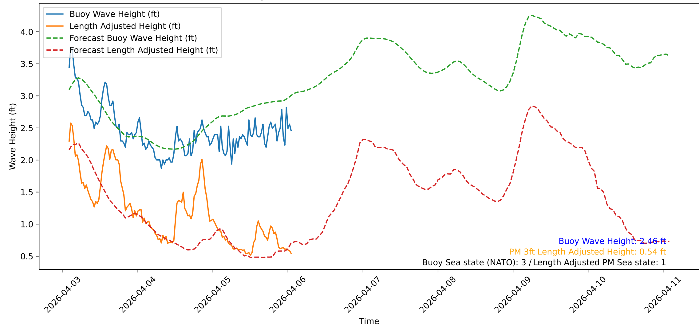
Wave Heights over Time for Red Beach at 2026-04-06 01:50:48
