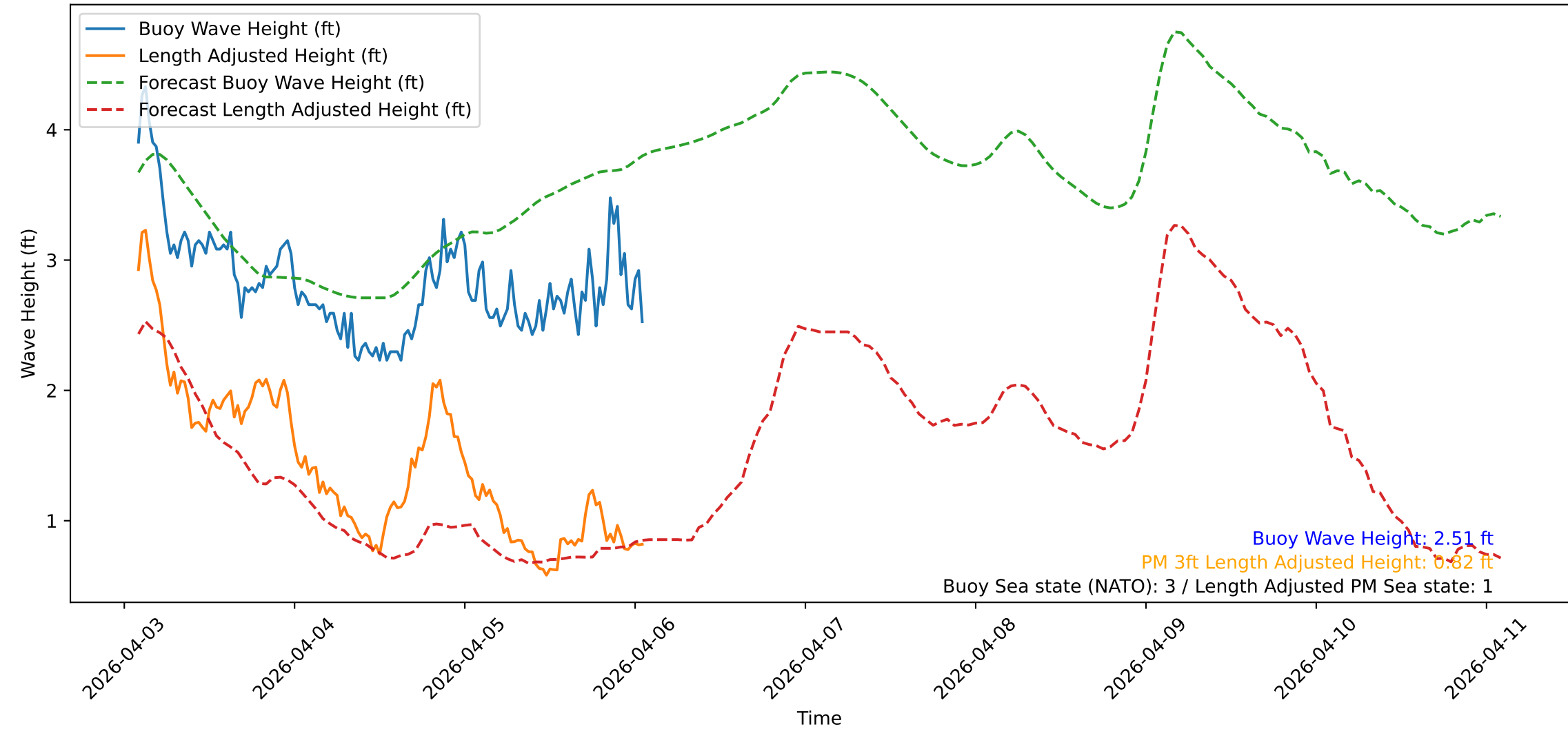
Wave Heights over Time for Green Beach at 2026-04-06 01:51:10
