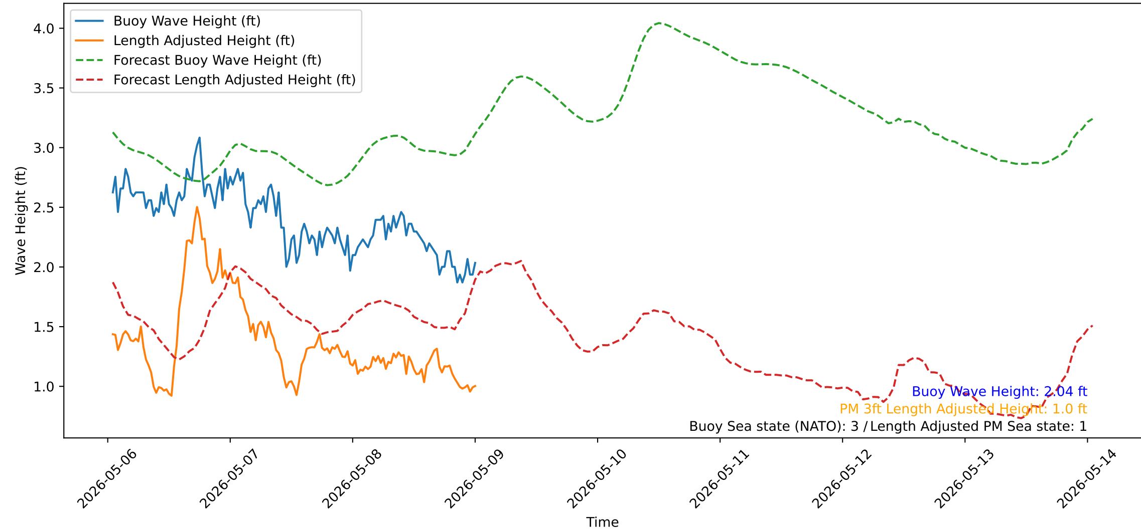
Wave Heights over Time for Oceanside Harbor at 2026-05-09 00:50:31
