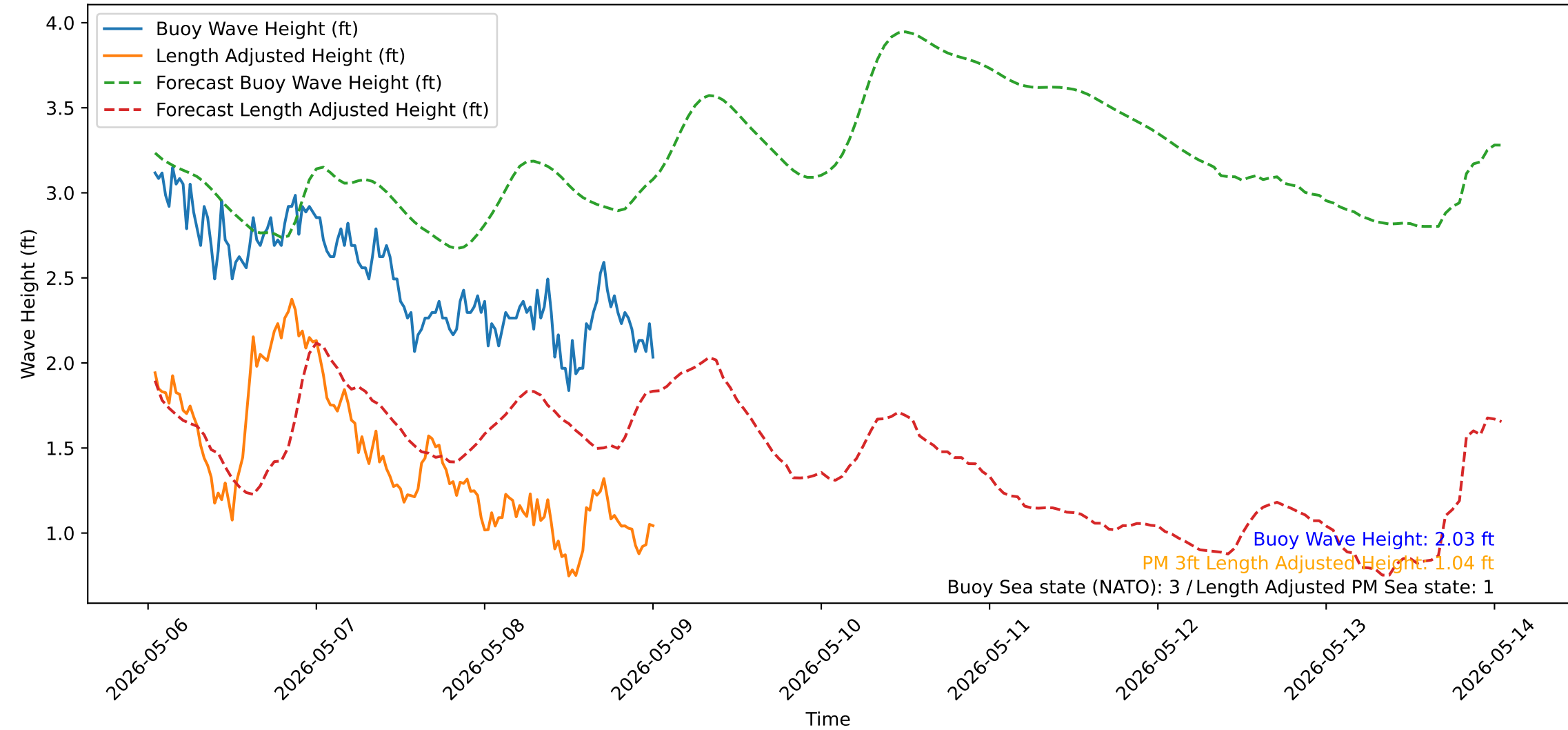
Wave Heights over Time for Green Beach at 2026-05-09 00:51:14
