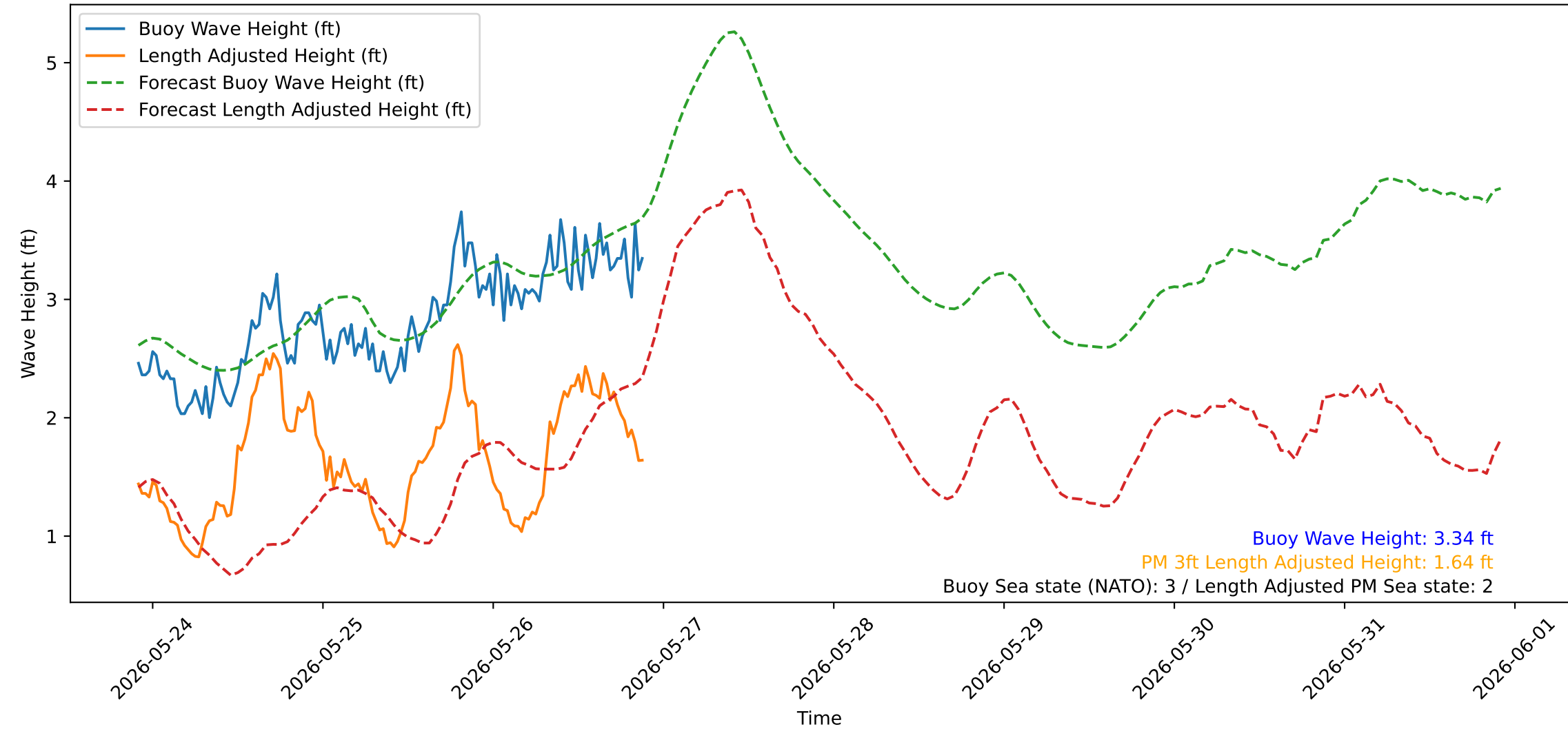
Wave Heights over Time for Red Beach at 2026-05-26 21:50:53
