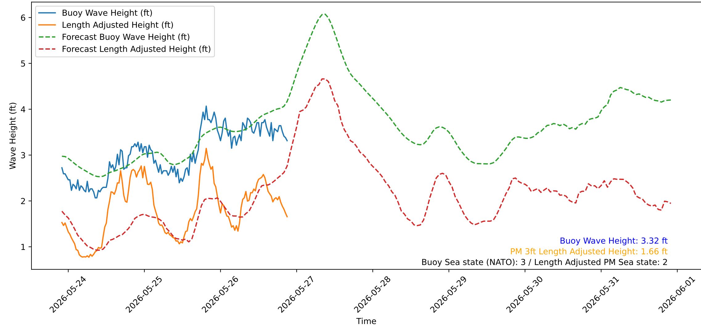
Wave Heights over Time for Green Beach at 2026-05-26 21:51:17
