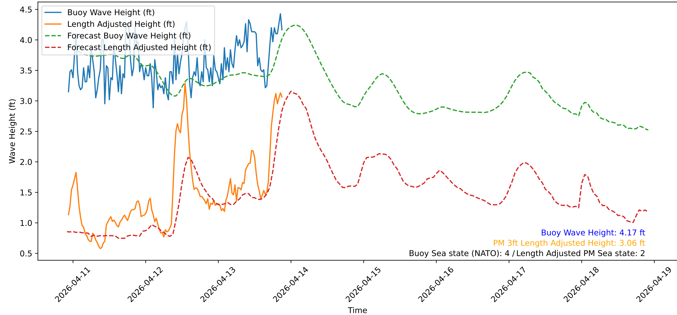
Wave Heights over Time for Red Beach at 2026-04-13 22:00:50
