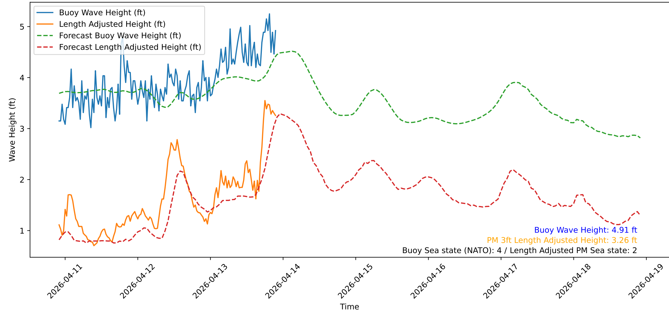
Wave Heights over Time for Oceanside Harbor at 2026-04-13 22:00:31
