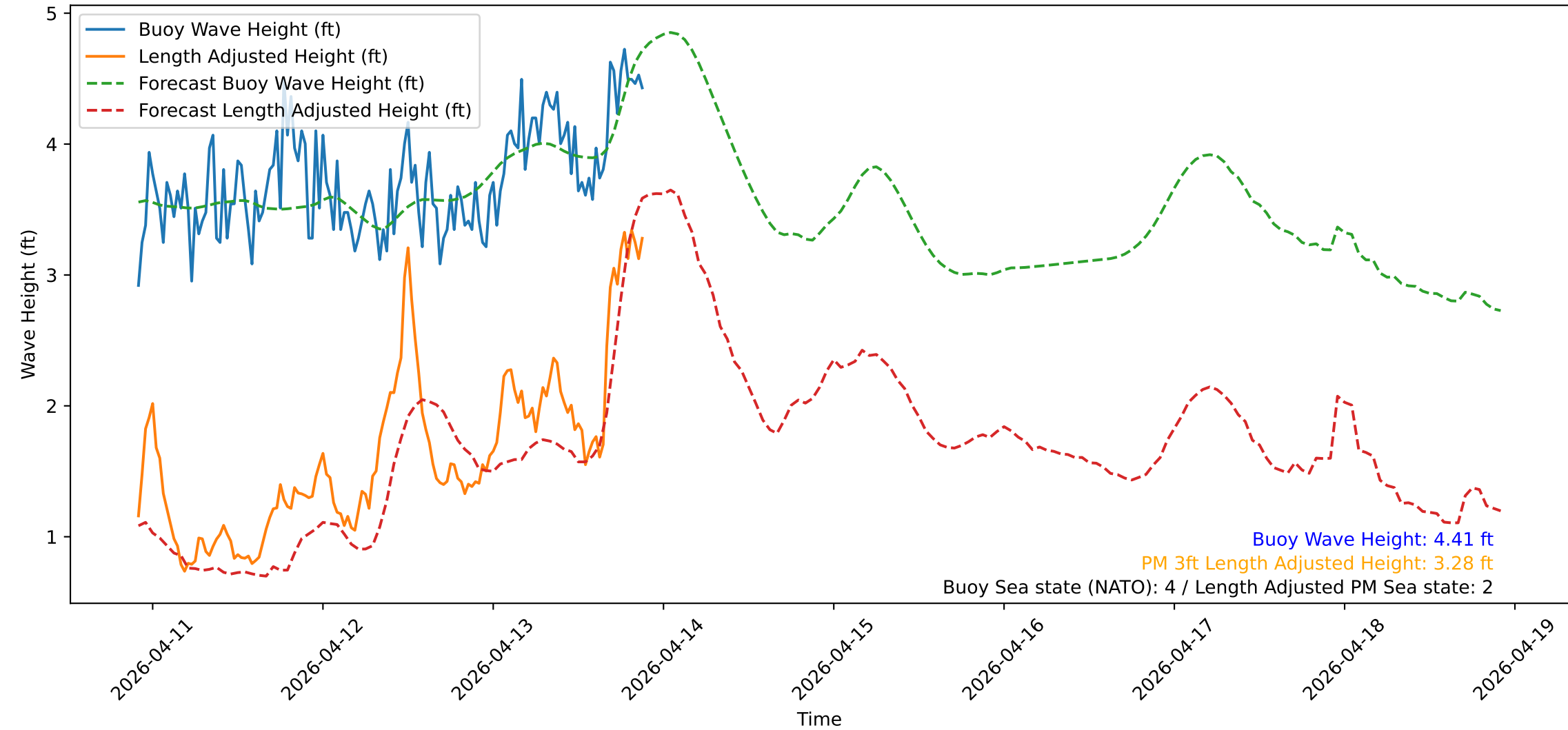
Wave Heights over Time for Green Beach at 2026-04-13 22:01:12
