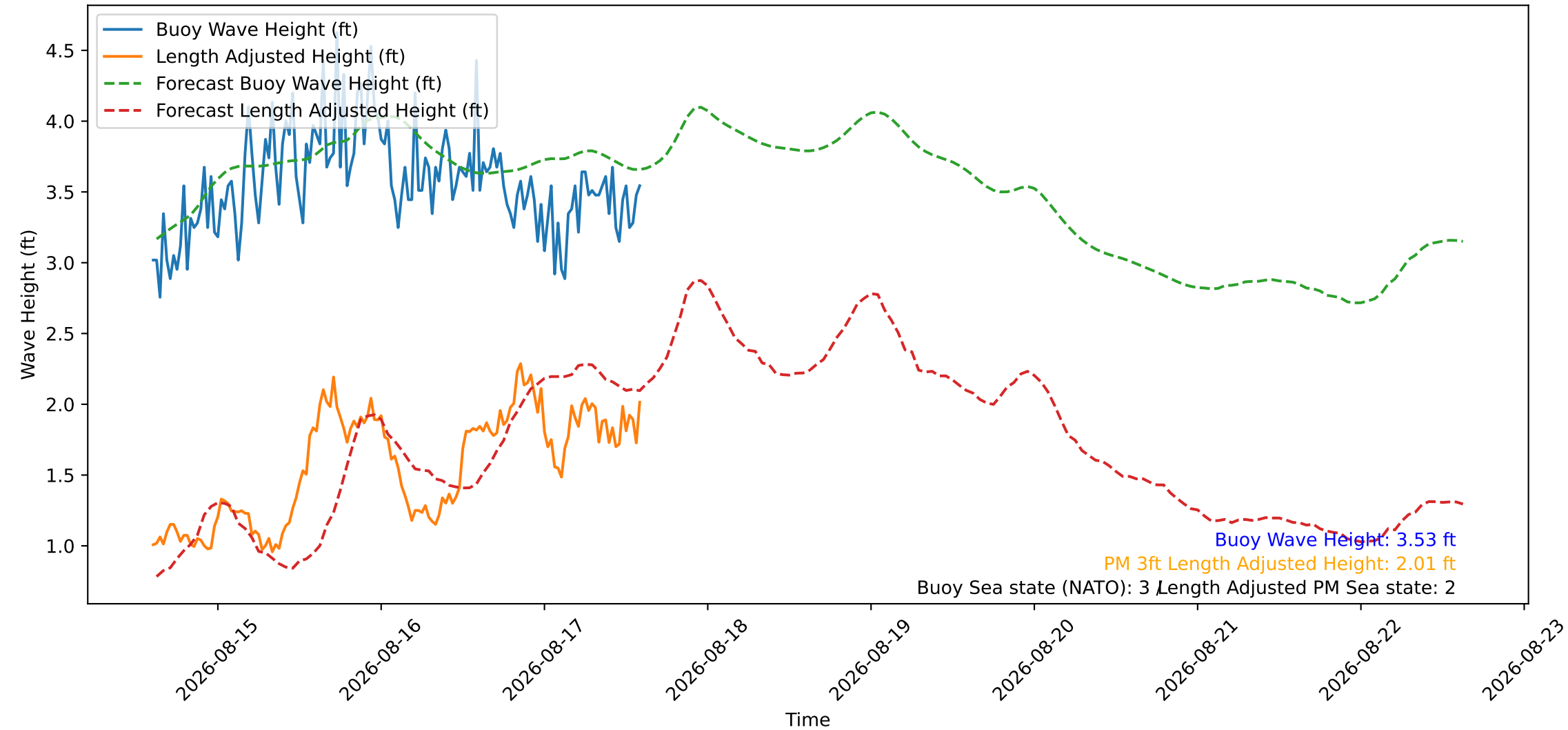
Wave Heights over Time for Oceanside Harbor at 2026-08-17 14:40:27
