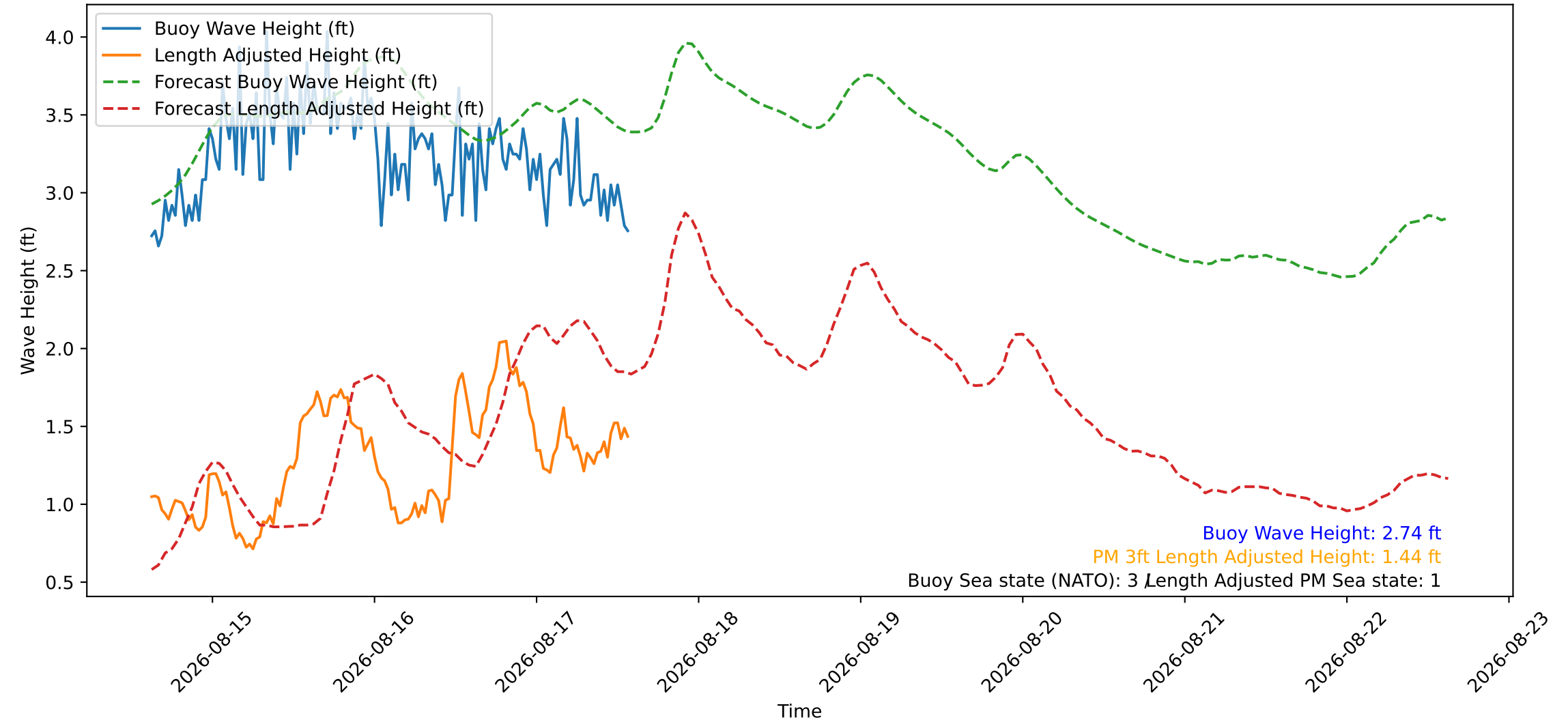
Wave Heights over Time for Red Beach at 2026-08-17 14:40:46
