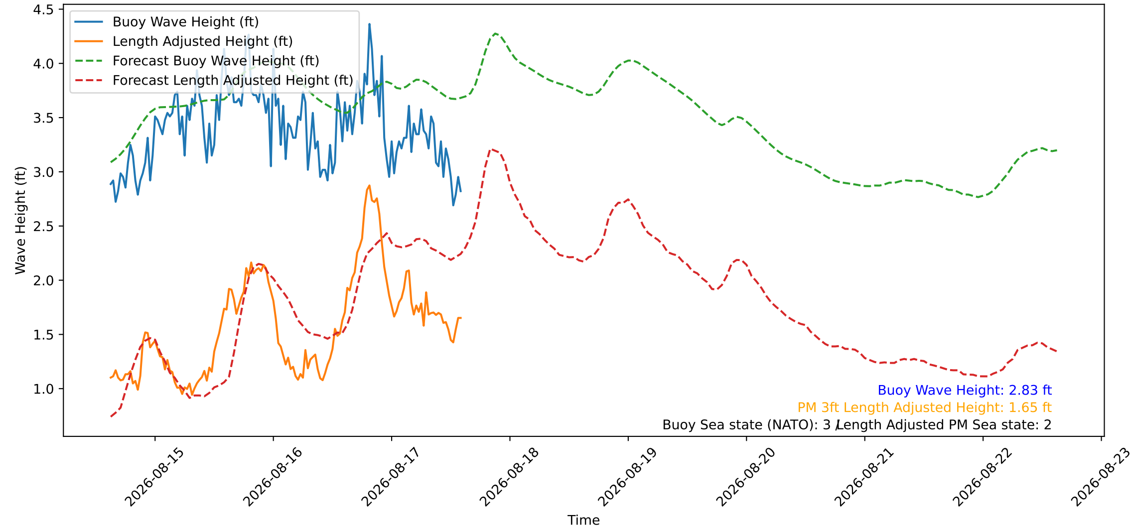
Wave Heights over Time for Green Beach at 2026-08-17 14:41:09
