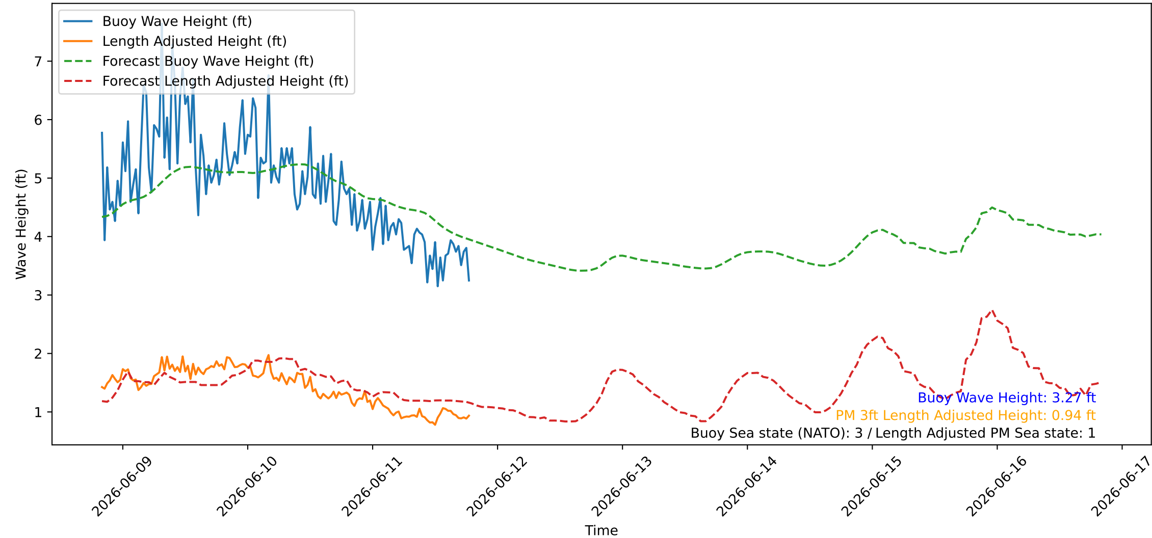
Wave Heights over Time for Red Beach at 2026-06-11 19:30:46
