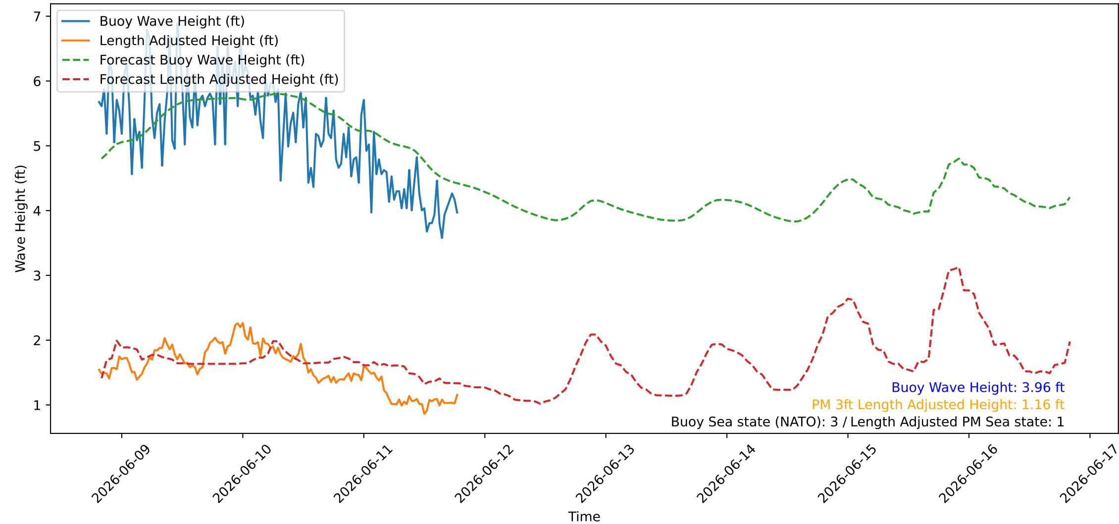
Wave Heights over Time for Green Beach at 2026-06-11 19:31:09
