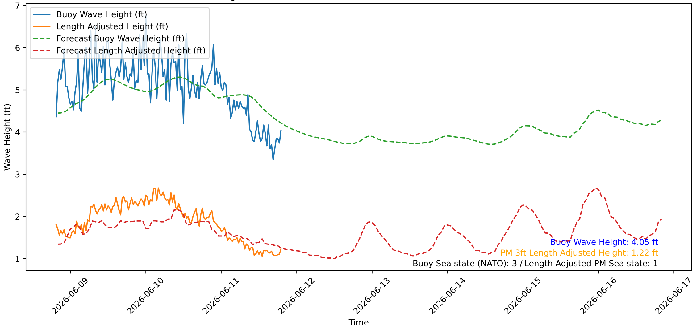
Wave Heights over Time for Oceanside Harbor at 2026-06-11 19:30:27
