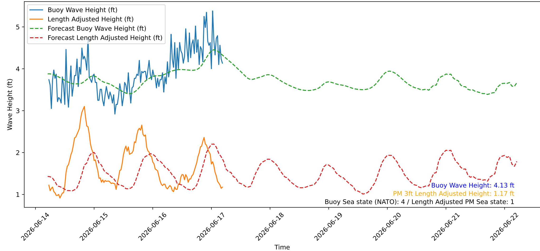
Wave Heights over Time for Red Beach at 2026-06-17 05:20:46
