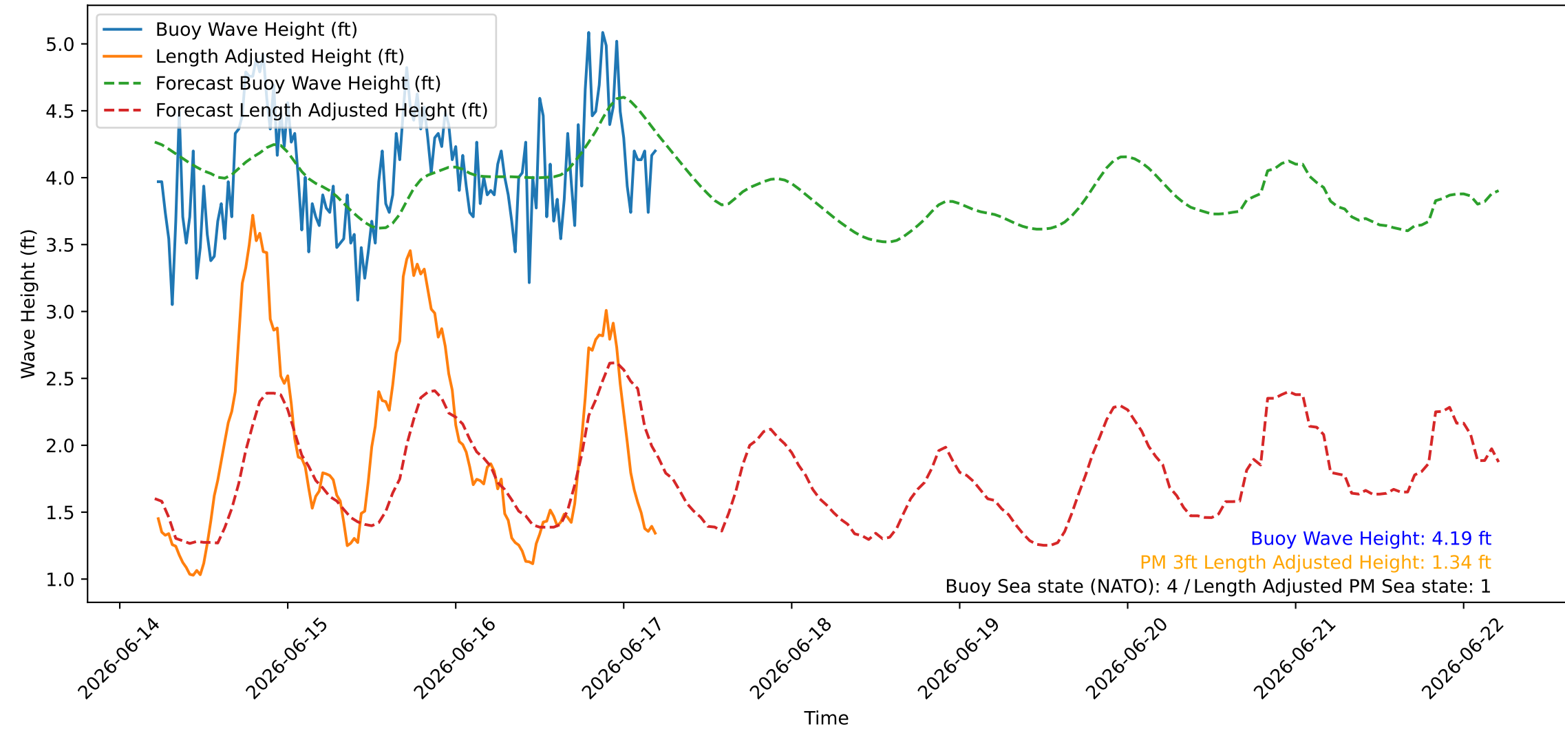
Wave Heights over Time for Green Beach at 2026-06-17 05:21:09
