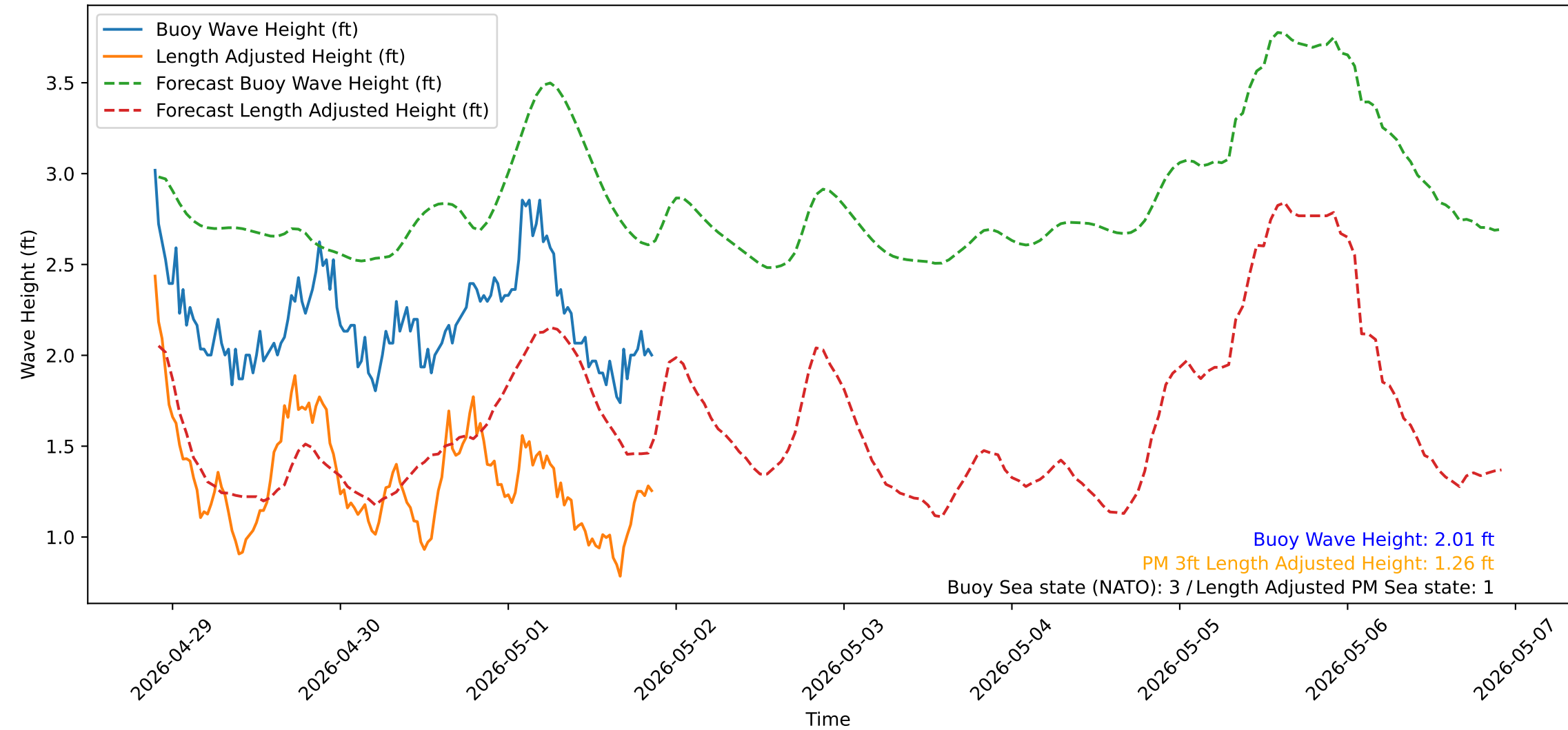
Wave Heights over Time for Green Beach at 2026-05-01 21:31:14
