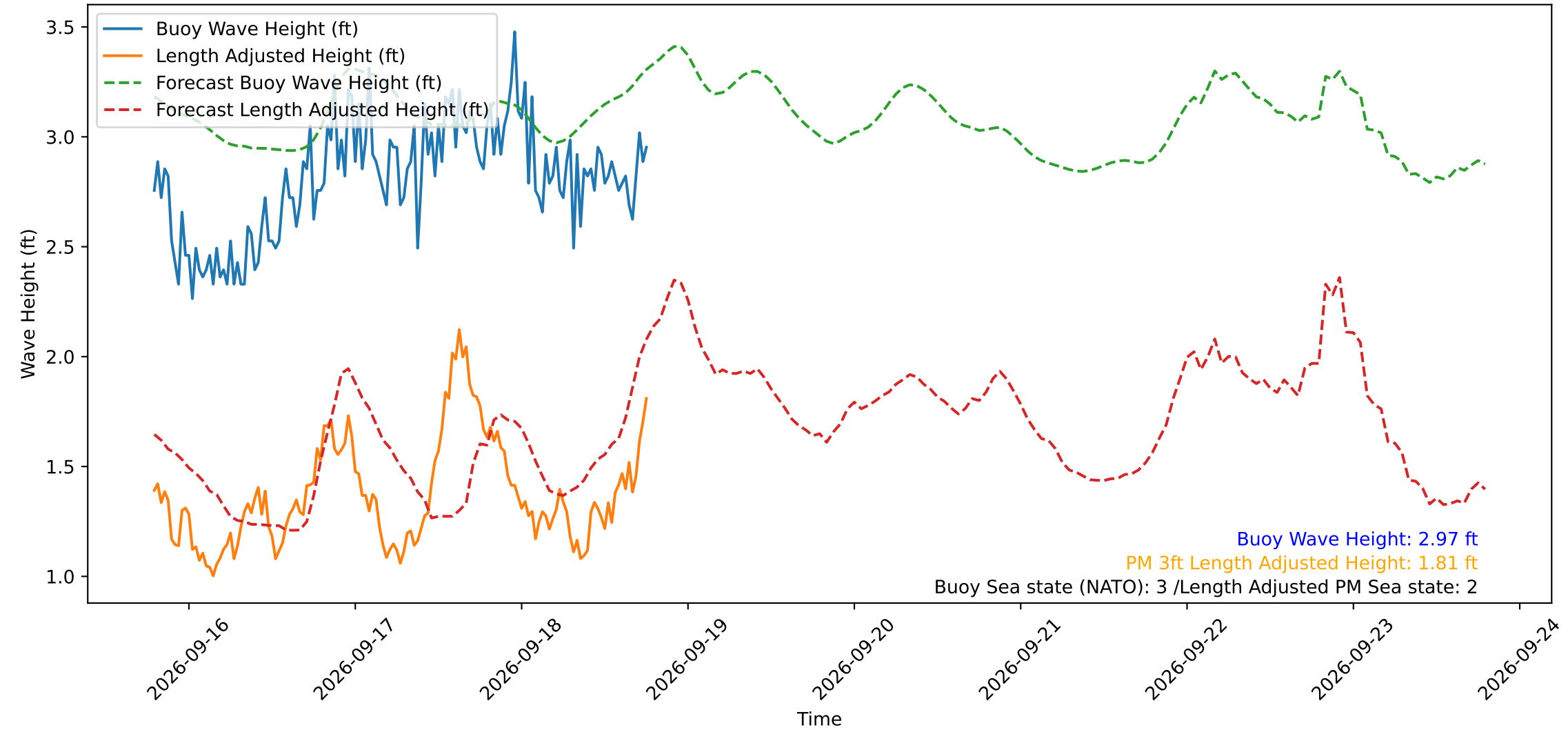
Wave Heights over Time for Green Beach at 2026-09-18 18:51:14
