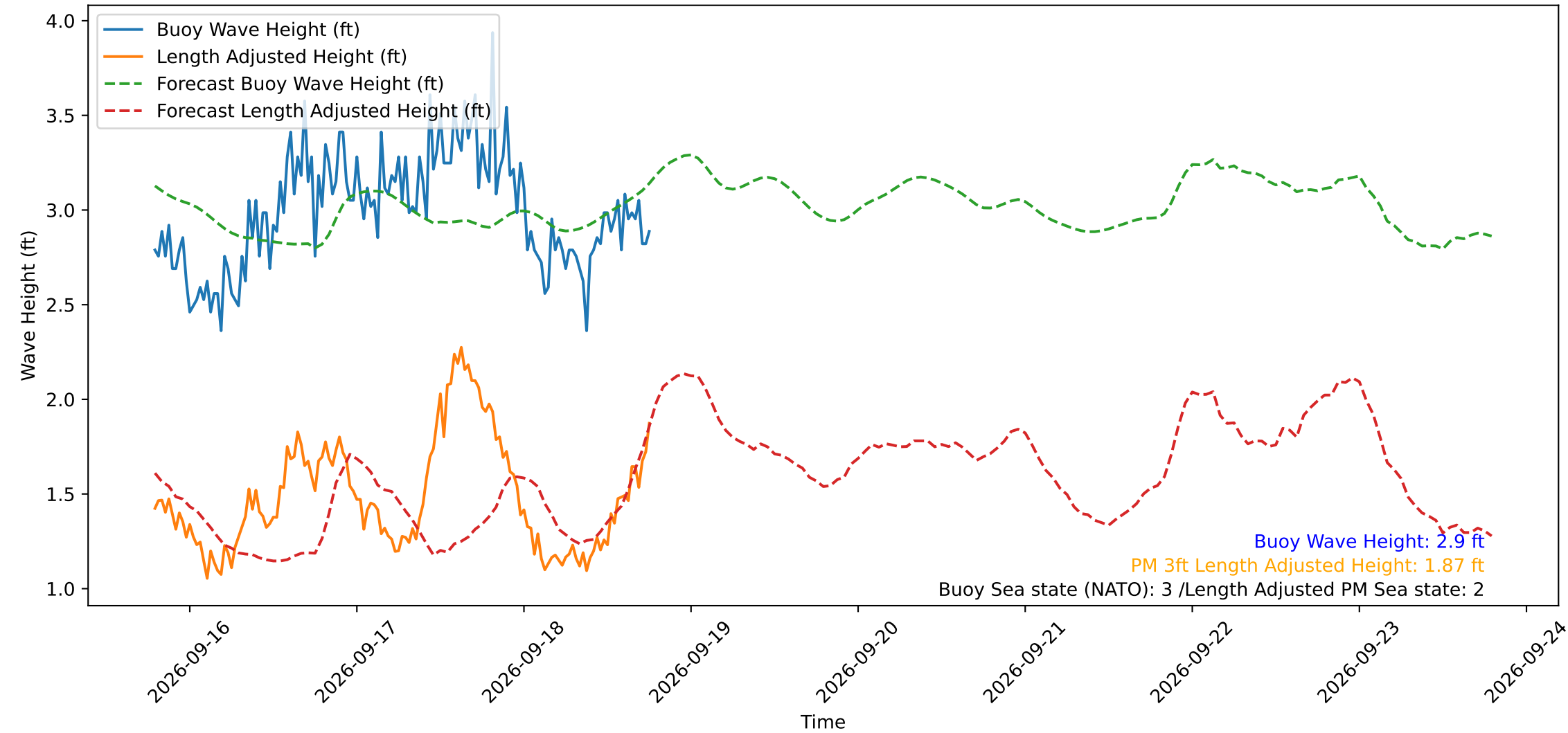
Wave Heights over Time for Oceanside Harbor at 2026-09-18 18:50:29
