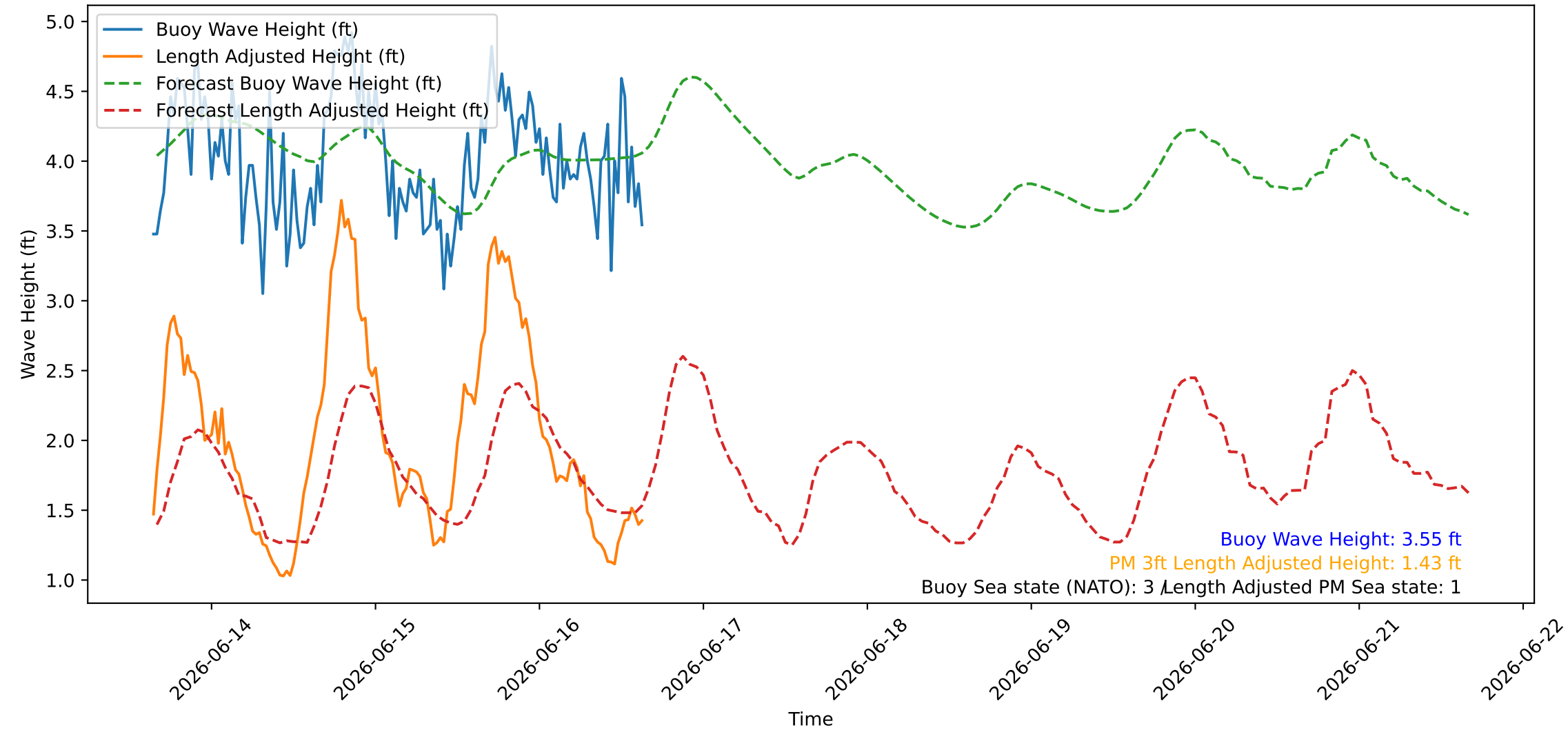
Wave Heights over Time for Green Beach at 2026-06-16 15:41:08
