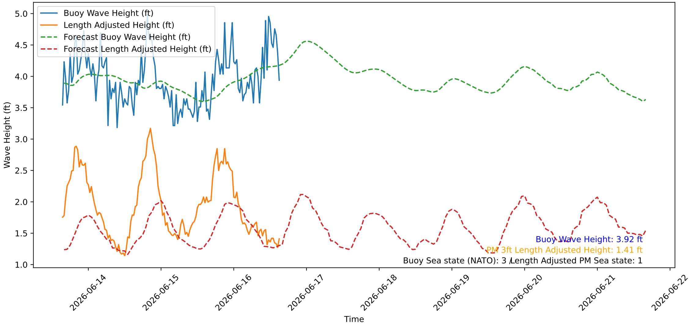
Wave Heights over Time for Oceanside Harbor at 2026-06-16 15:40:26
