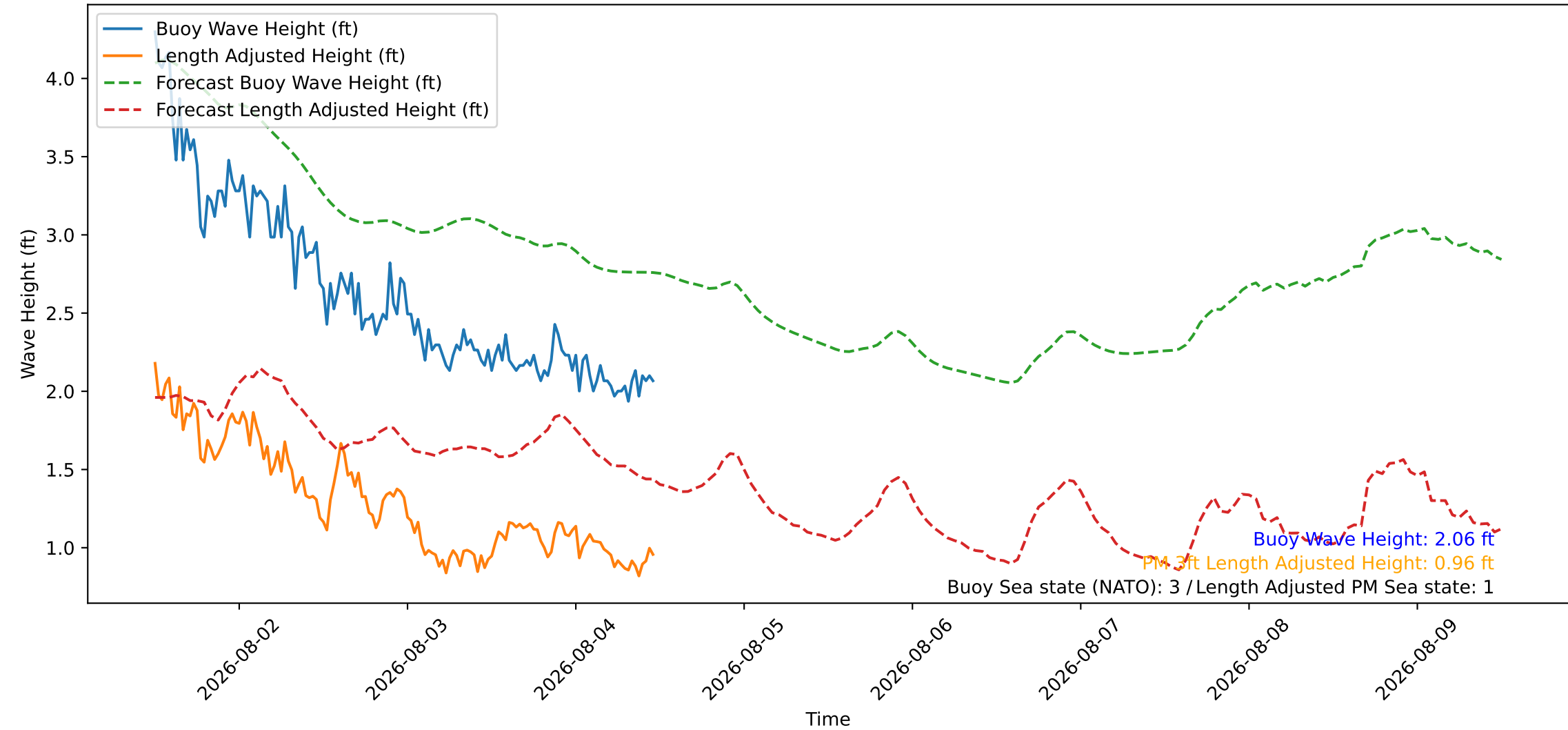
Wave Heights over Time for Green Beach at 2026-08-04 12:01:08
