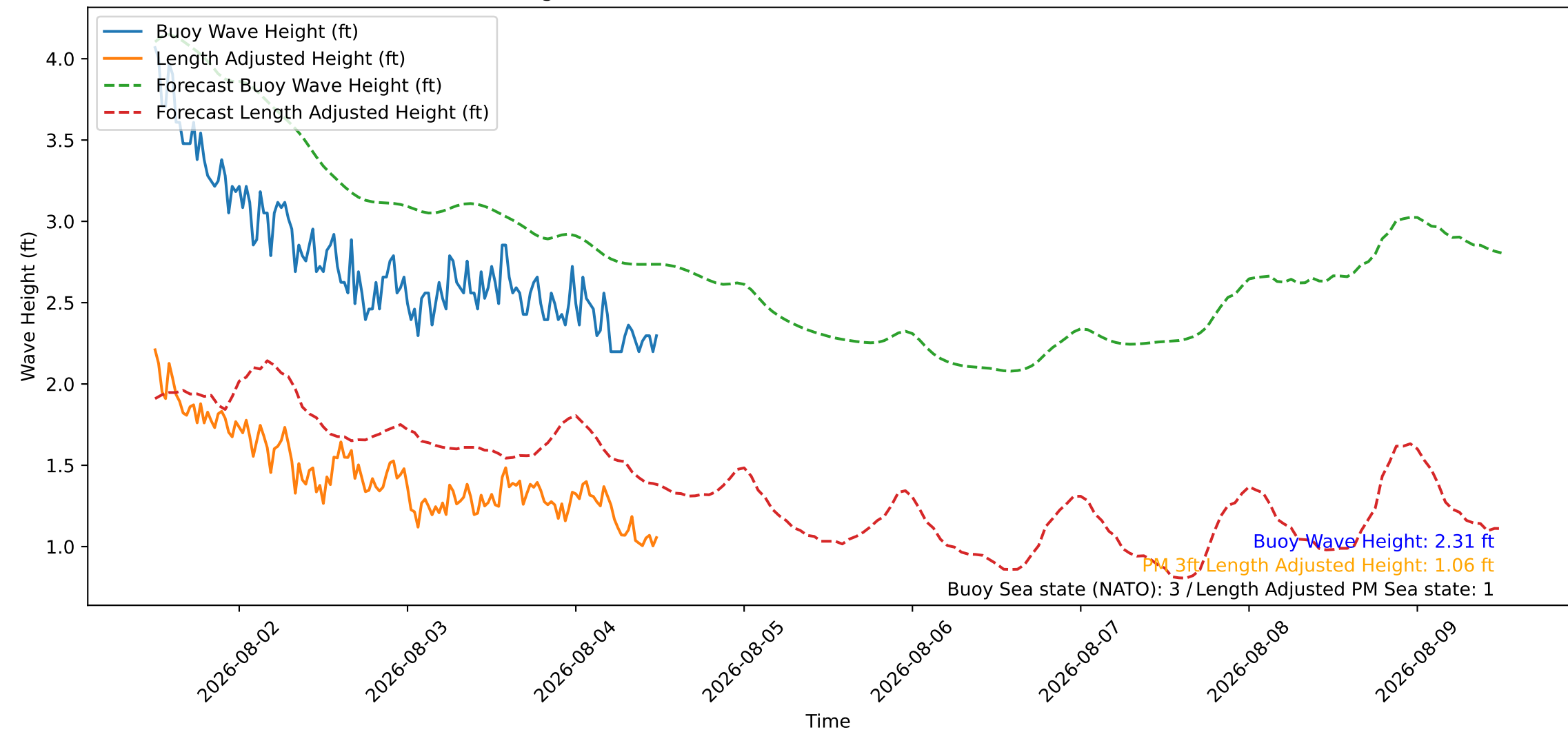
Wave Heights over Time for Oceanside Harbor at 2026-08-04 12:00:27
