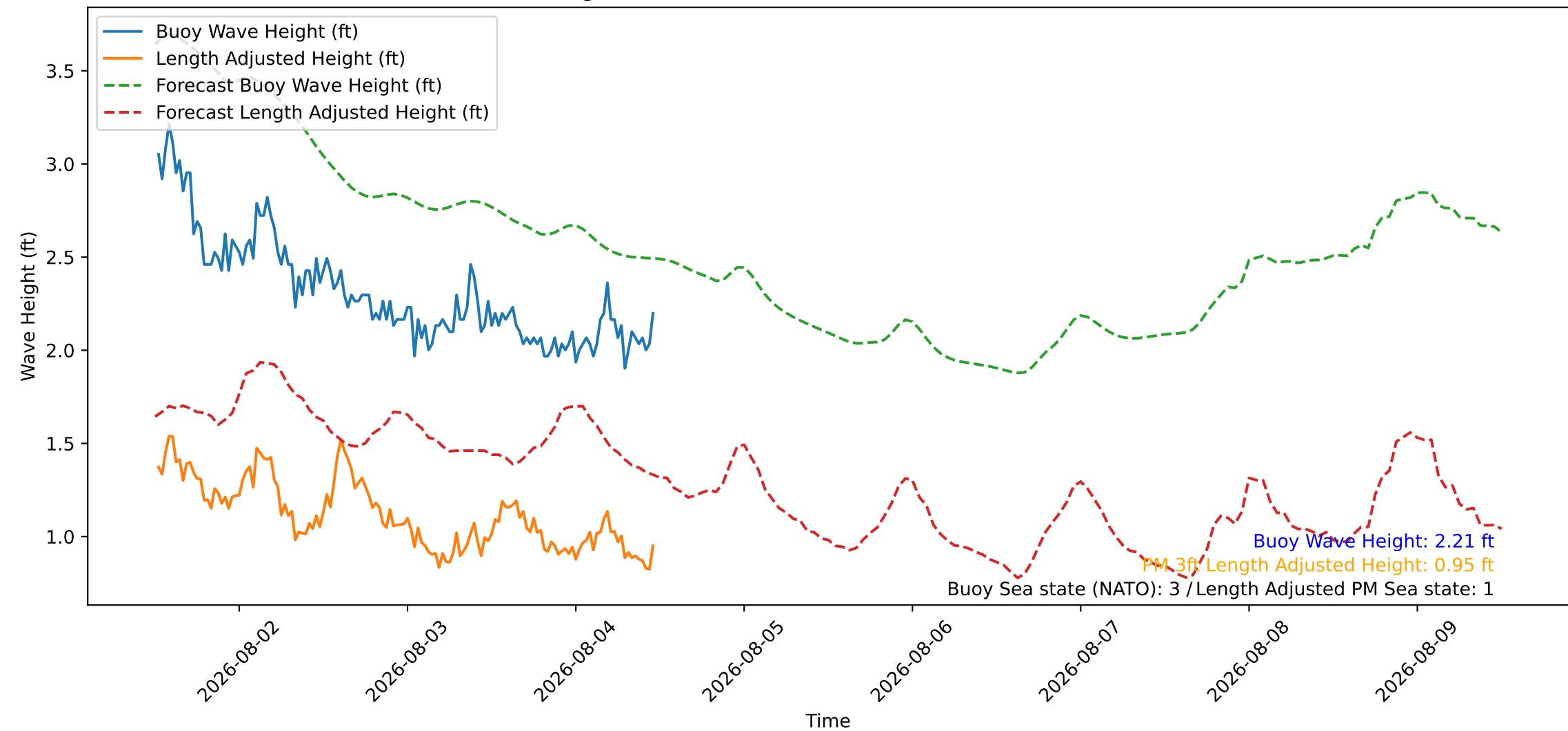
Wave Heights over Time for Red Beach at 2026-08-04 12:00:46
