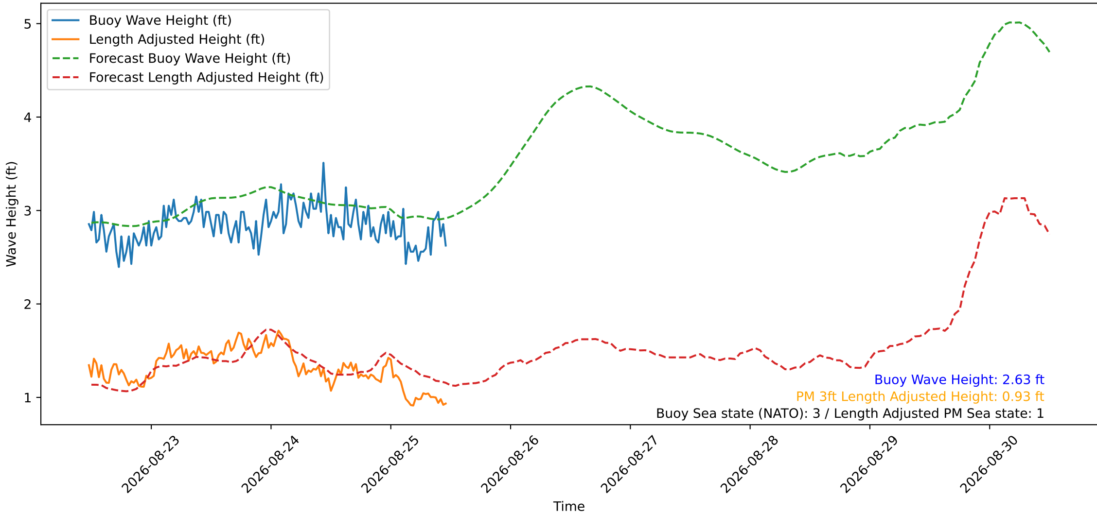
Wave Heights over Time for Oceanside Harbor at 2026-08-25 11:40:29
