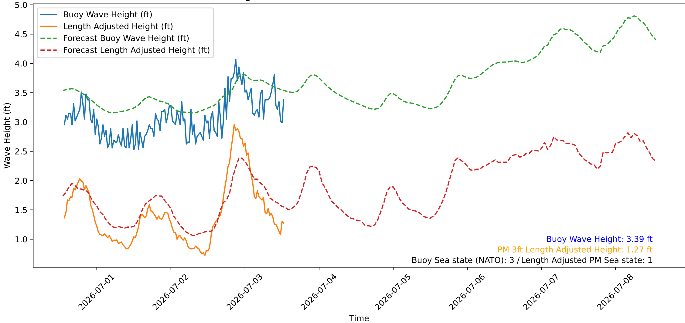
Wave Heights over Time for Green Beach at 2026-07-03 13:21:09
