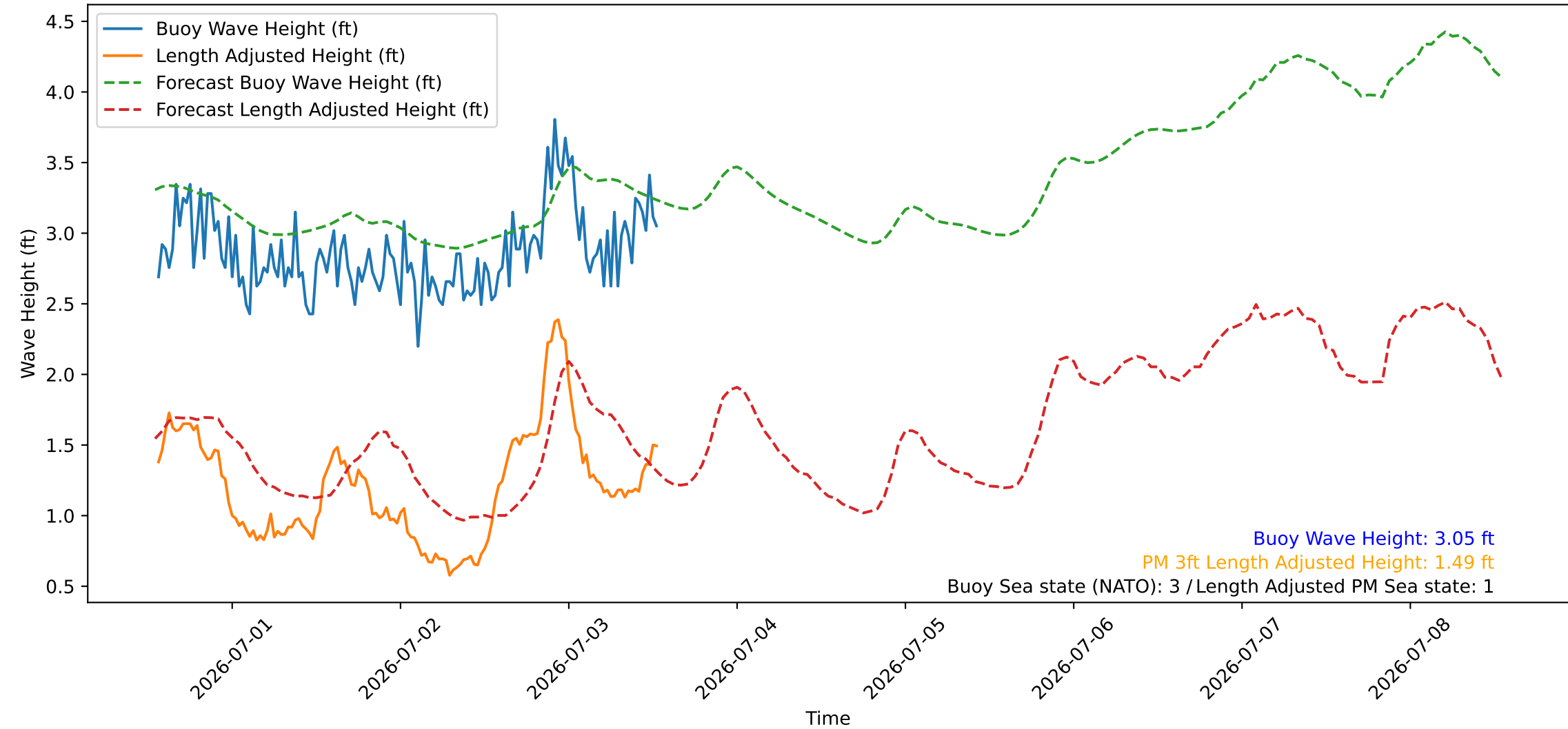
Wave Heights over Time for Red Beach at 2026-07-03 13:20:47
