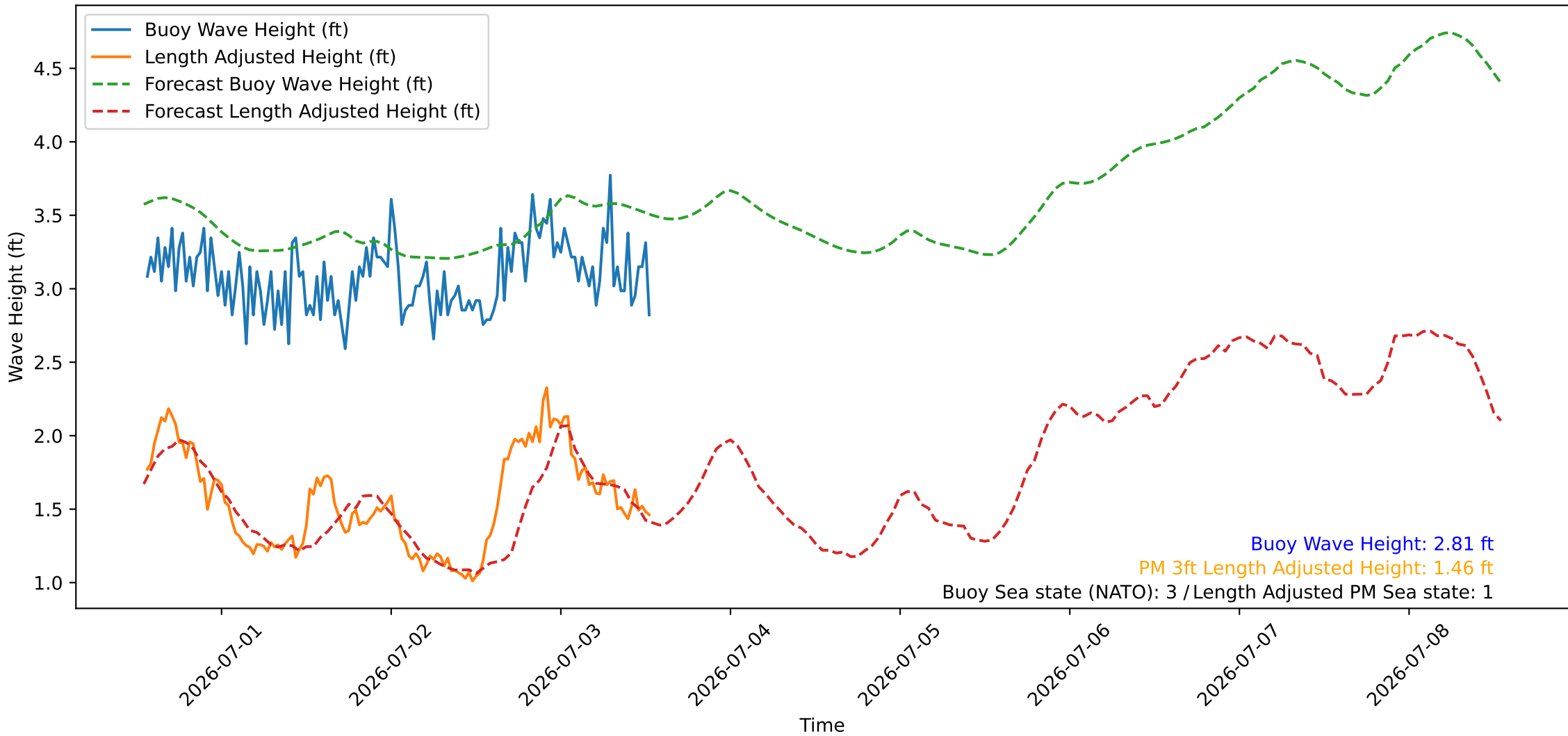
Wave Heights over Time for Oceanside Harbor at 2026-07-03 13:20:26
