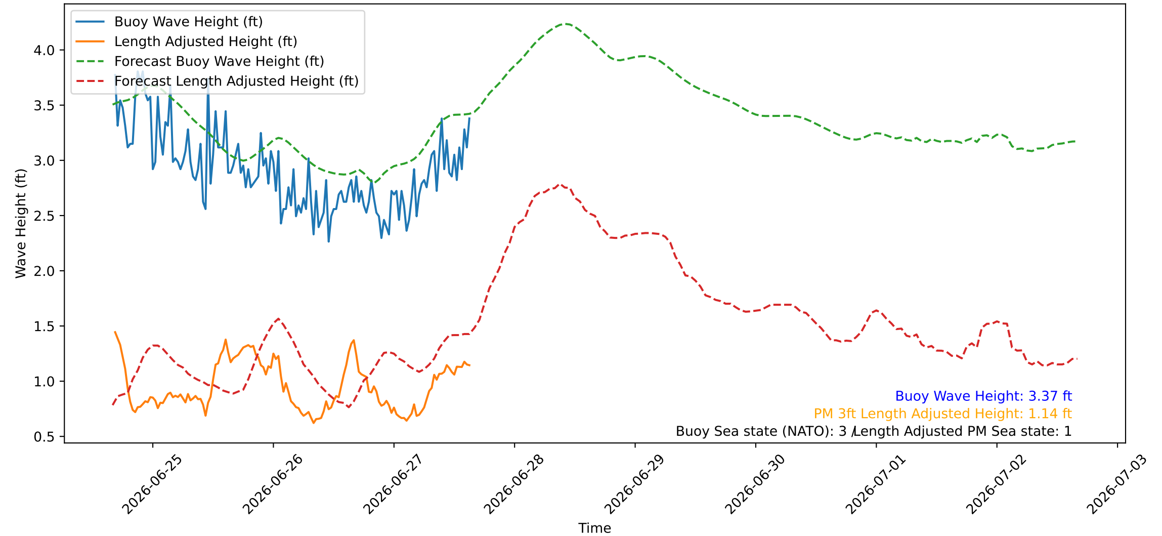
Wave Heights over Time for Red Beach at 2026-06-27 16:00:45
