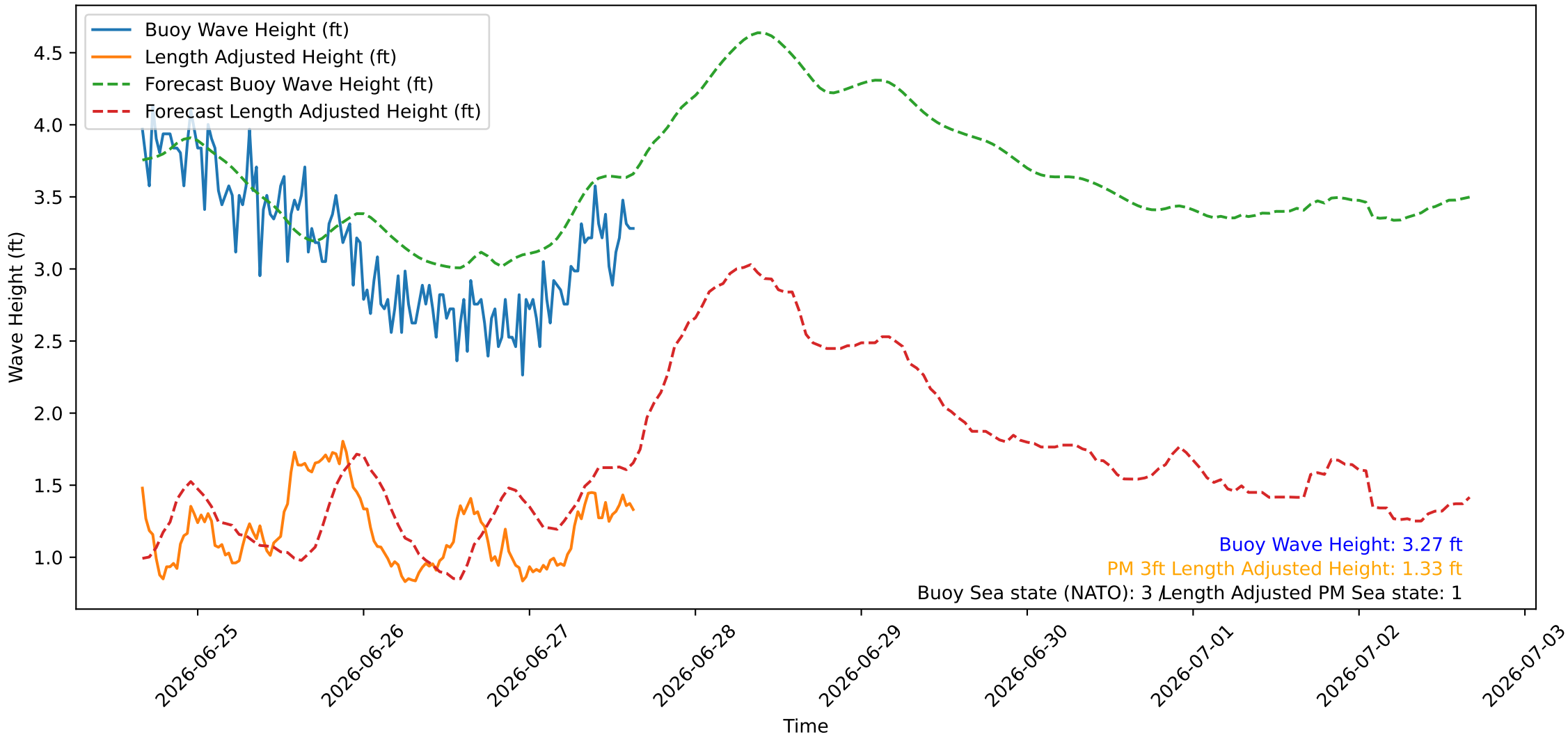
Wave Heights over Time for Green Beach at 2026-06-27 16:01:08
