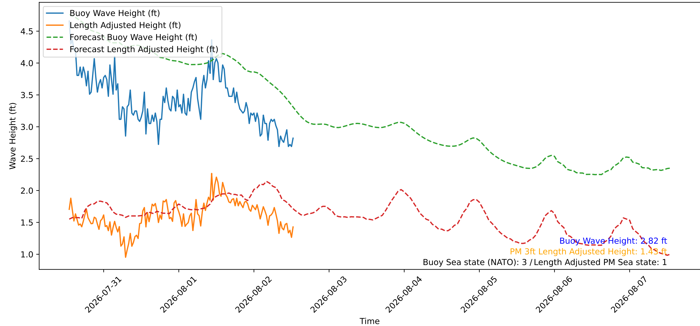
Wave Heights over Time for Oceanside Harbor at 2026-08-02 13:10:26
