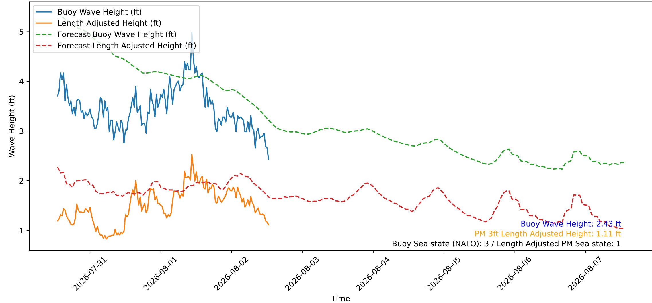
Wave Heights over Time for Green Beach at 2026-08-02 13:11:09
