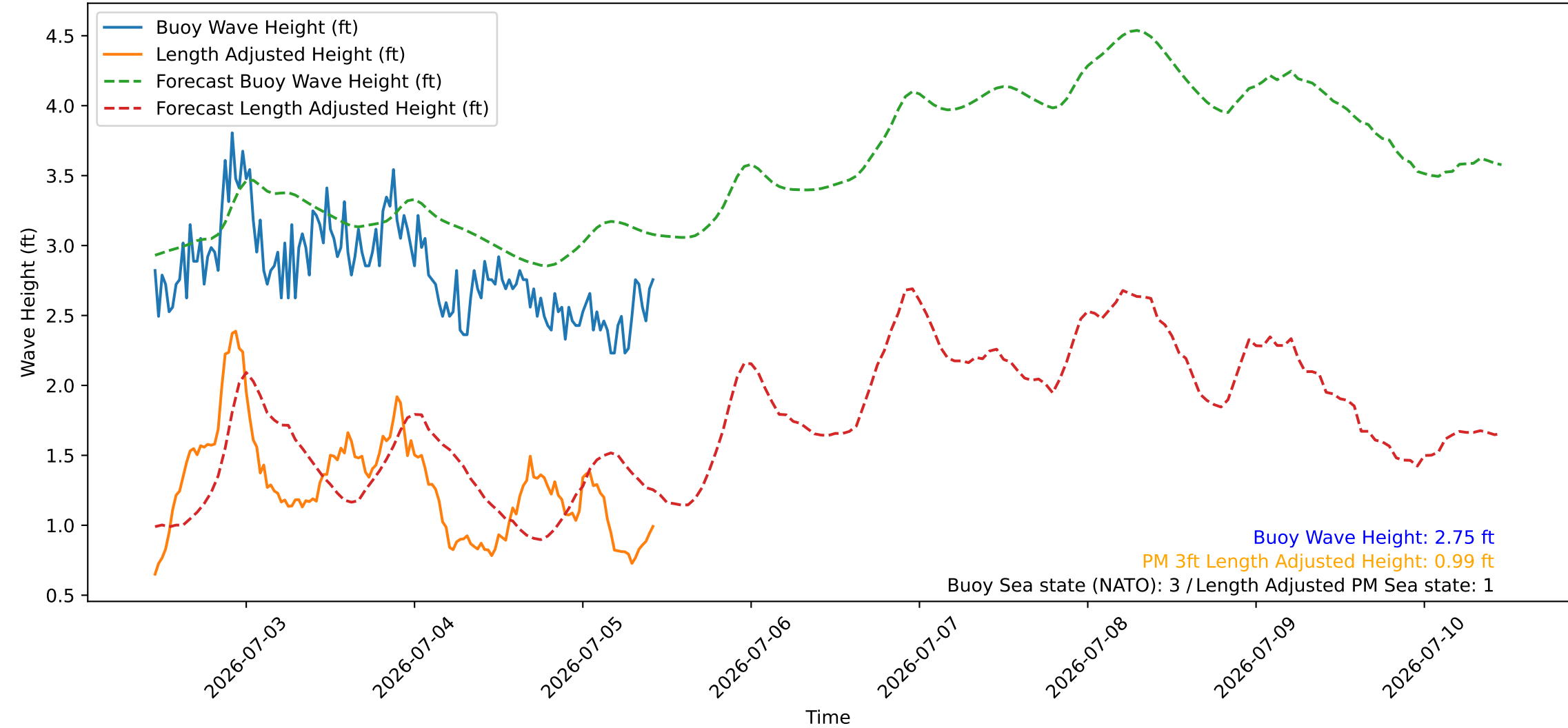
Wave Heights over Time for Red Beach at 2026-07-05 10:50:48
