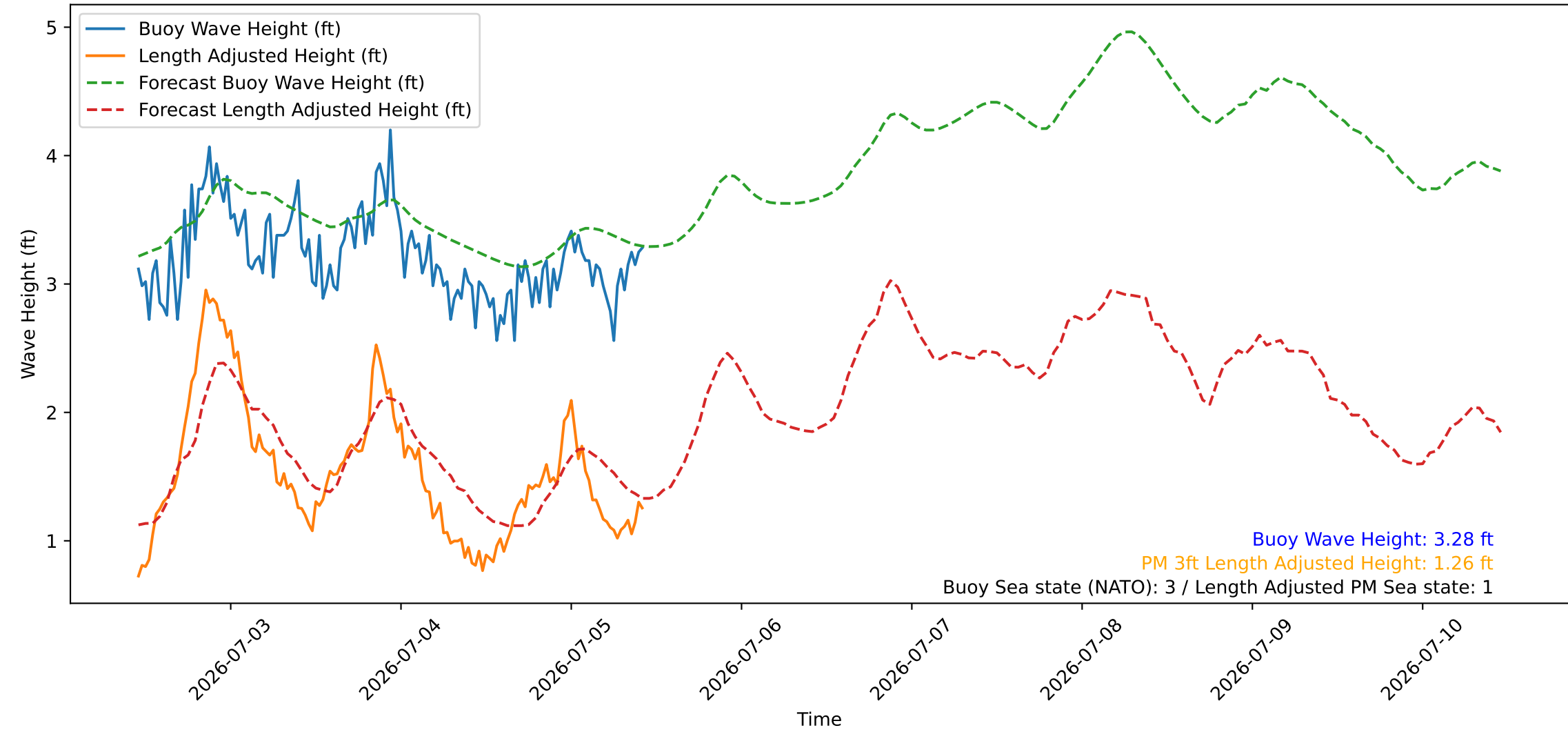
Wave Heights over Time for Green Beach at 2026-07-05 10:51:11
