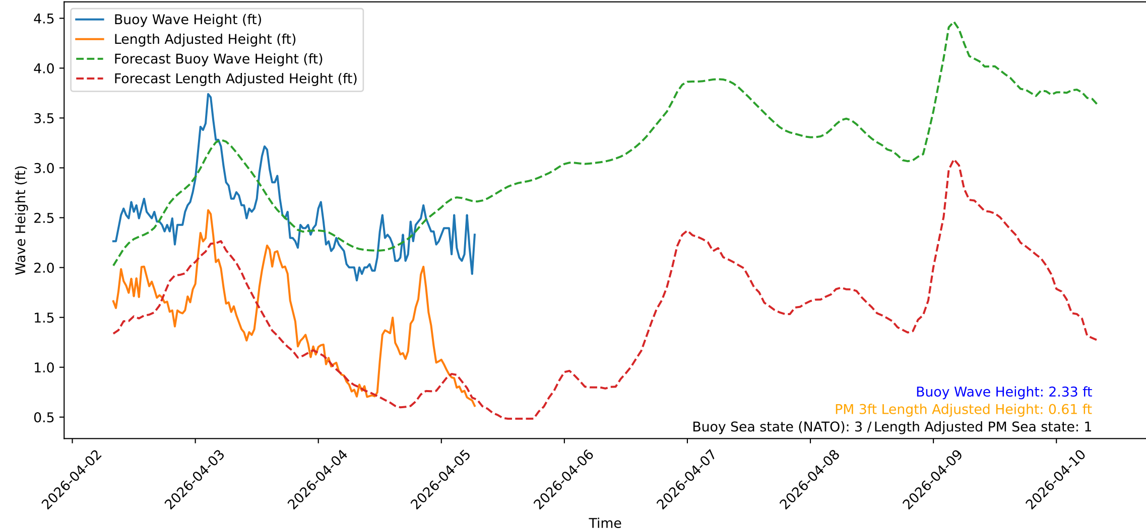
Wave Heights over Time for Red Beach at 2026-04-05 07:30:47
