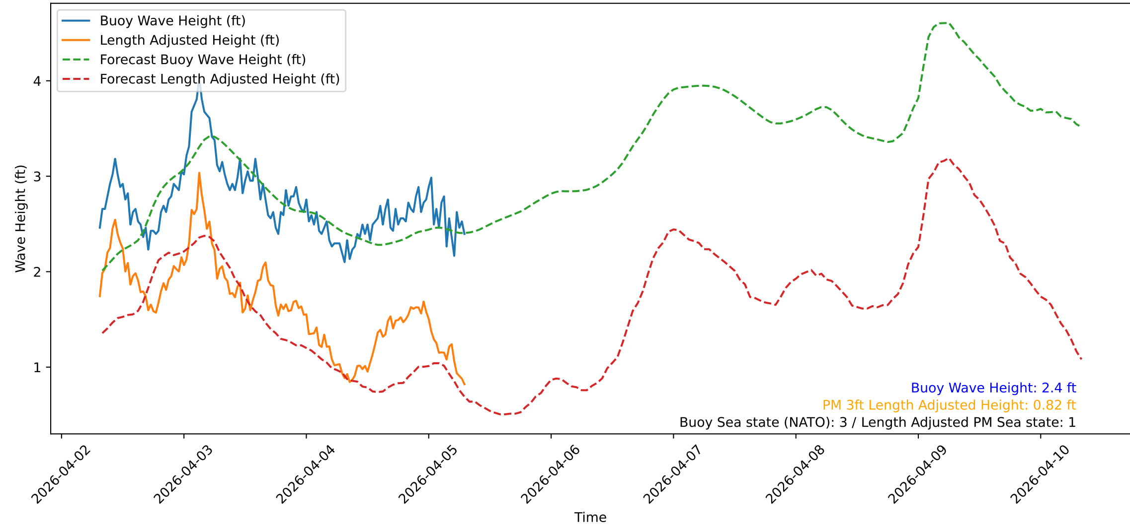
Wave Heights over Time for Oceanside Harbor at 2026-04-05 07:30:32
