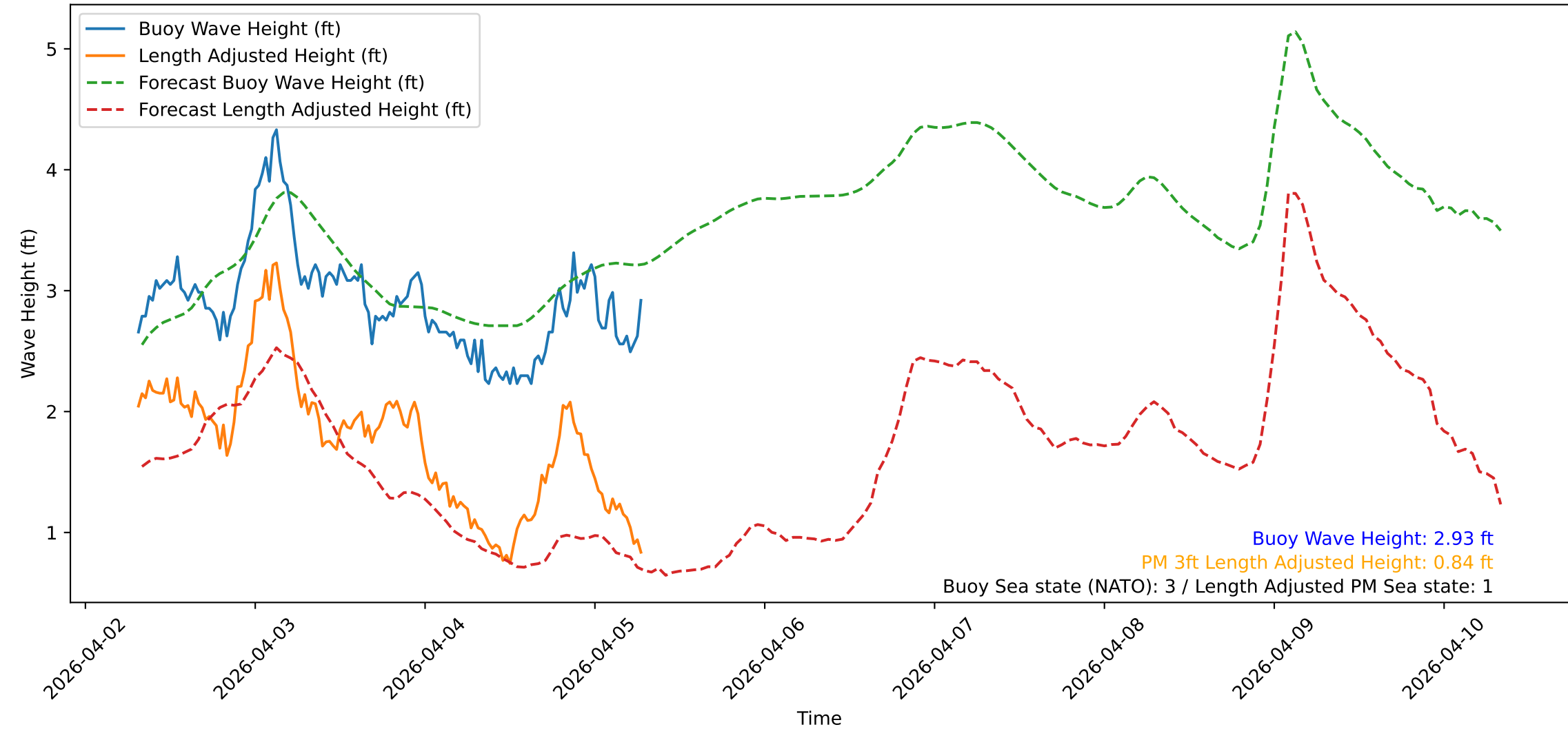
Wave Heights over Time for Green Beach at 2026-04-05 07:31:10
