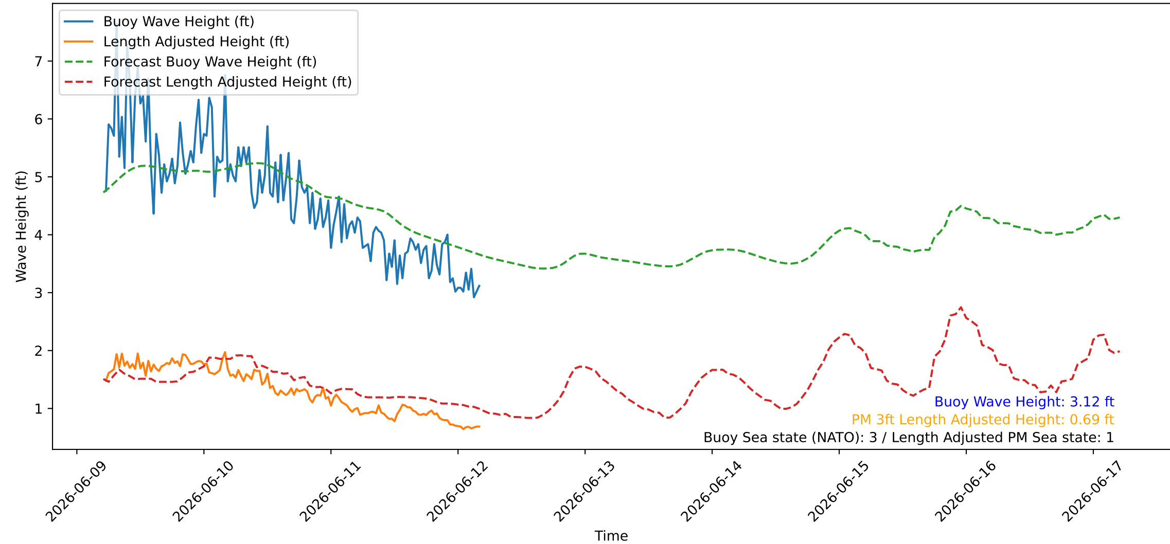
Wave Heights over Time for Red Beach at 2026-06-12 05:00:45
