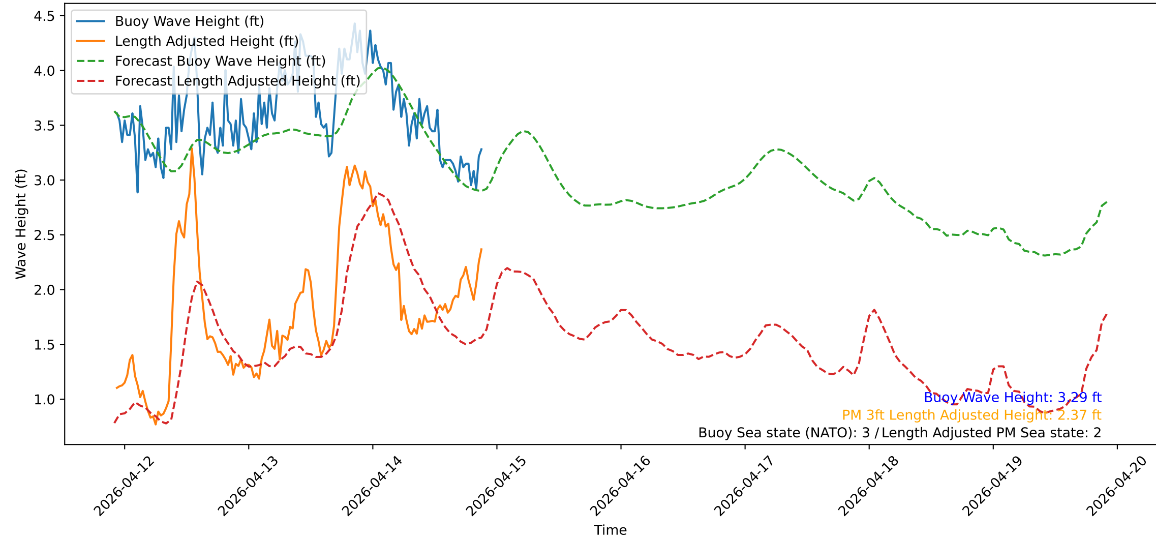
Wave Heights over Time for Red Beach at 2026-04-14 22:00:50
