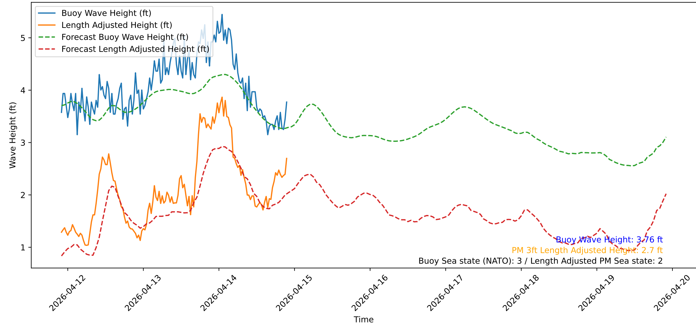
Wave Heights over Time for Oceanside Harbor at 2026-04-14 22:00:31
