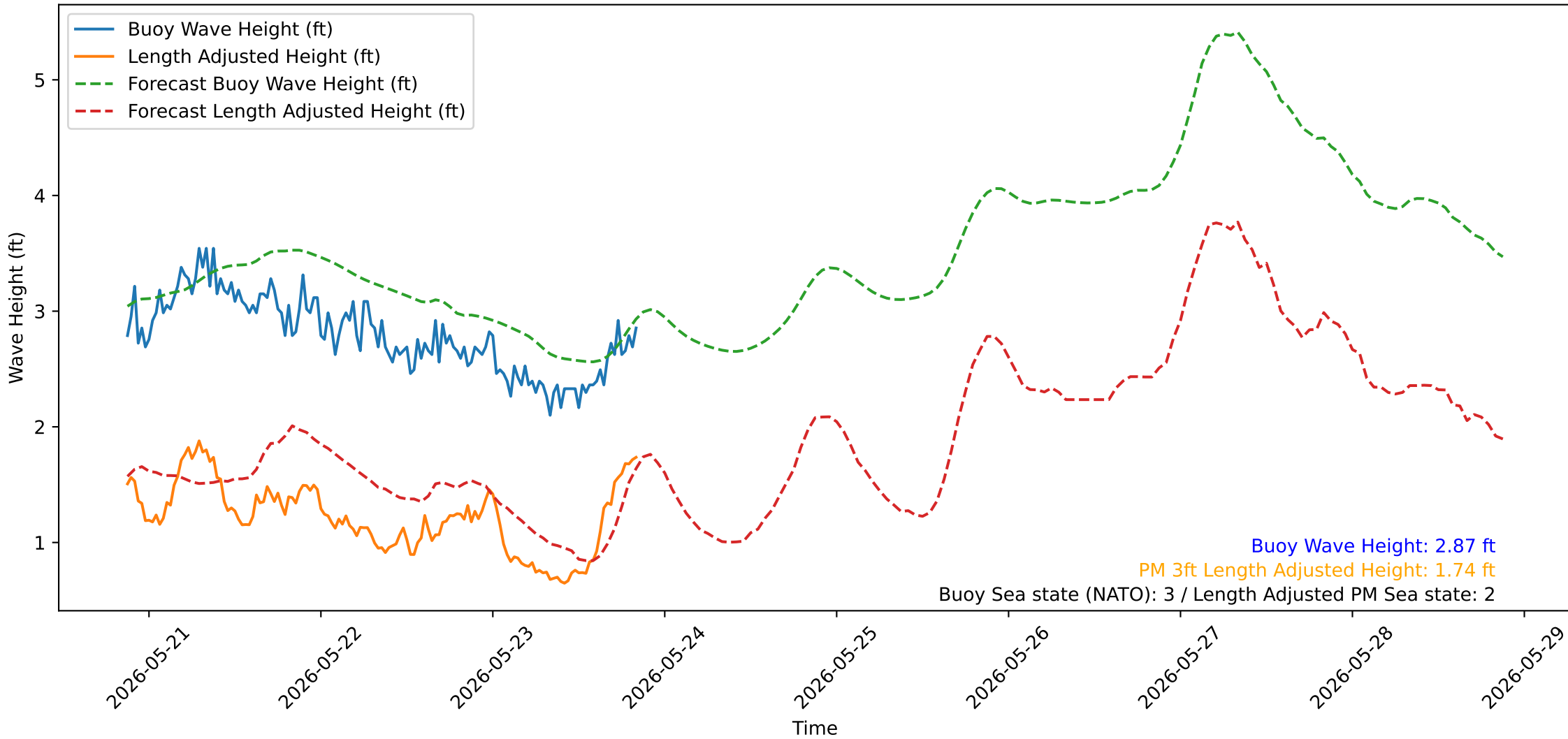
Wave Heights over Time for Green Beach at 2026-05-23 20:51:14
