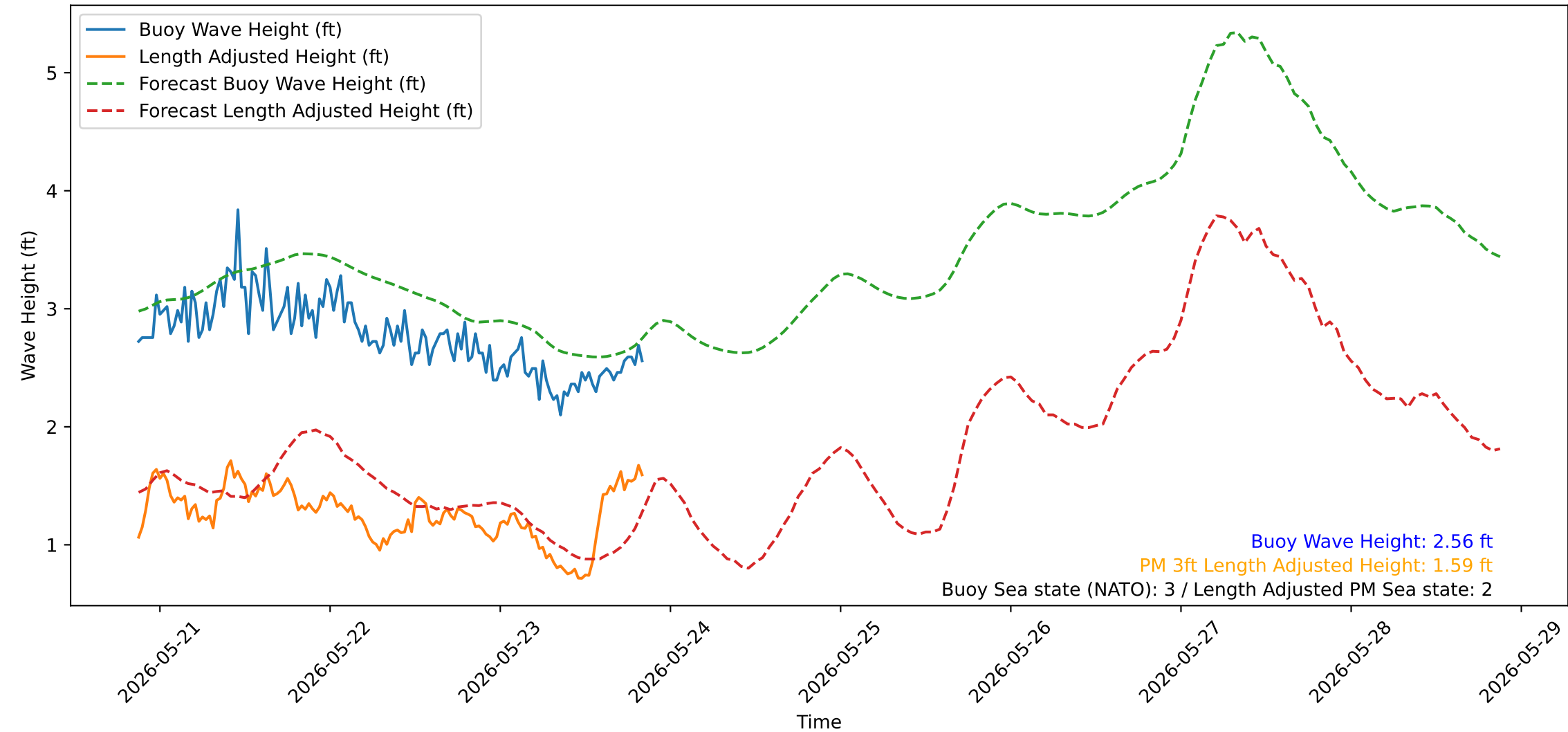
Wave Heights over Time for Oceanside Harbor at 2026-05-23 20:50:31
