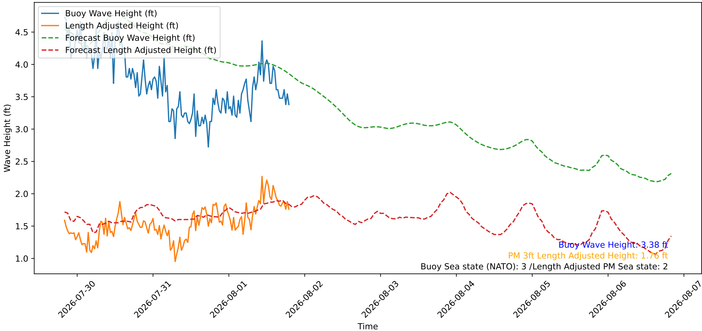
Wave Heights over Time for Oceanside Harbor at 2026-08-01 19:50:26
