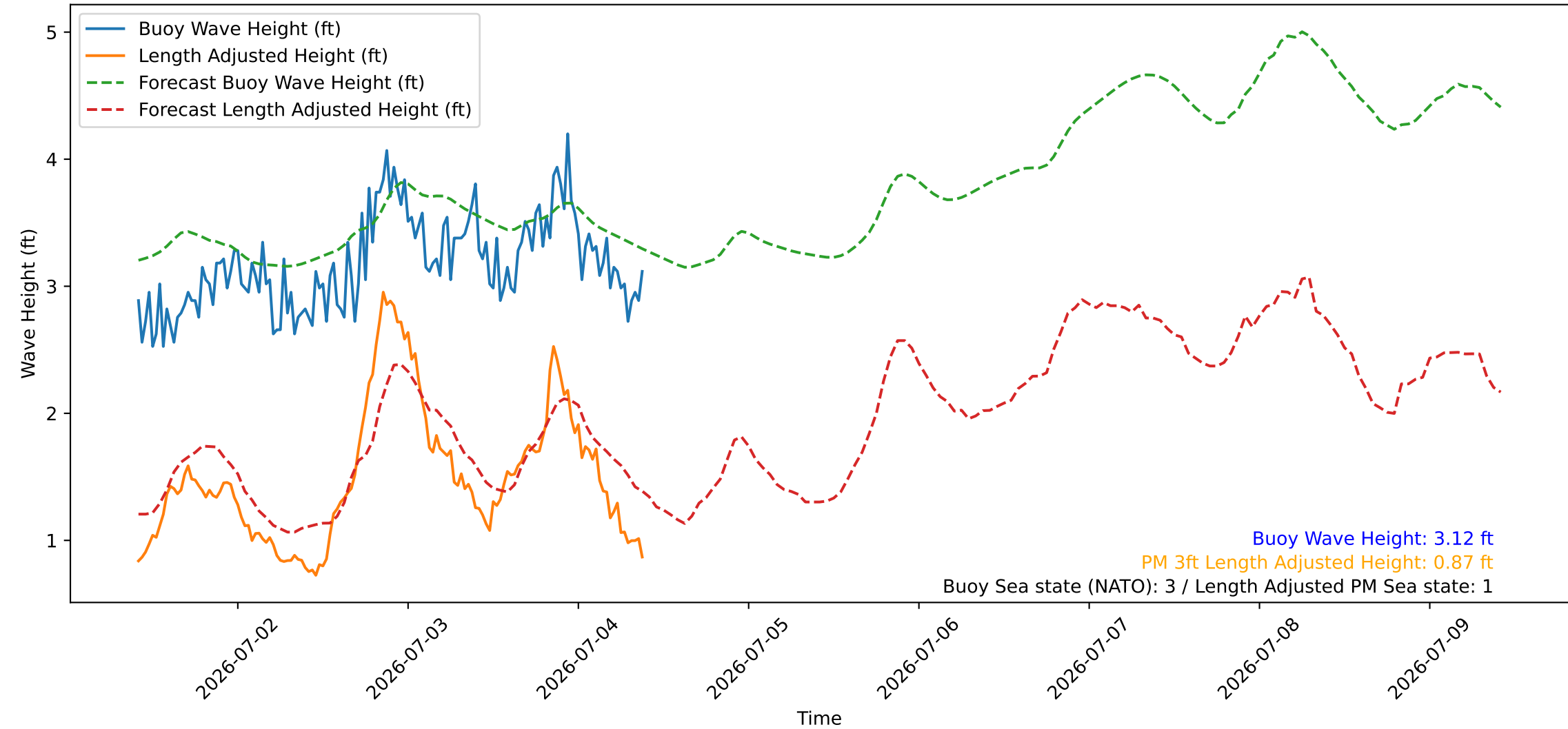
Wave Heights over Time for Green Beach at 2026-07-04 10:01:08
