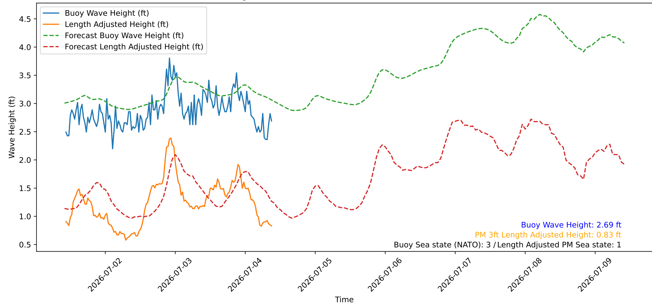
Wave Heights over Time for Red Beach at 2026-07-04 10:00:45
