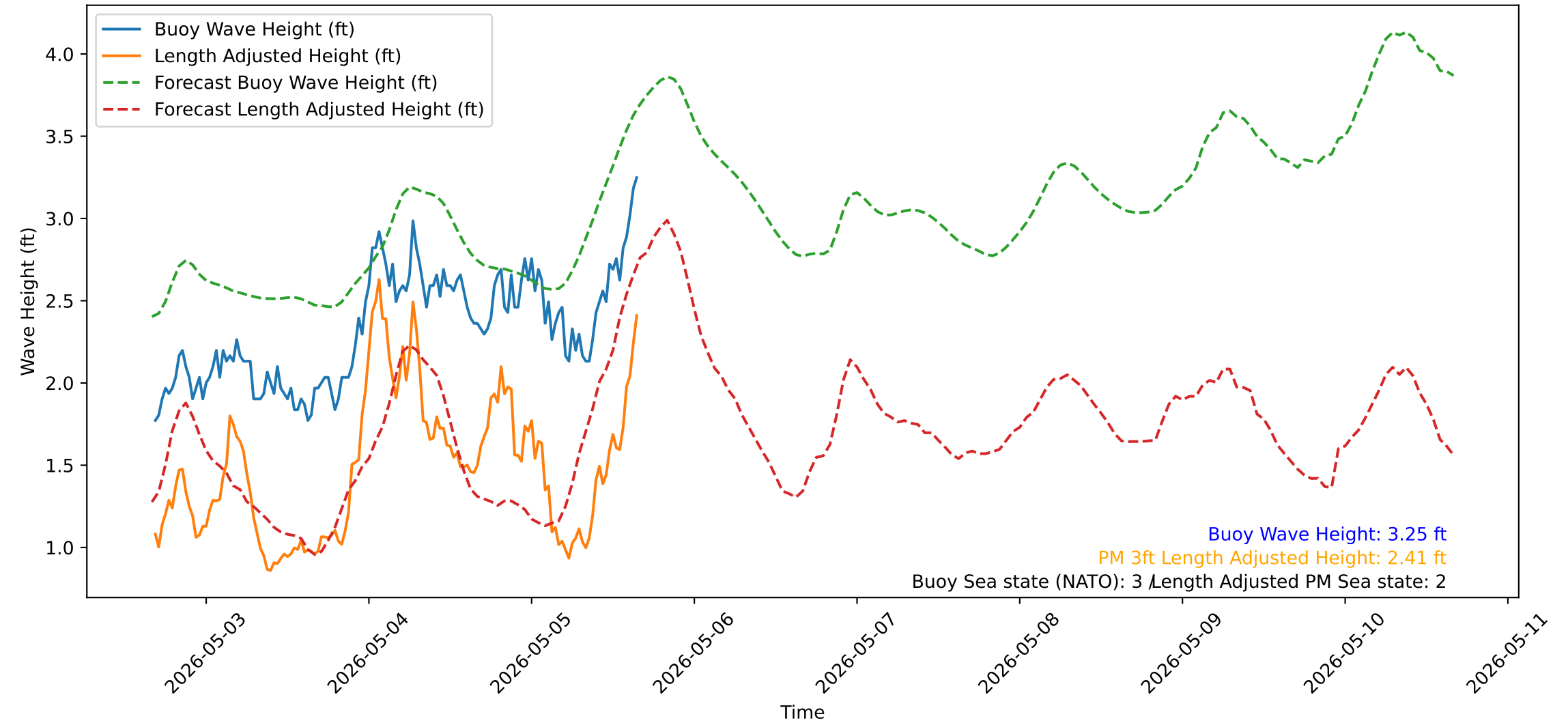
Wave Heights over Time for Green Beach at 2026-05-05 16:21:13
