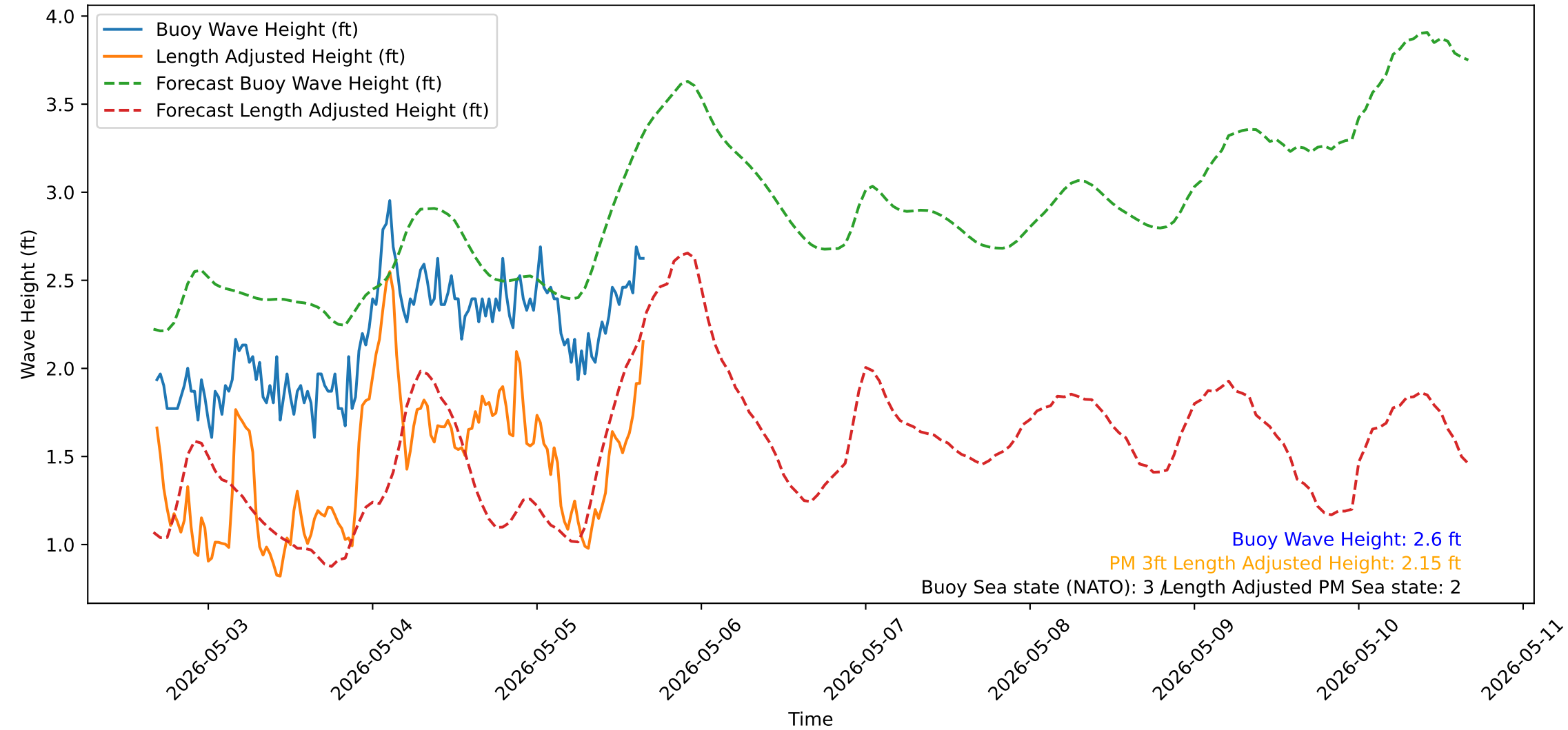
Wave Heights over Time for Red Beach at 2026-05-05 16:20:51
