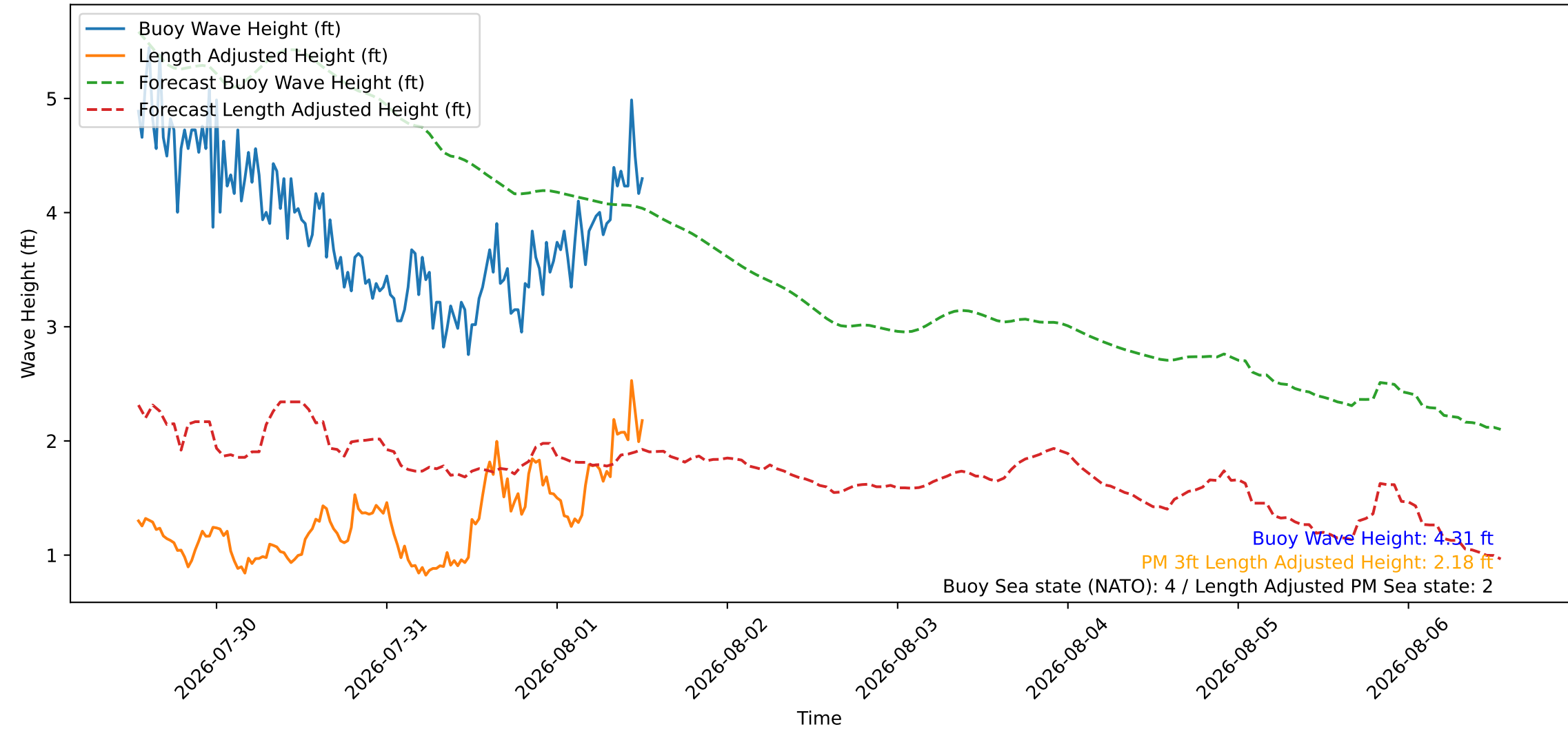
Wave Heights over Time for Green Beach at 2026-08-01 12:51:10
