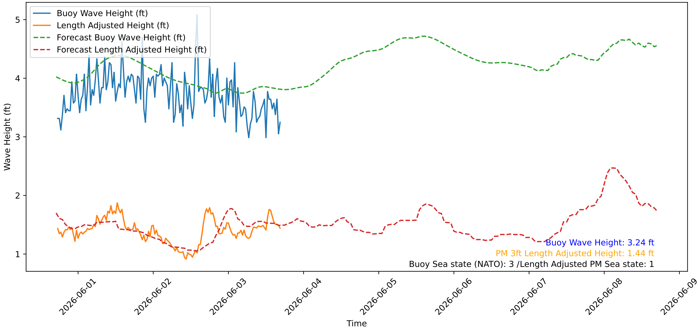
Wave Heights over Time for Oceanside Harbor at 2026-06-03 17:20:26
