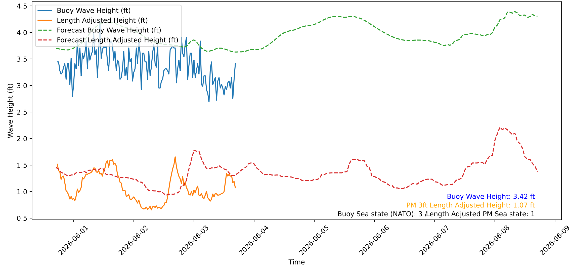
Wave Heights over Time for Red Beach at 2026-06-03 17:20:46
