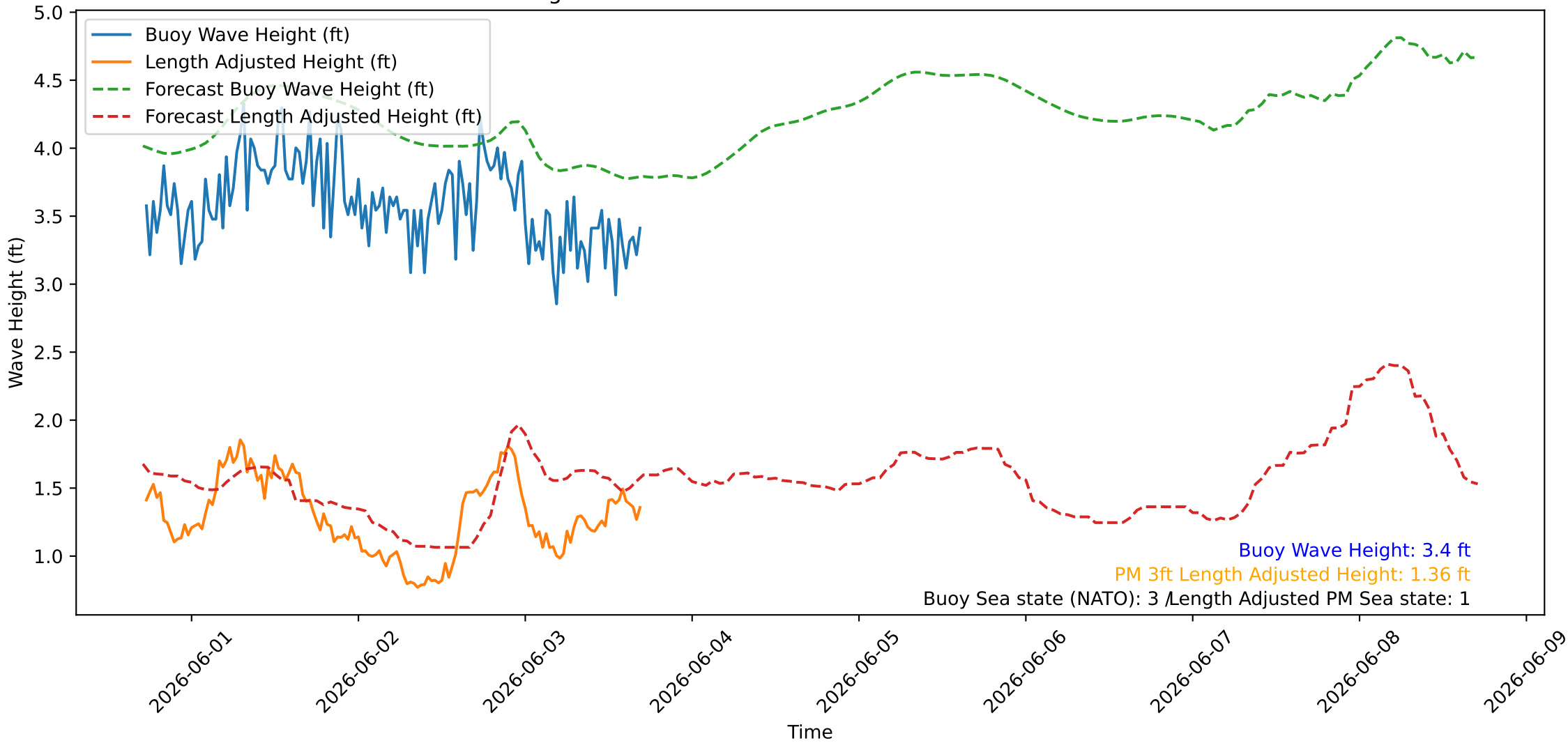
Wave Heights over Time for Green Beach at 2026-06-03 17:21:09
