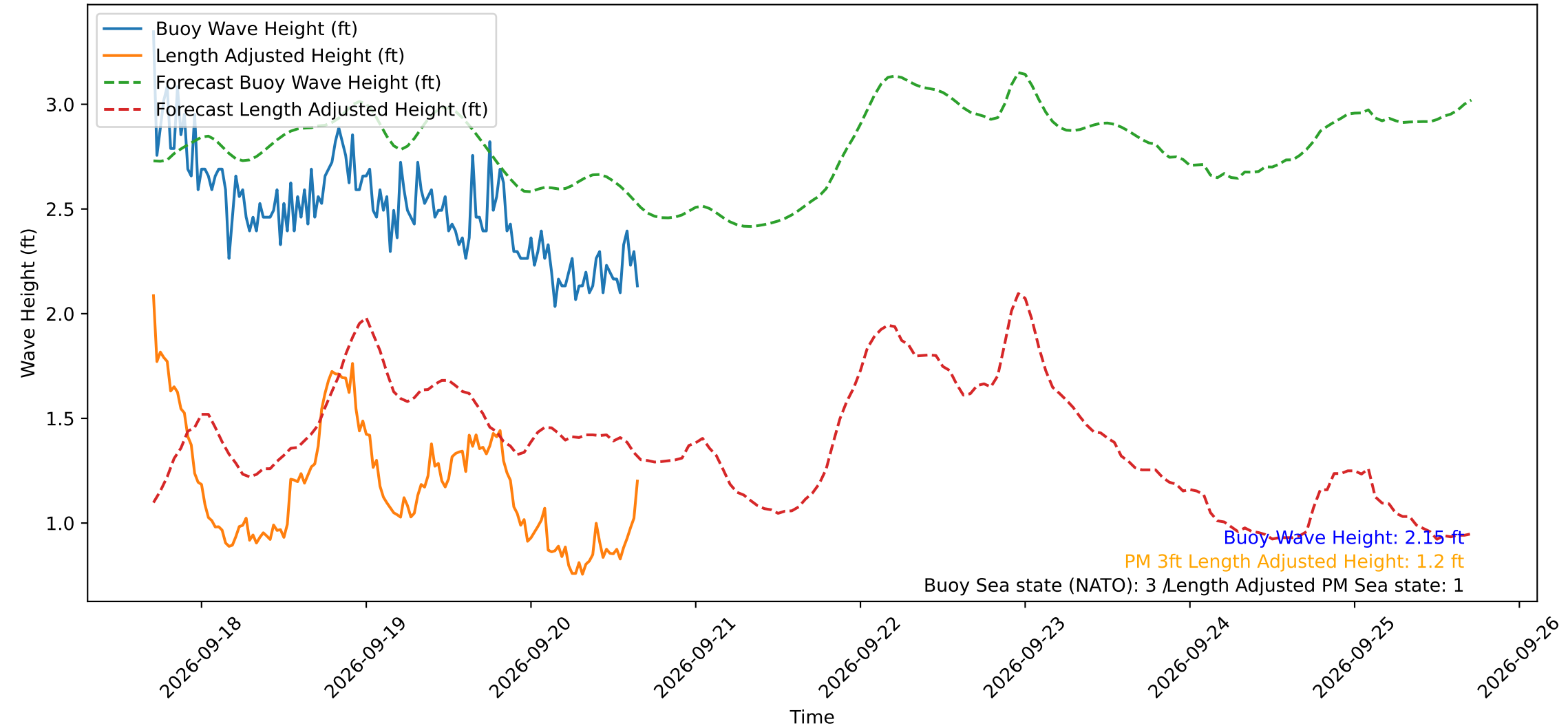
Wave Heights over Time for Red Beach at 2026-09-20 16:30:48
