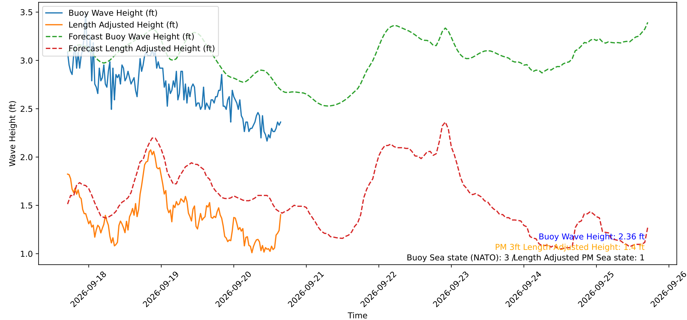
Wave Heights over Time for Green Beach at 2026-09-20 16:31:11
