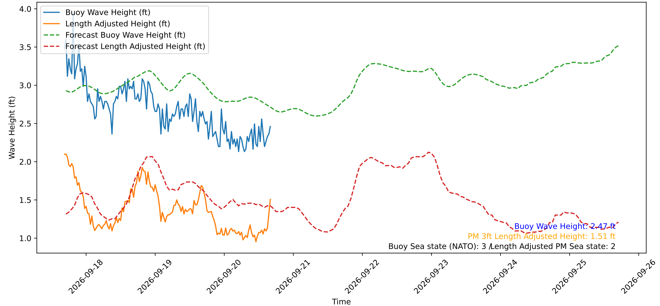
Wave Heights over Time for Oceanside Harbor at 2026-09-20 16:30:29
