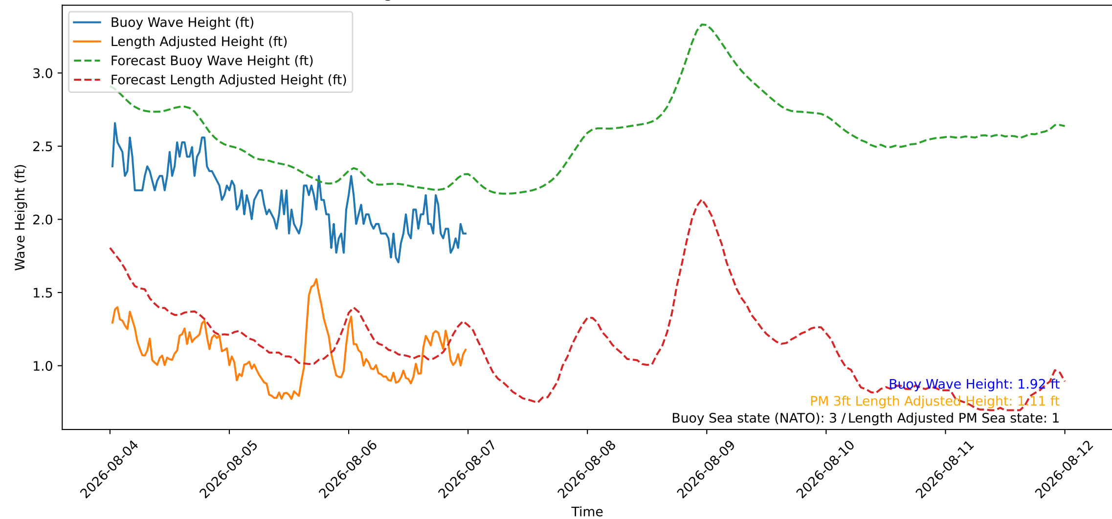
Wave Heights over Time for Oceanside Harbor at 2026-08-07 00:20:26
