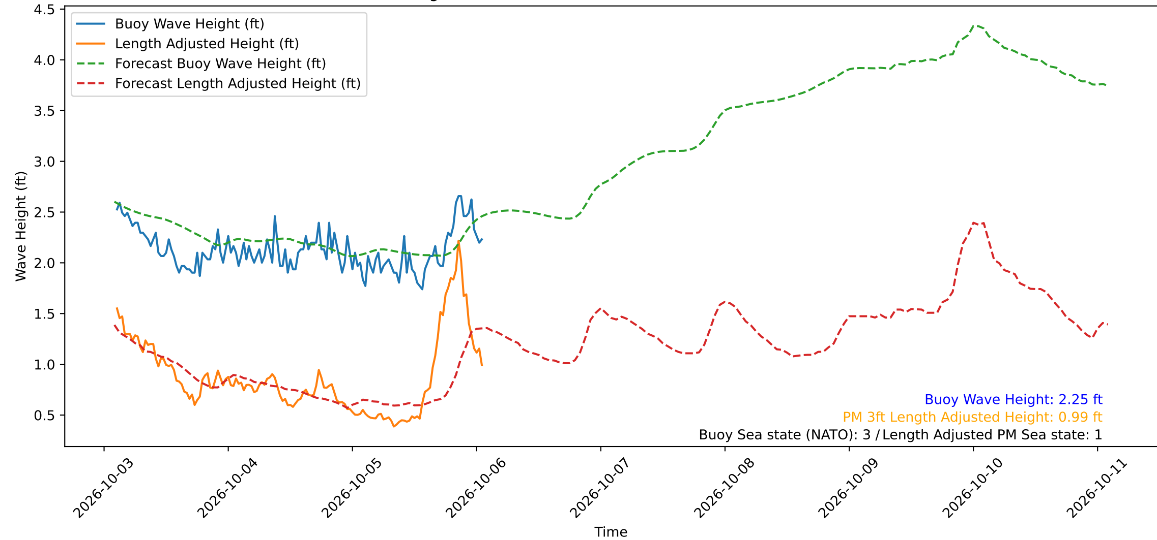
Wave Heights over Time for Red Beach at 2026-10-06 02:00:48
