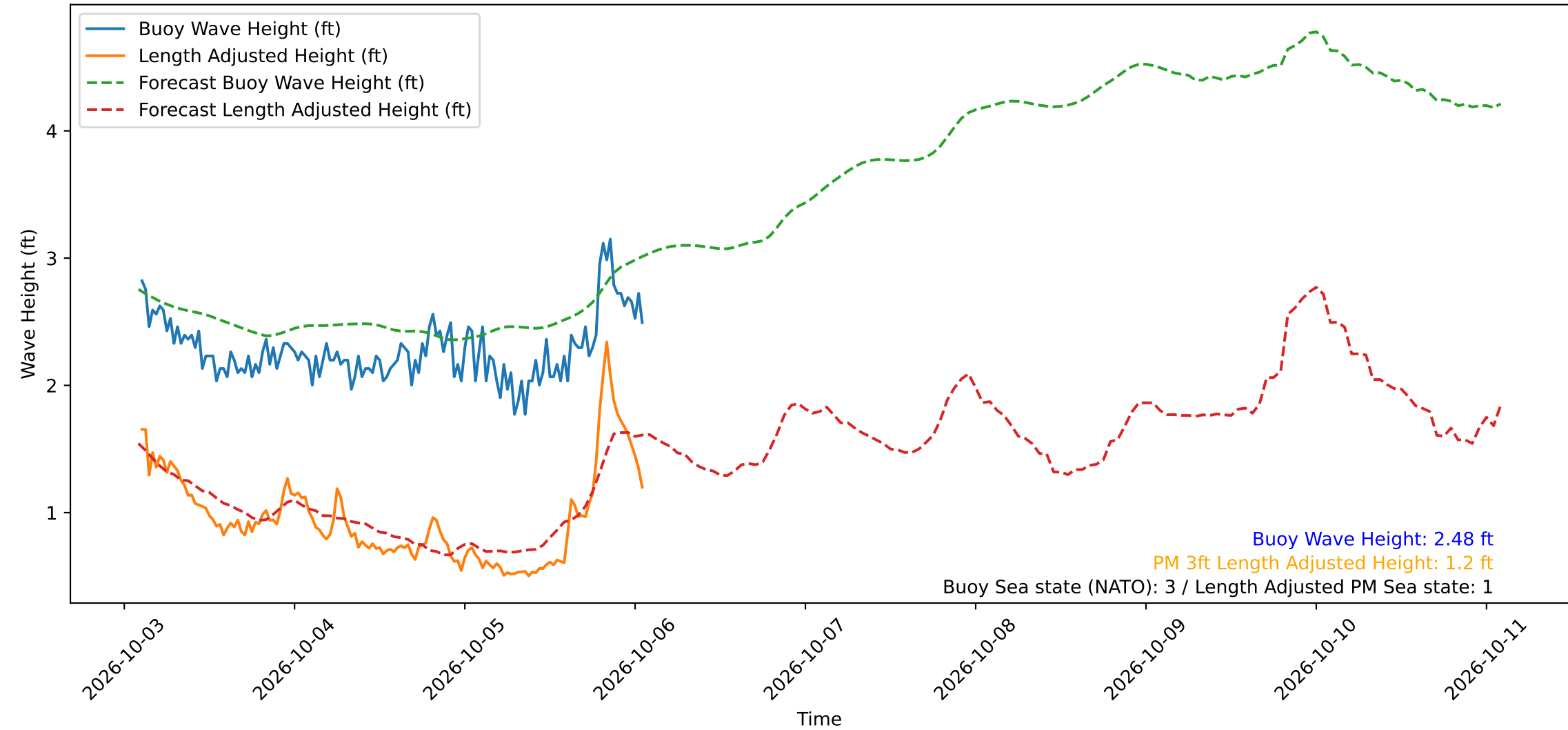
Wave Heights over Time for Green Beach at 2026-10-06 02:01:11
