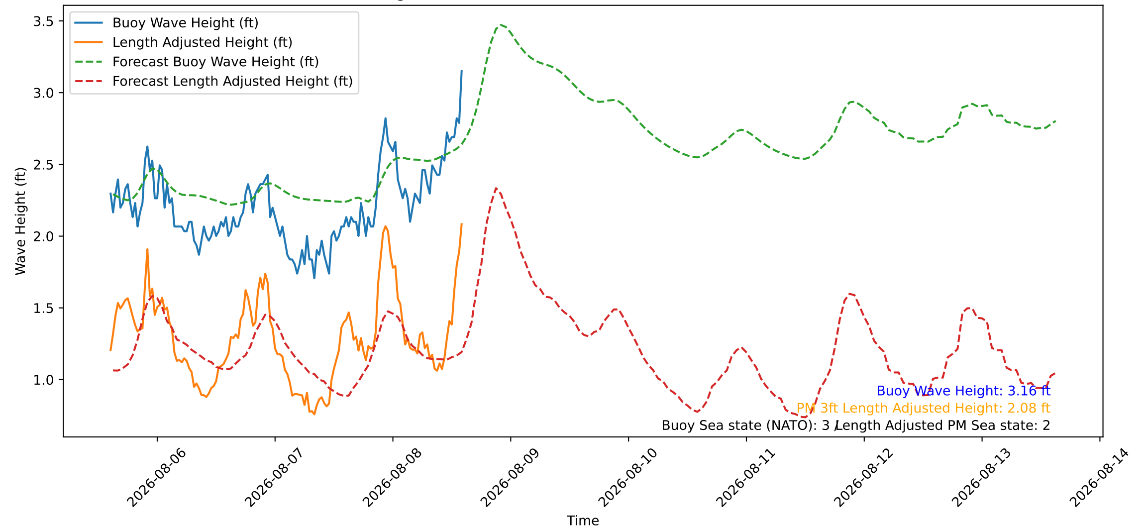
Wave Heights over Time for Green Beach at 2026-08-08 14:41:08
