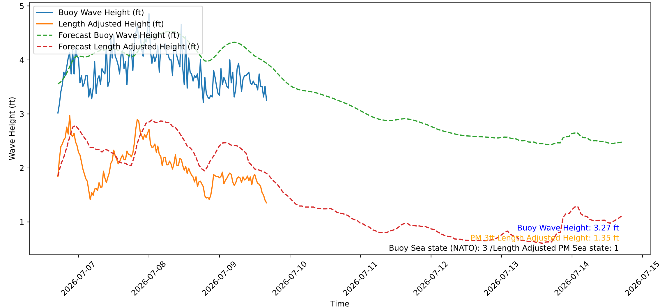
Wave Heights over Time for Red Beach at 2026-07-09 16:50:47
