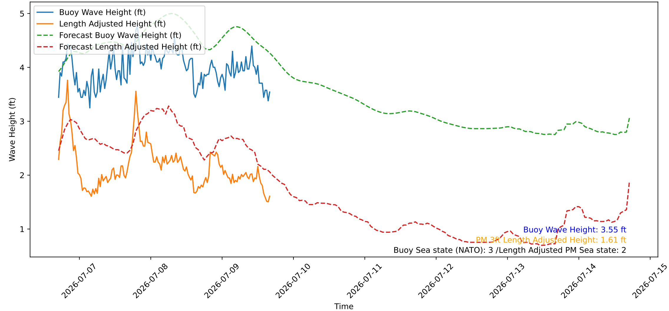
Wave Heights over Time for Green Beach at 2026-07-09 16:51:10
