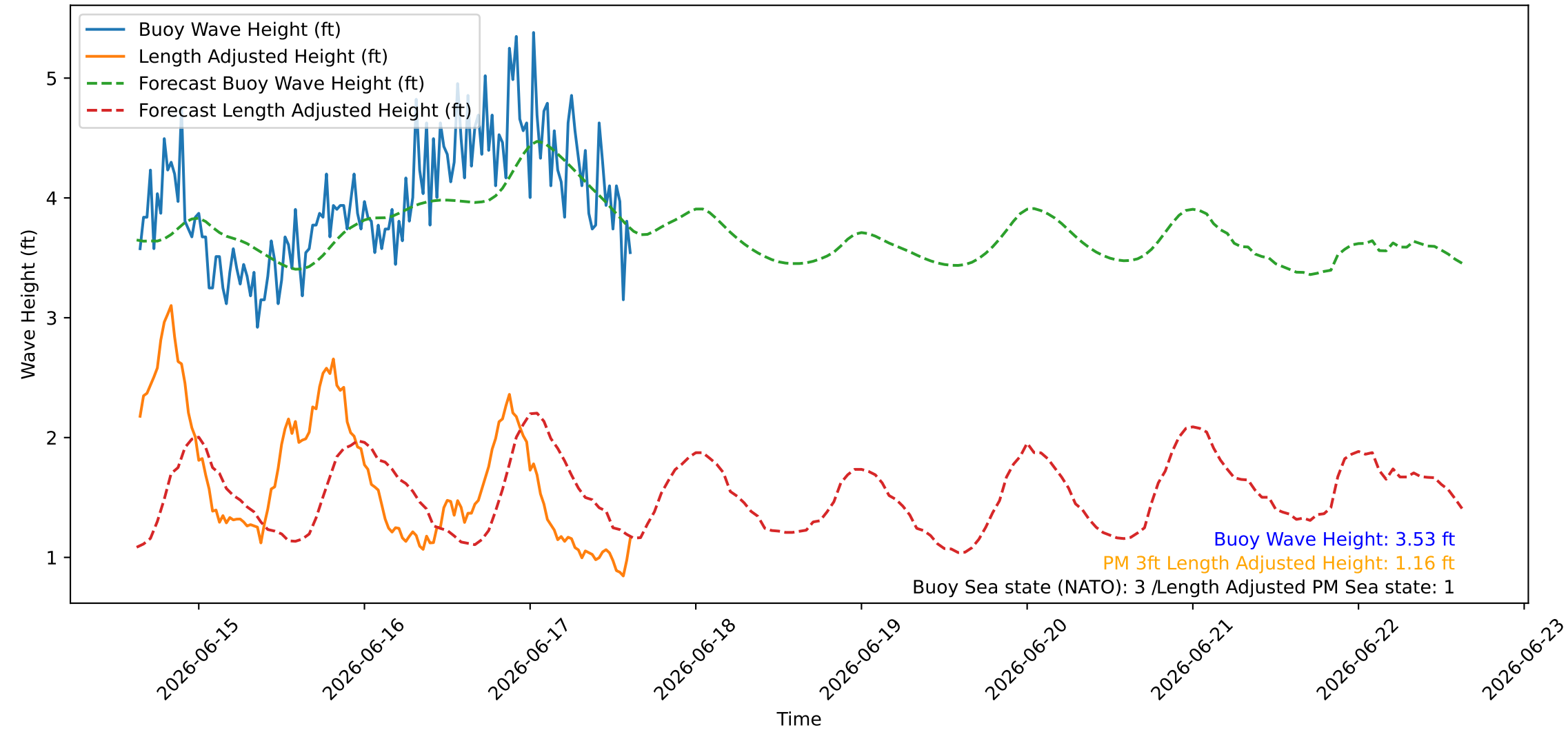
Wave Heights over Time for Red Beach at 2026-06-17 15:20:47
