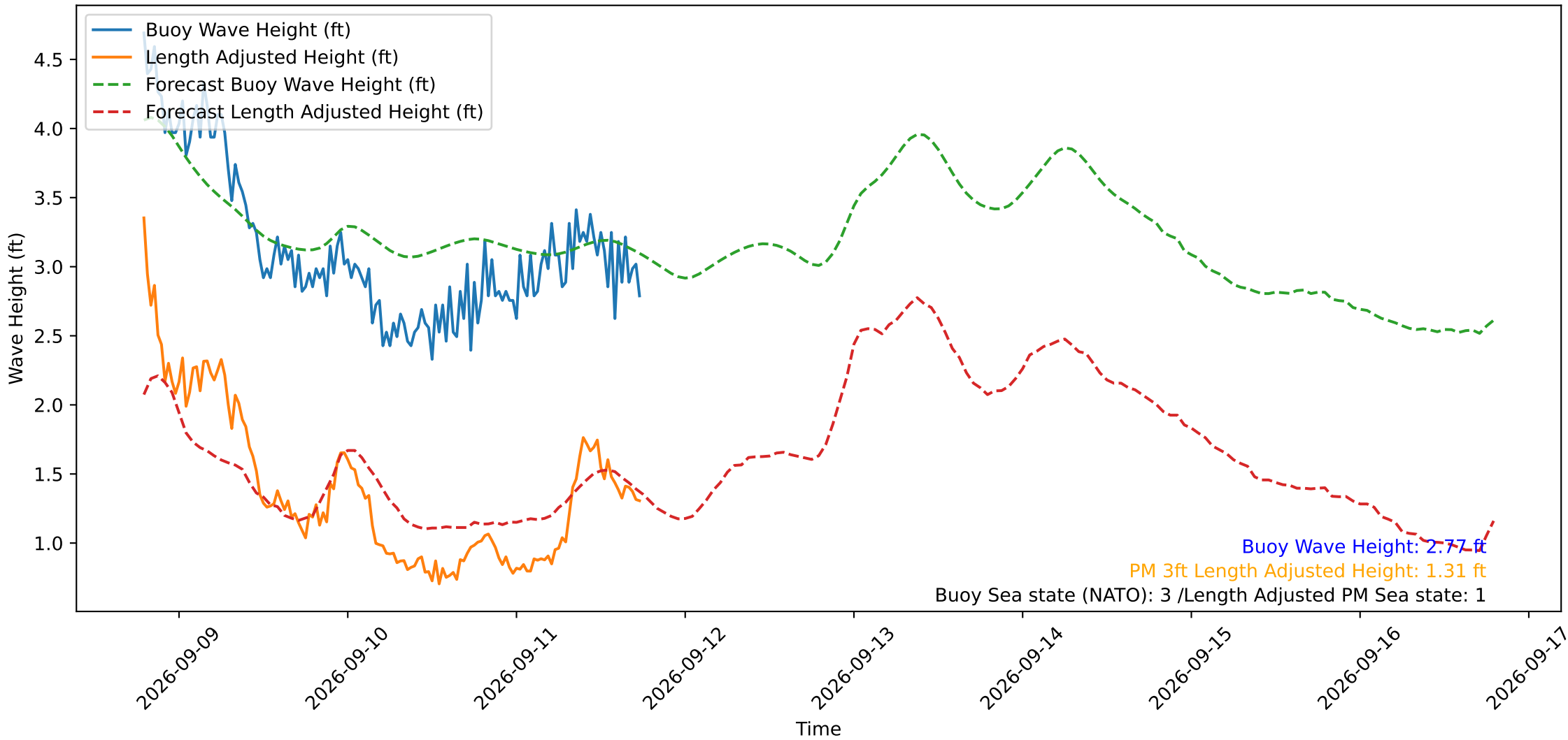
Wave Heights over Time for Red Beach at 2026-09-11 18:30:50
