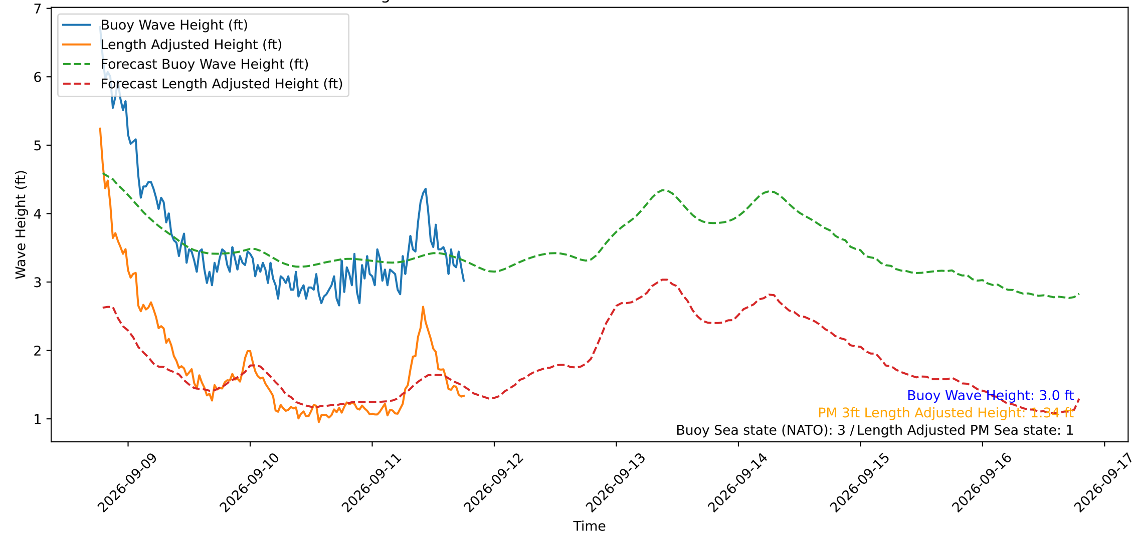
Wave Heights over Time for Oceanside Harbor at 2026-09-11 18:30:30
