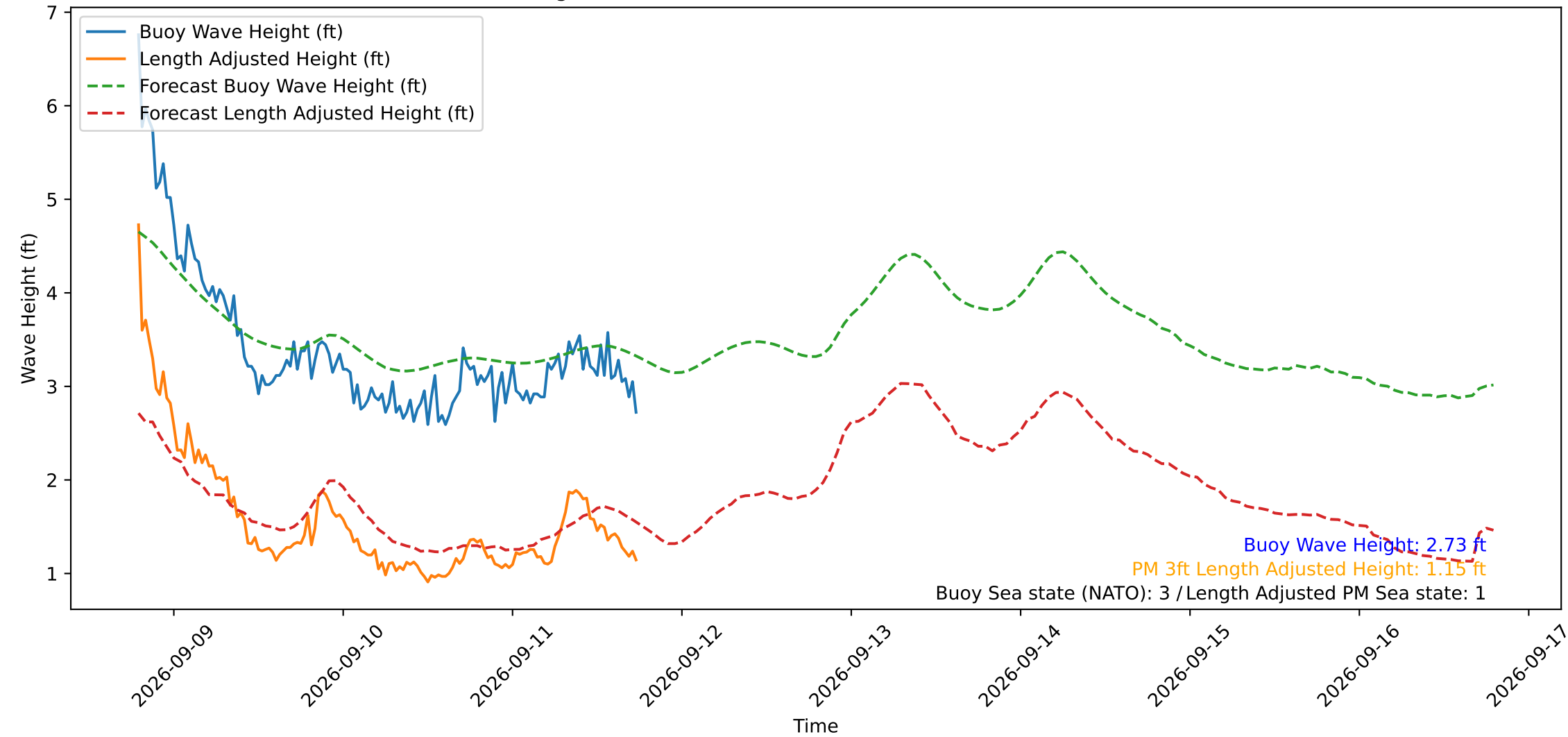
Wave Heights over Time for Green Beach at 2026-09-11 18:31:13
