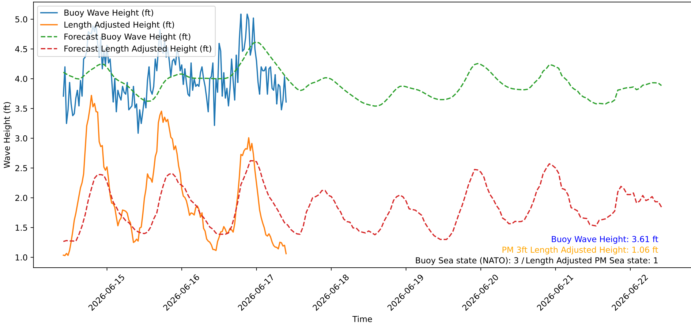
Wave Heights over Time for Green Beach at 2026-06-17 10:11:08
