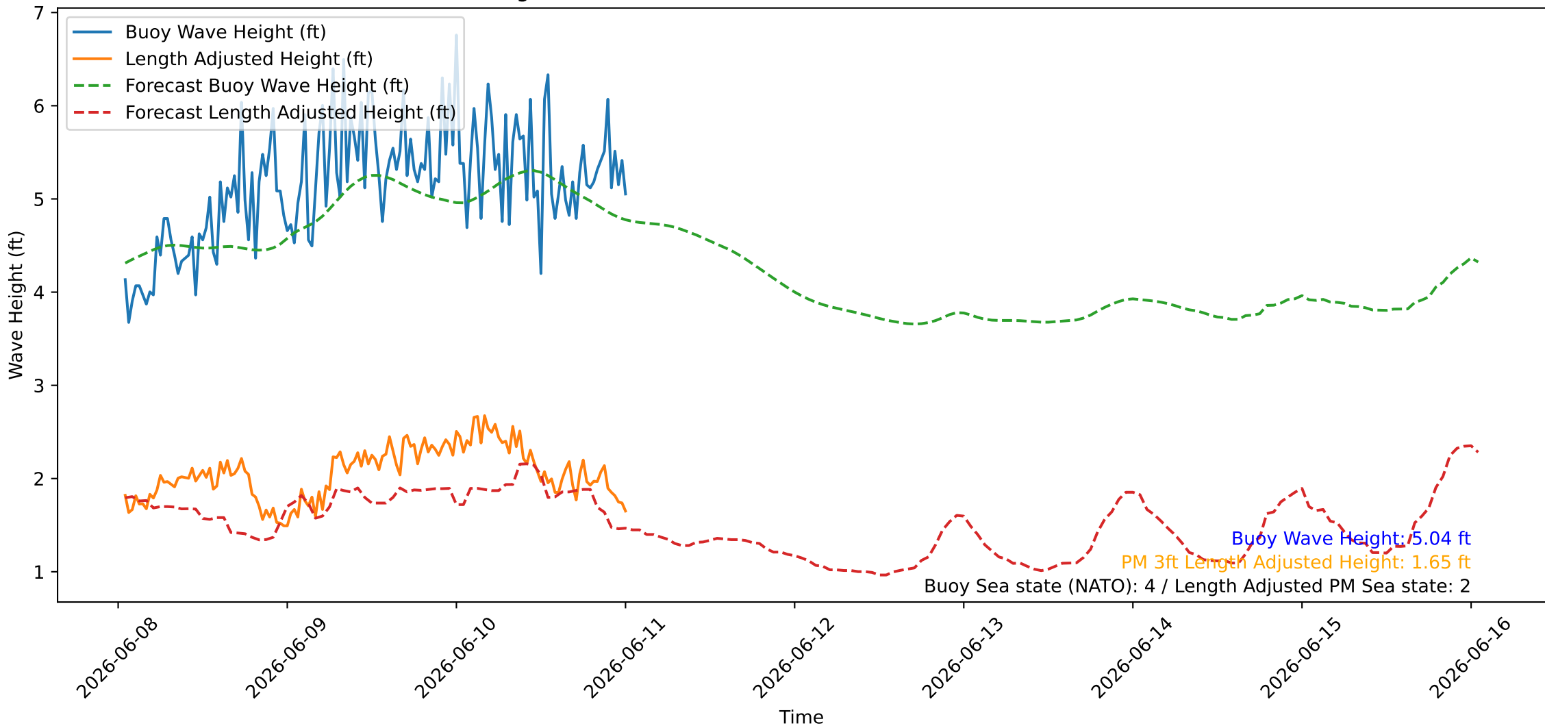
Wave Heights over Time for Oceanside Harbor at 2026-06-11 00:50:26
