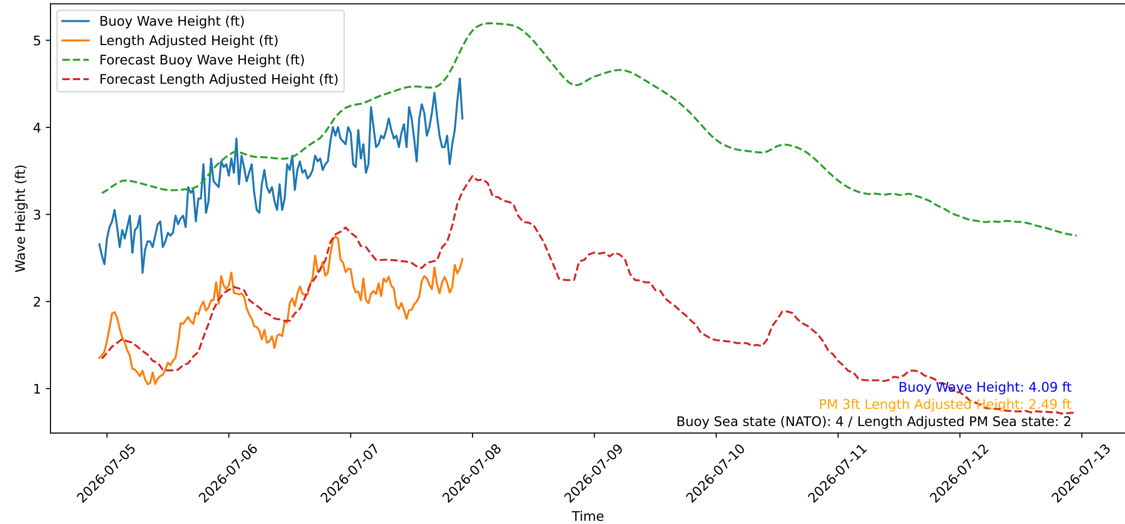
Wave Heights over Time for Oceanside Harbor at 2026-07-07 22:30:27
