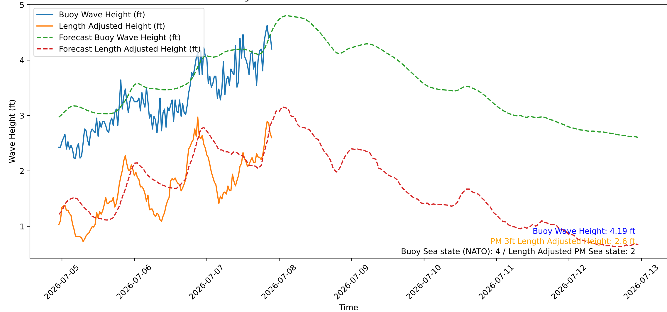
Wave Heights over Time for Red Beach at 2026-07-07 22:30:46
