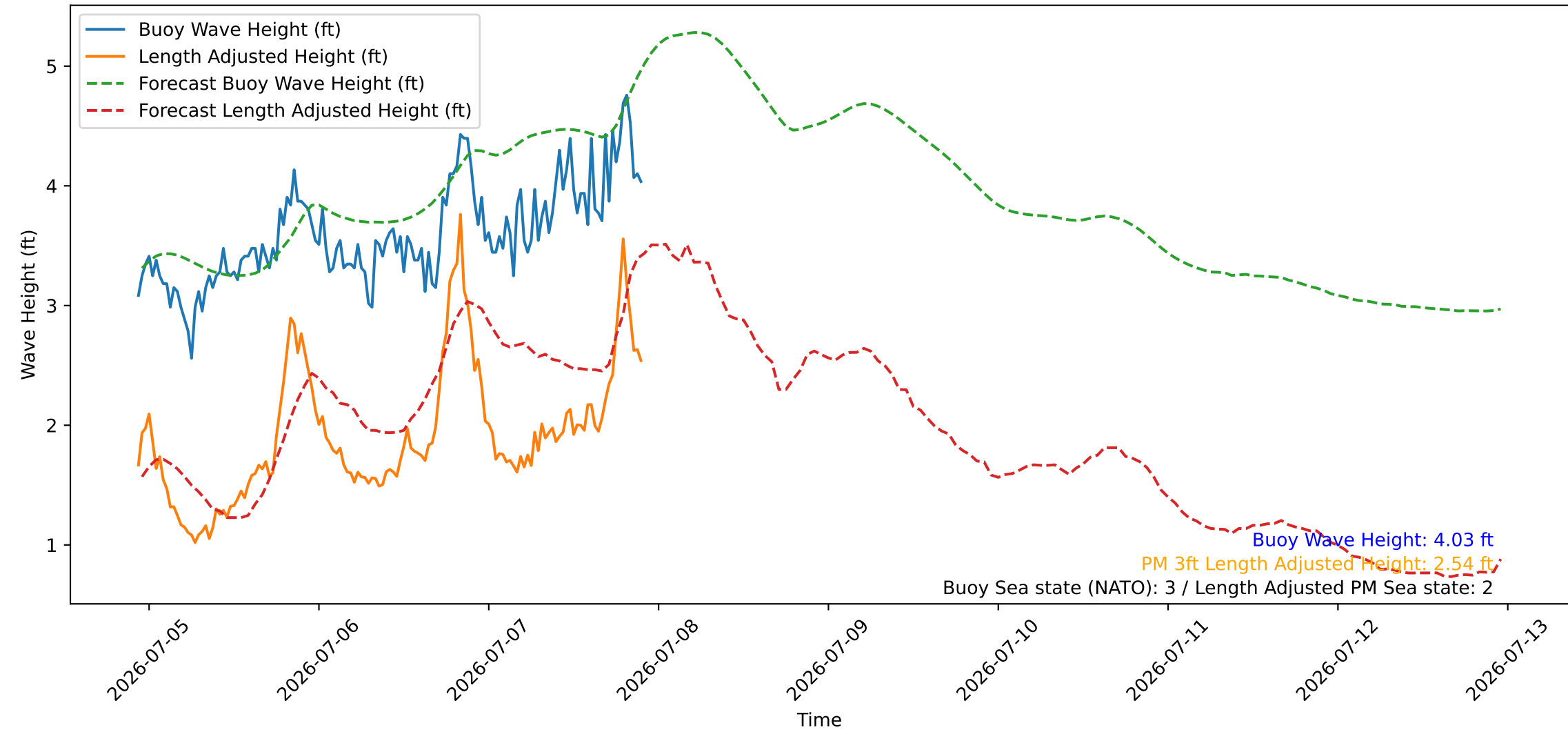
Wave Heights over Time for Green Beach at 2026-07-07 22:31:09
