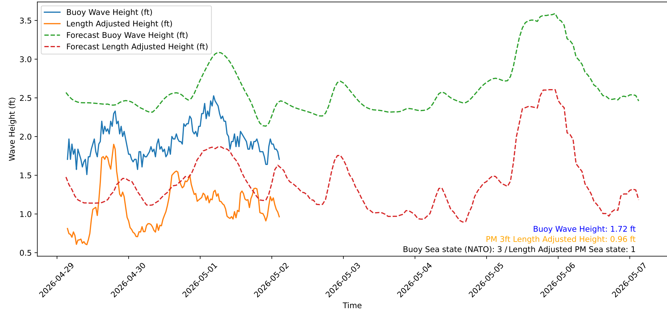
Wave Heights over Time for Red Beach at 2026-05-02 03:10:50
