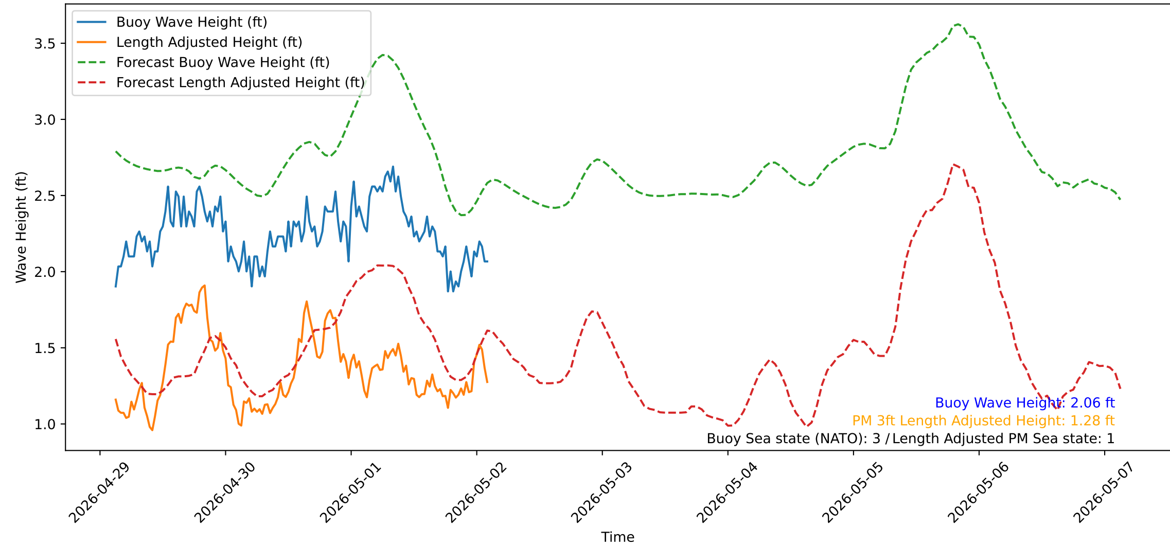
Wave Heights over Time for Oceanside Harbor at 2026-05-02 03:10:31
