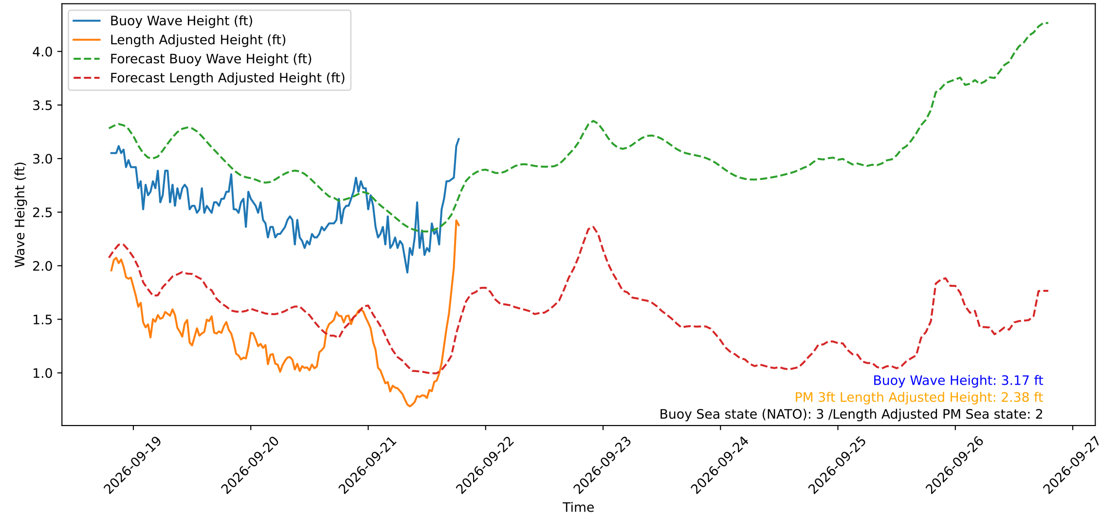
Wave Heights over Time for Green Beach at 2026-09-21 19:11:13
