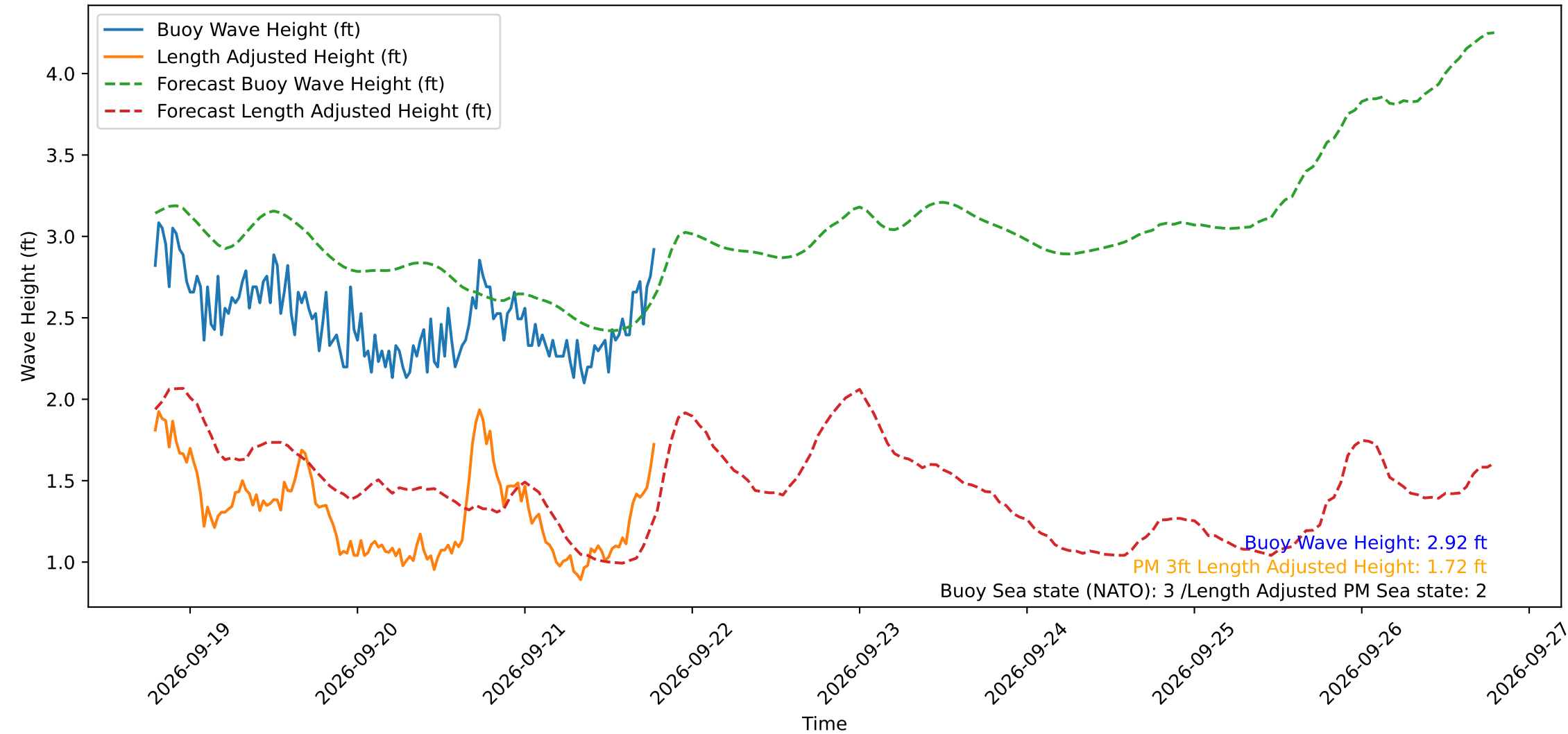
Wave Heights over Time for Oceanside Harbor at 2026-09-21 19:10:30
