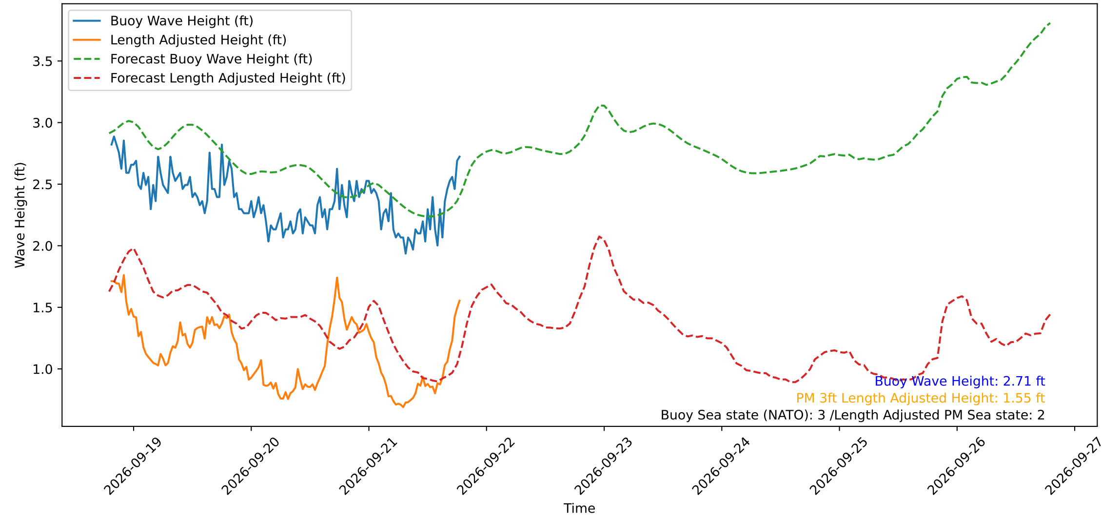
Wave Heights over Time for Red Beach at 2026-09-21 19:10:50
