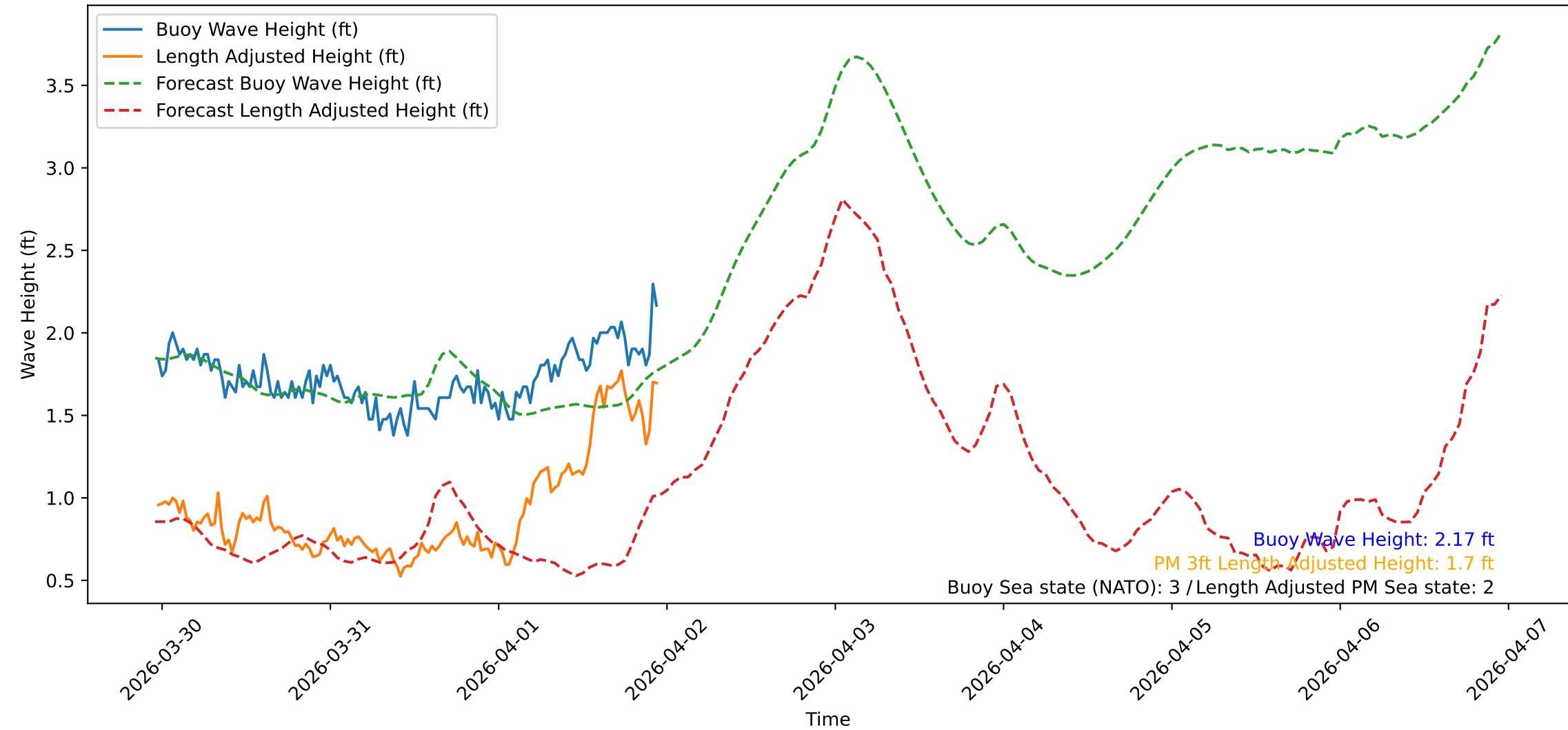
Wave Heights over Time for Red Beach at 2026-04-01 23:10:48
