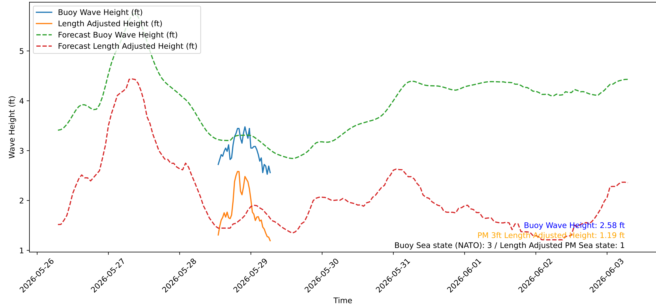
Wave Heights over Time for Oceanside Harbor at 2026-05-29 07:00:21
