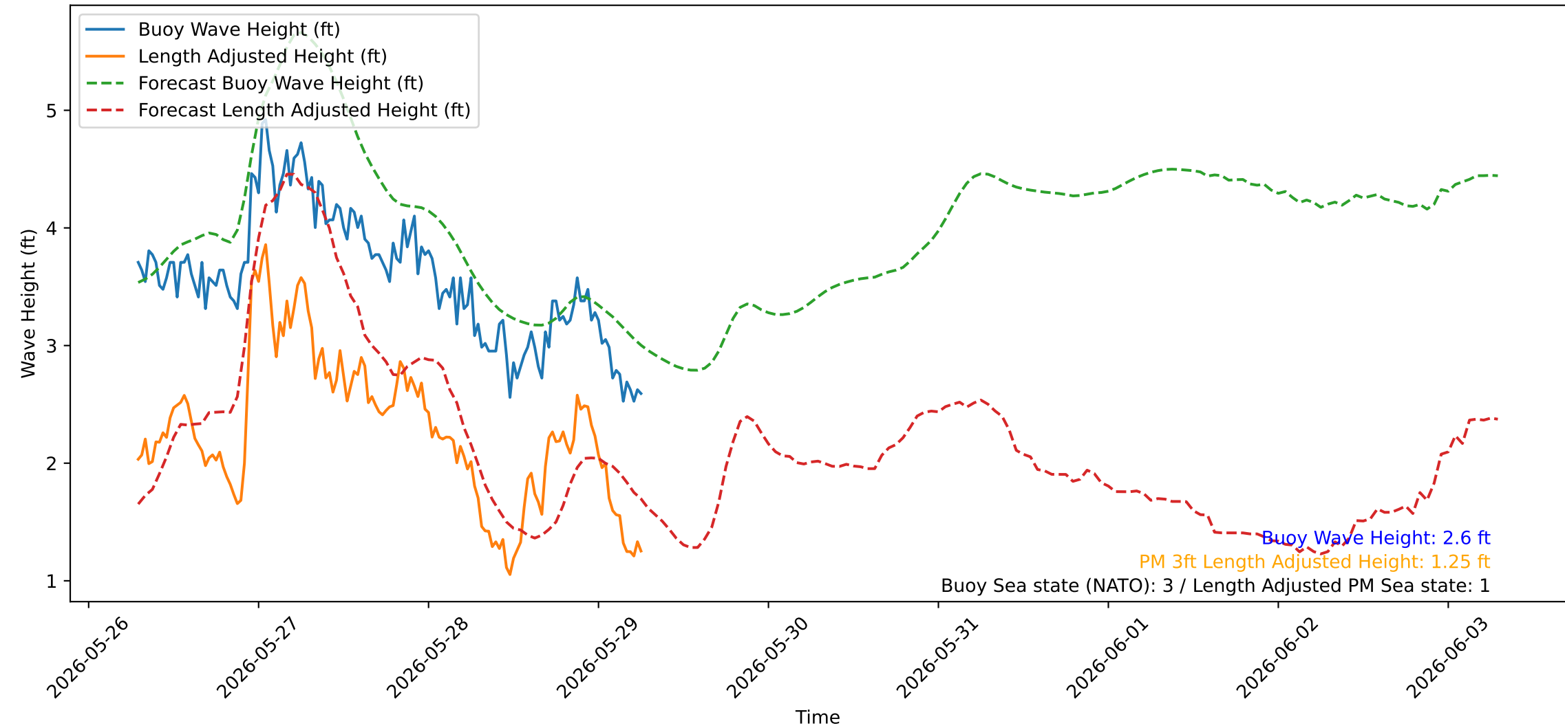
Wave Heights over Time for Green Beach at 2026-05-29 07:01:03
