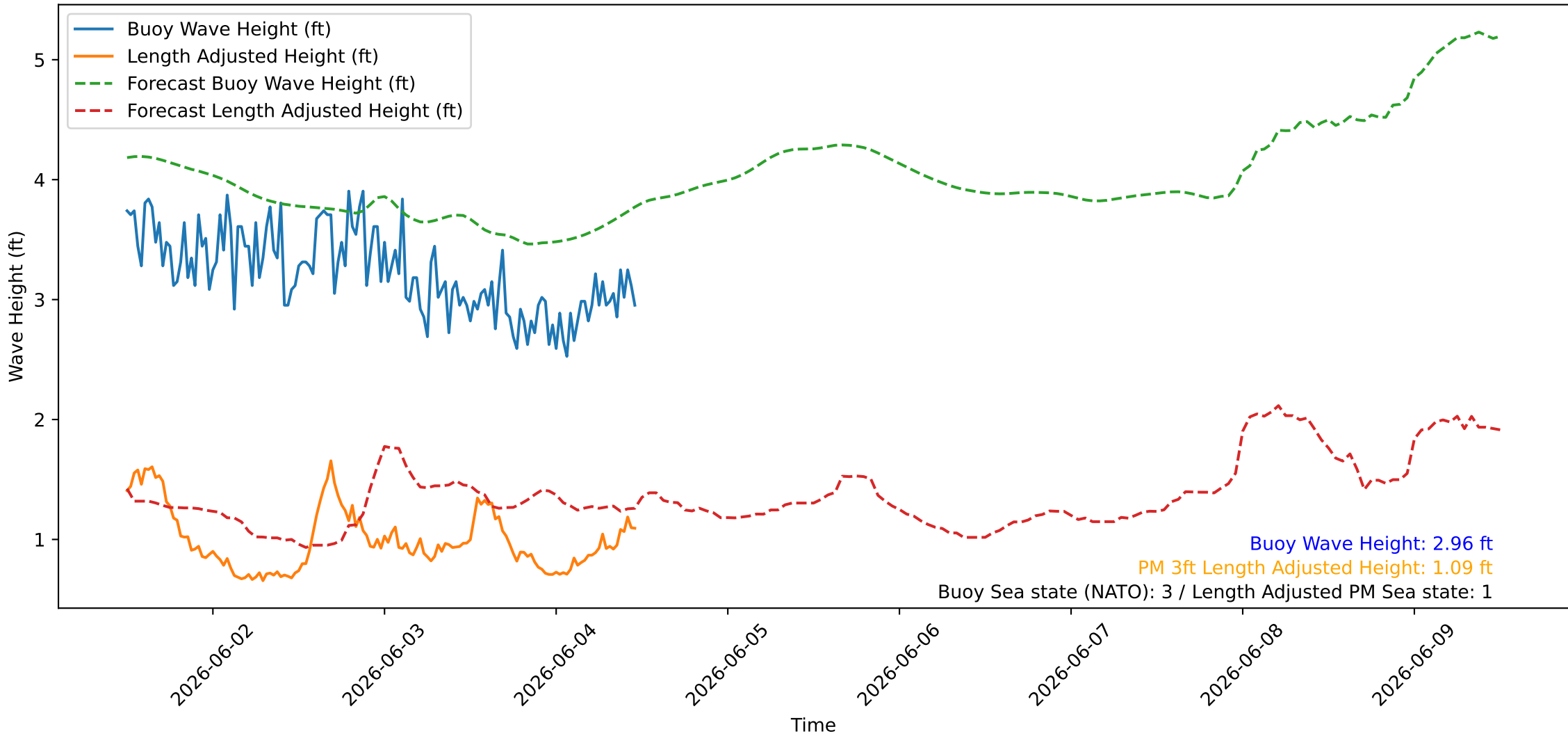
Wave Heights over Time for Red Beach at 2026-06-04 11:40:45
