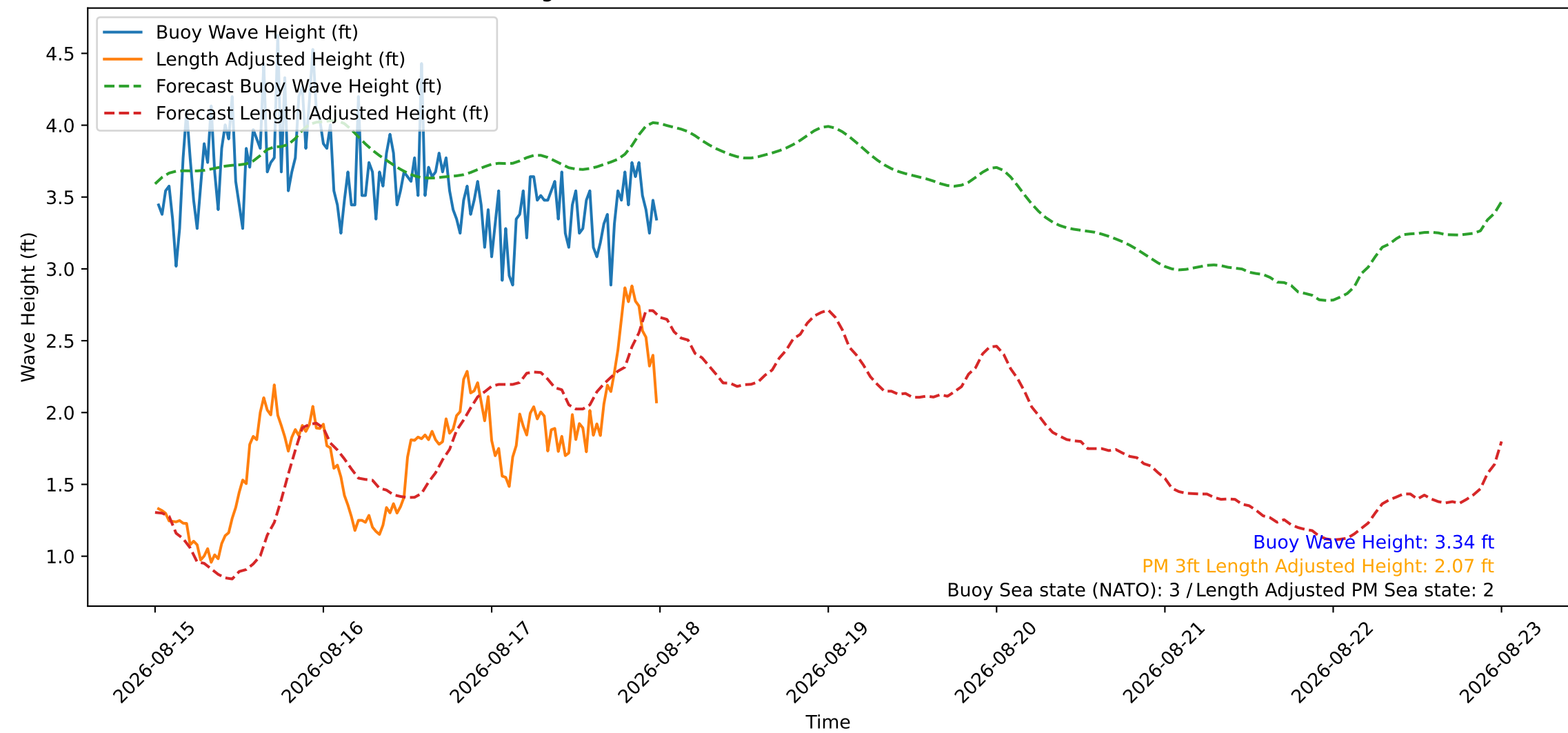
Wave Heights over Time for Oceanside Harbor at 2026-08-18 00:20:26
