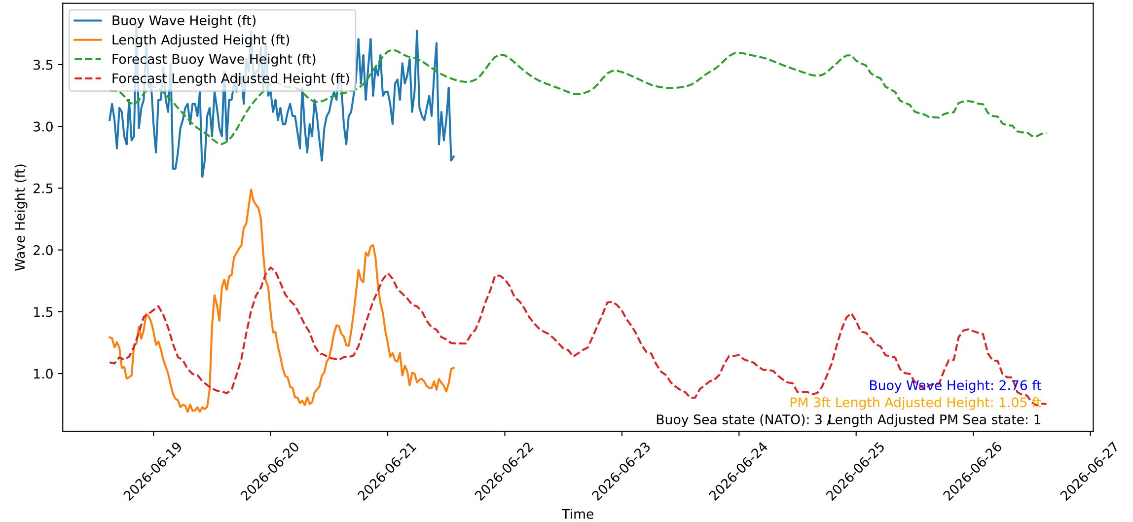
Wave Heights over Time for Red Beach at 2026-06-21 14:30:45
