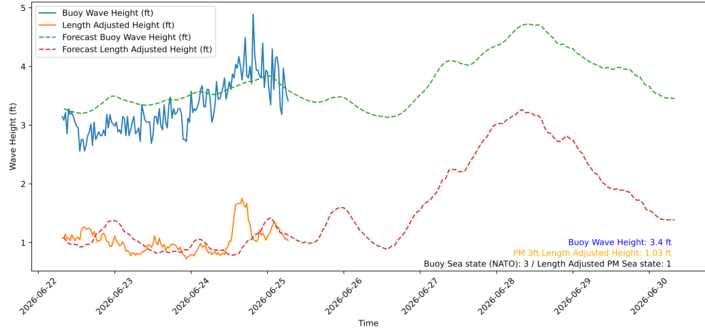
Wave Heights over Time for Oceanside Harbor at 2026-06-25 07:30:26
