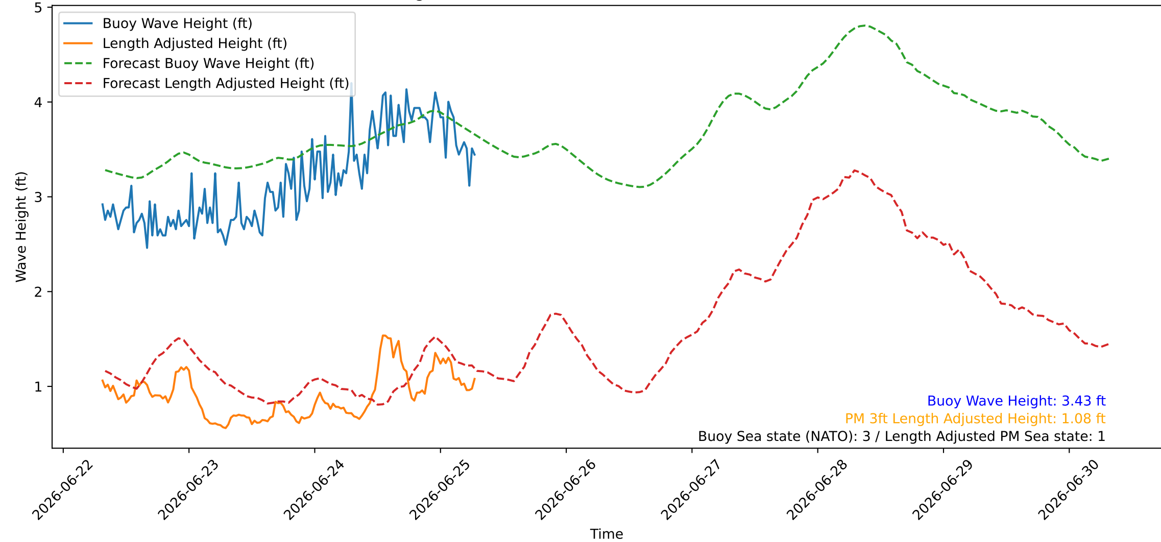
Wave Heights over Time for Green Beach at 2026-06-25 07:31:08
