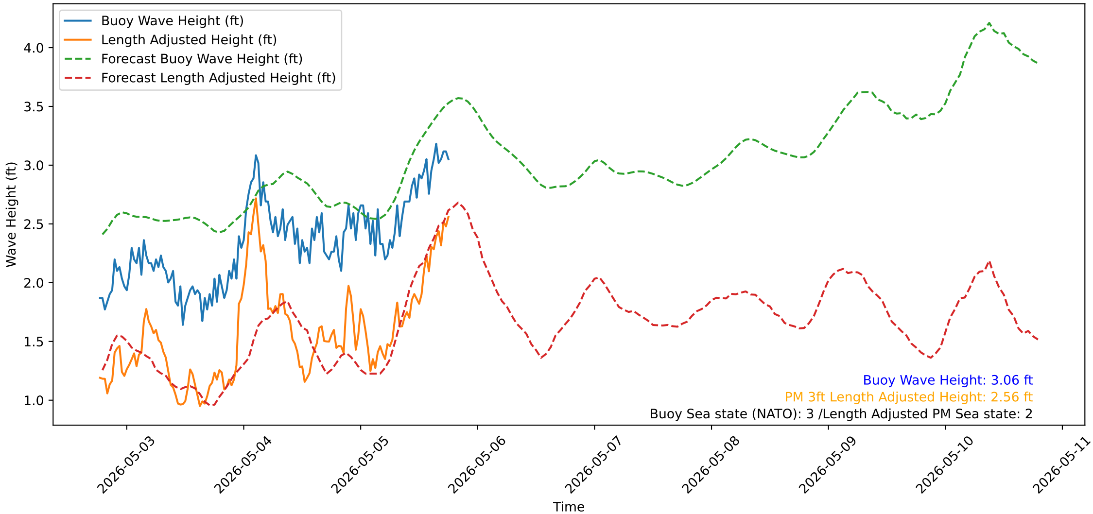
Wave Heights over Time for Oceanside Harbor at 2026-05-05 18:30:32
