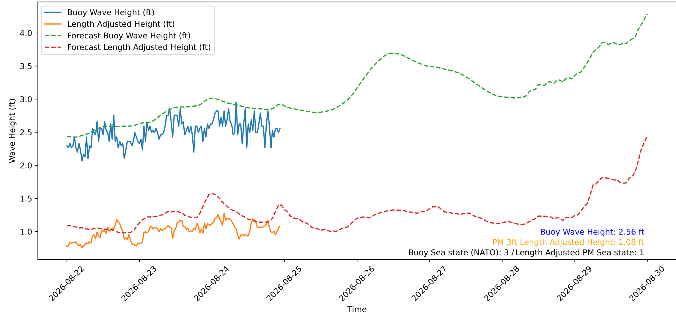
Wave Heights over Time for Red Beach at 2026-08-24 23:30:50
