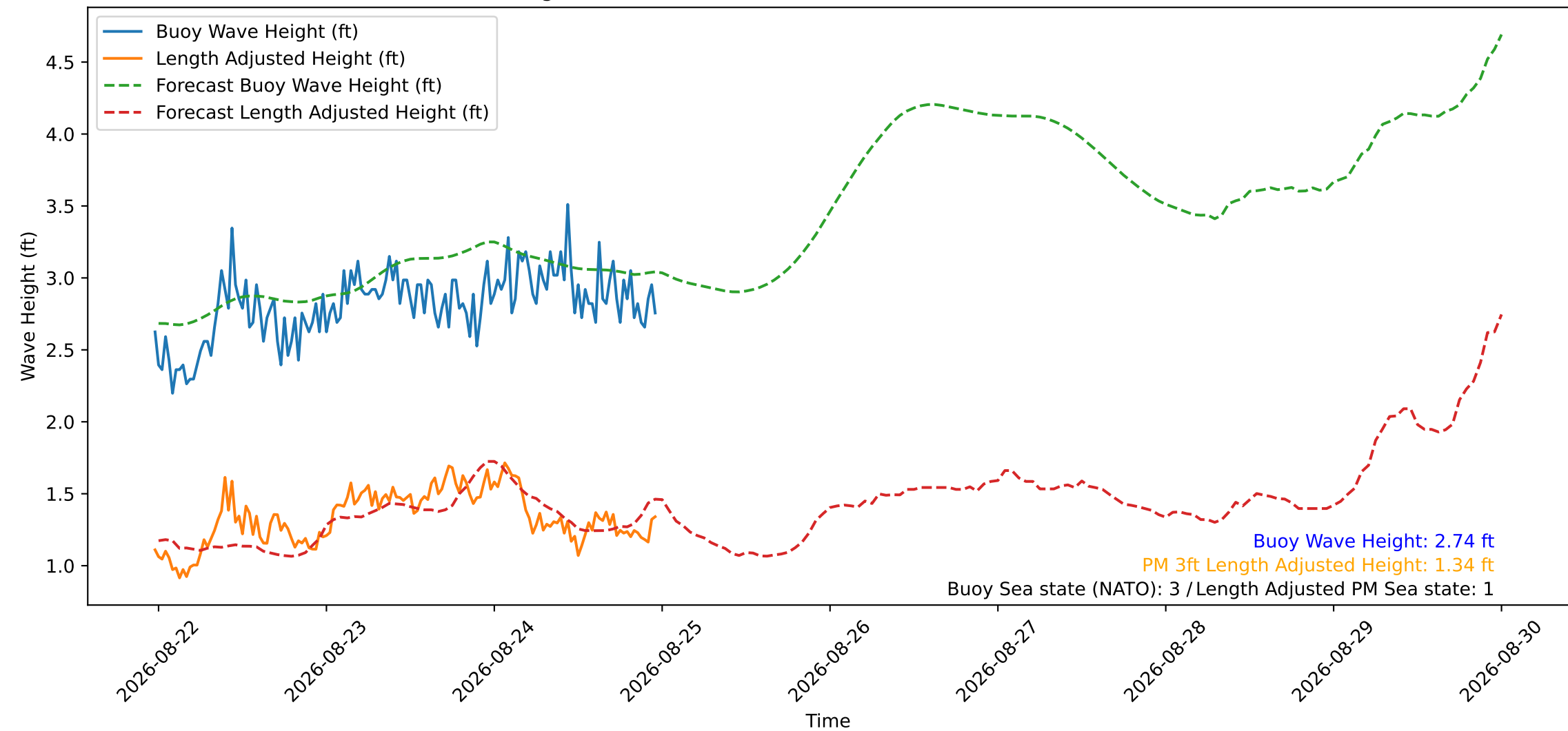
Wave Heights over Time for Oceanside Harbor at 2026-08-24 23:30:30
