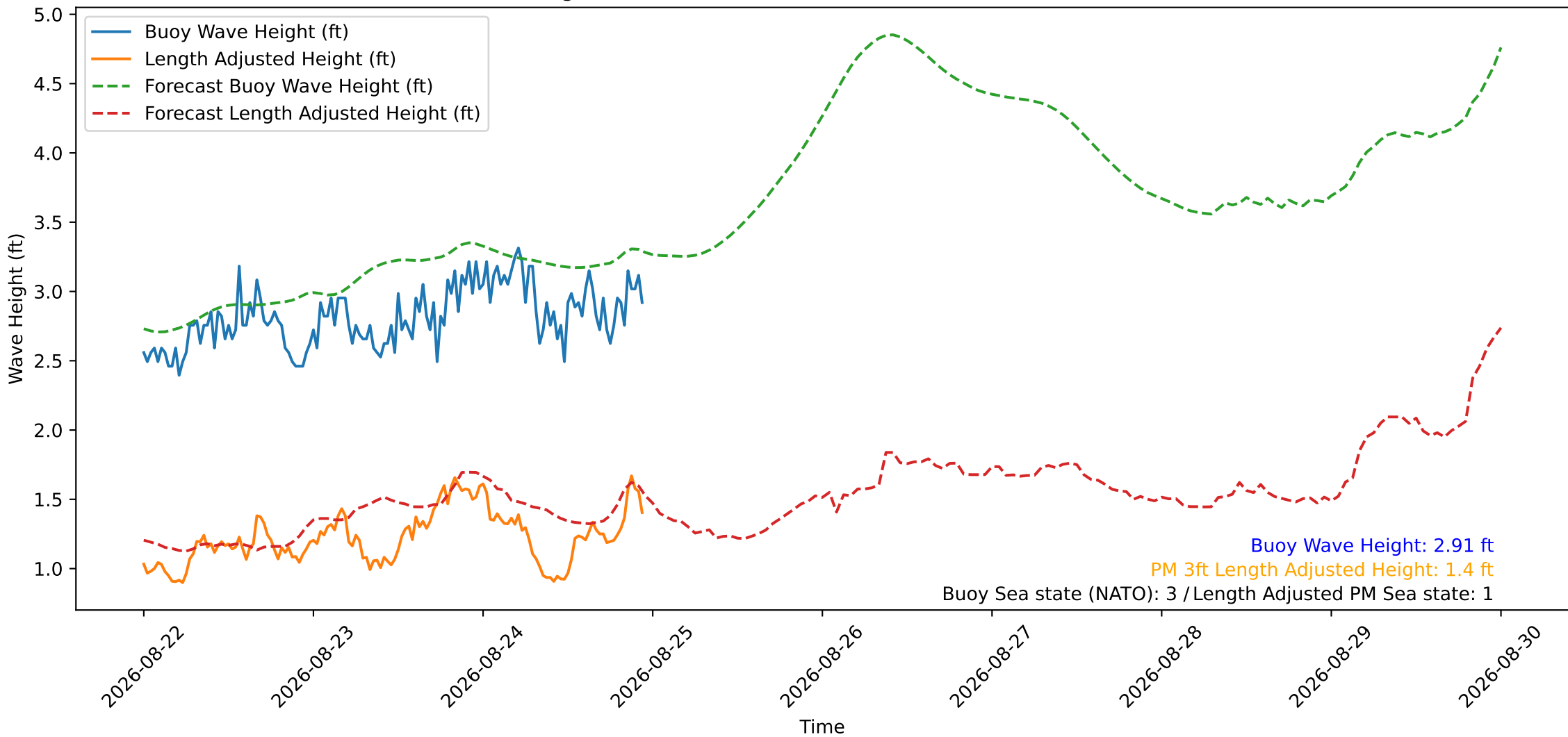
Wave Heights over Time for Green Beach at 2026-08-24 23:31:12
